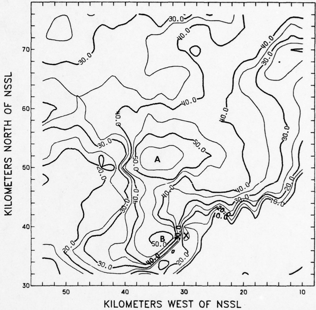
Fig. 38. Pittman's 0-deg reflectivity map for 1810 CST, 23 May 1974. Isoleths of reflectivity in dBZ.
