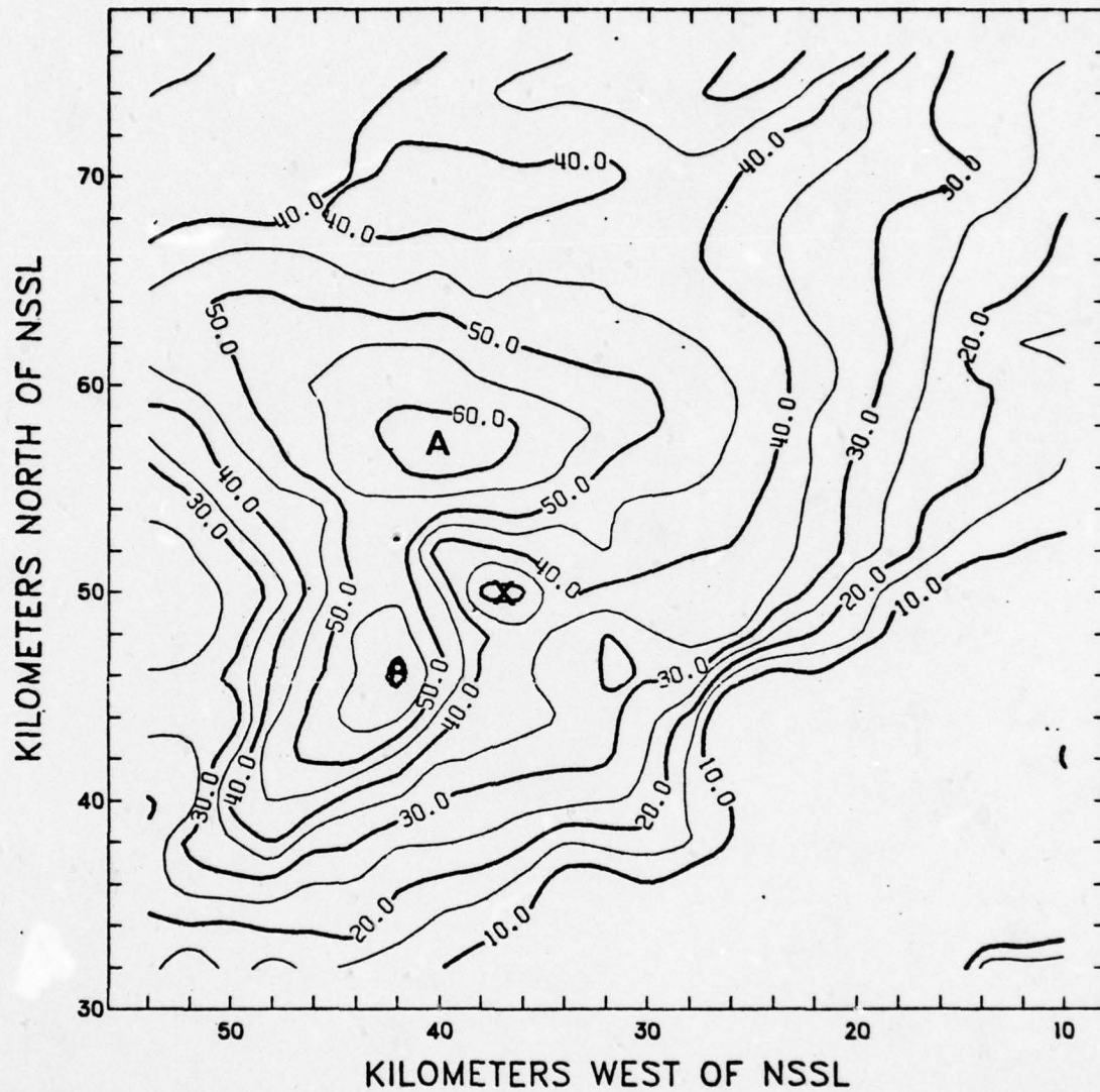
Fig. 41. Lower-layer PVSZ map (LAG-QUAD/LIN) for 1800. CST, 23 May 1974. Isoleths of reflectivity in dBZ.
