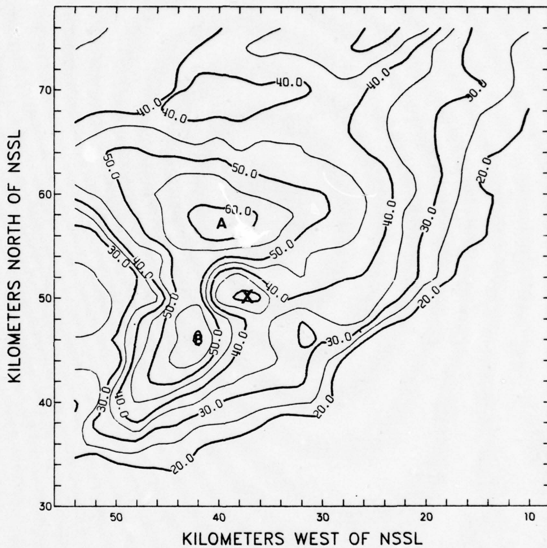
Fig. 20. Lower-layer PVSZ map (LIN-QUAD) for 1800 CST, 23 May 1974. Isoleths of reflectivity in dBZ.
