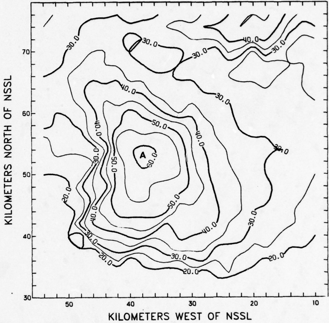
Fig. 30. Pittman's middle-layer PVSZ map for 1800 CST, 23 May 1974. Isoleths of reflectivity in dBZ.
