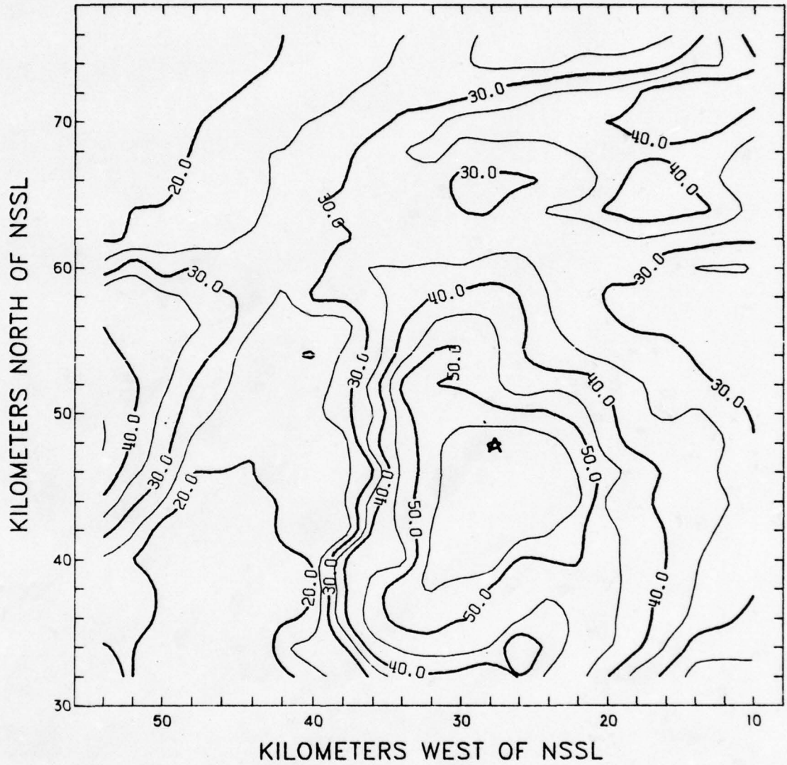
Fig. 33. Middle-layer PVSZ map (LAG-QUAD) for 1810 CST, 23 May 1974. Isopleths of reflectivity in dBZ.
