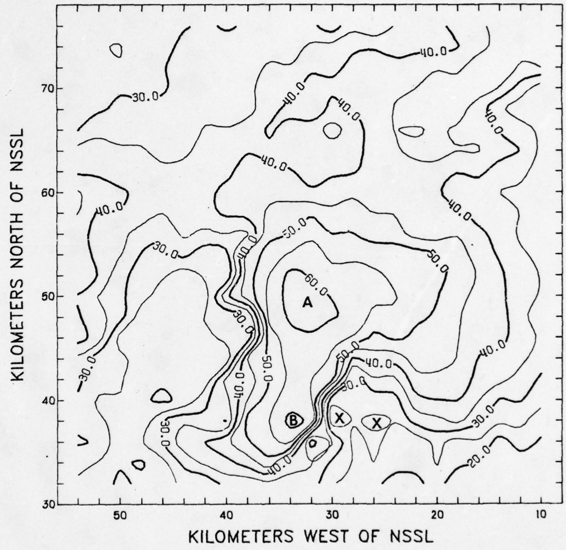
Fig. 35. Pittman's lower-layer PVSZ map for 1810 CST, 23 May 1974. Isopleths of reflectivity in dBZ.
