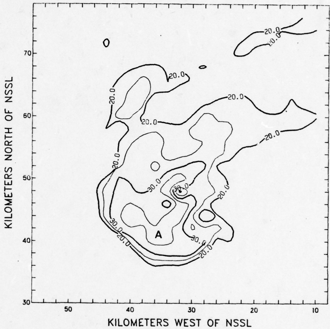
Fig. 19. Upper-layer PVSZ map (LAG-QUAD) for 1800 CST, 23 May 1974. Isopleths of reflectivity in dBZ.
