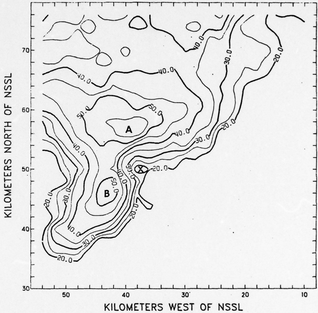
Fig. 47. The 0-deg reflectivity map (QUAD/LIN) for 1800 CST, 23 May 1974. Isoleths of reflectivity in dBZ.
