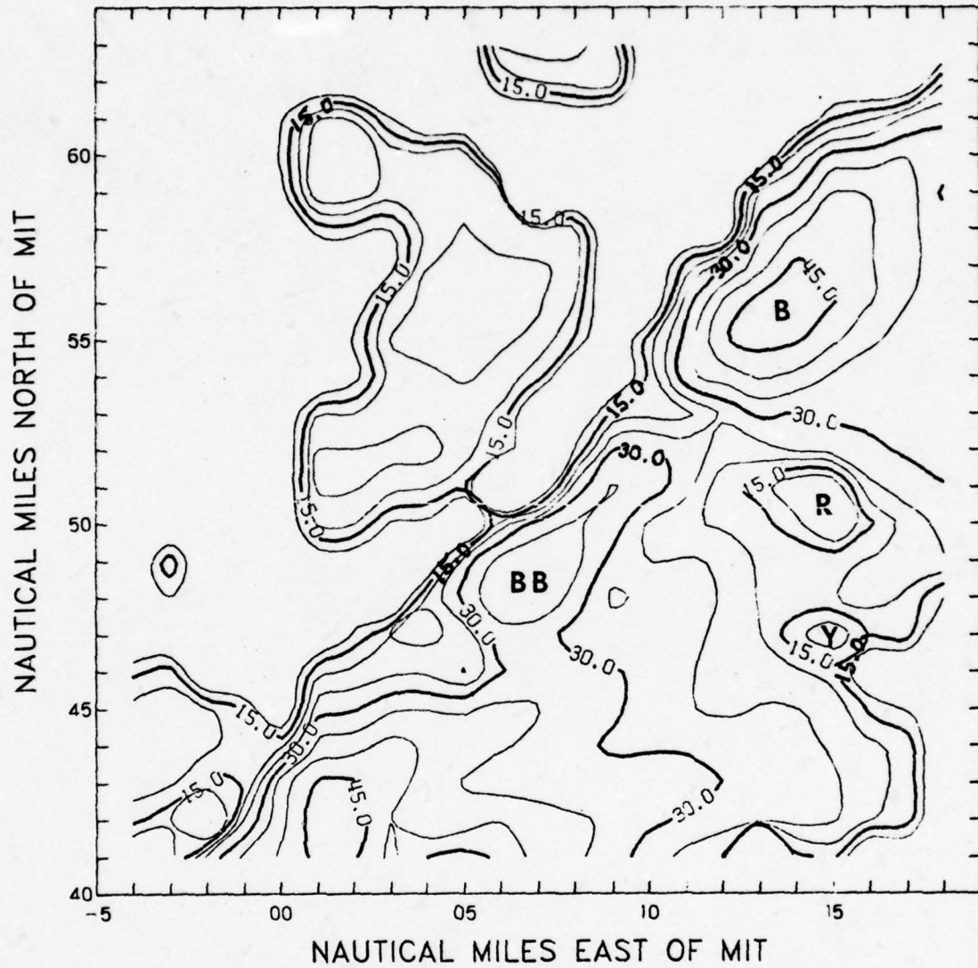
Fig. 74. Lower-layer PVSZ map for 1855 EST, 13 August 1976. Isopleths of reflectivity in dBZ.
