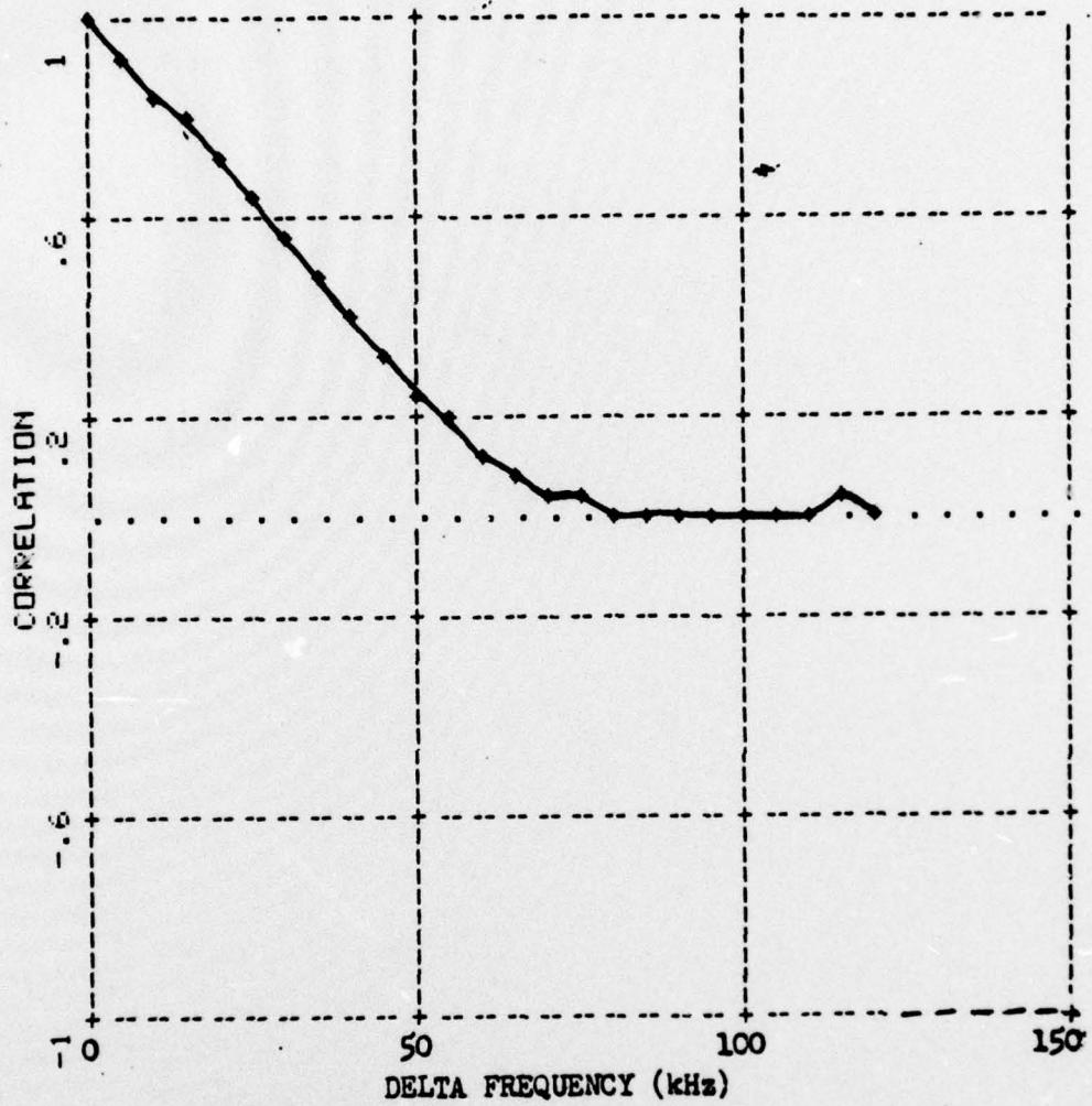
Figure 18. Interfrequency Correlation vs. Delta Frequency
