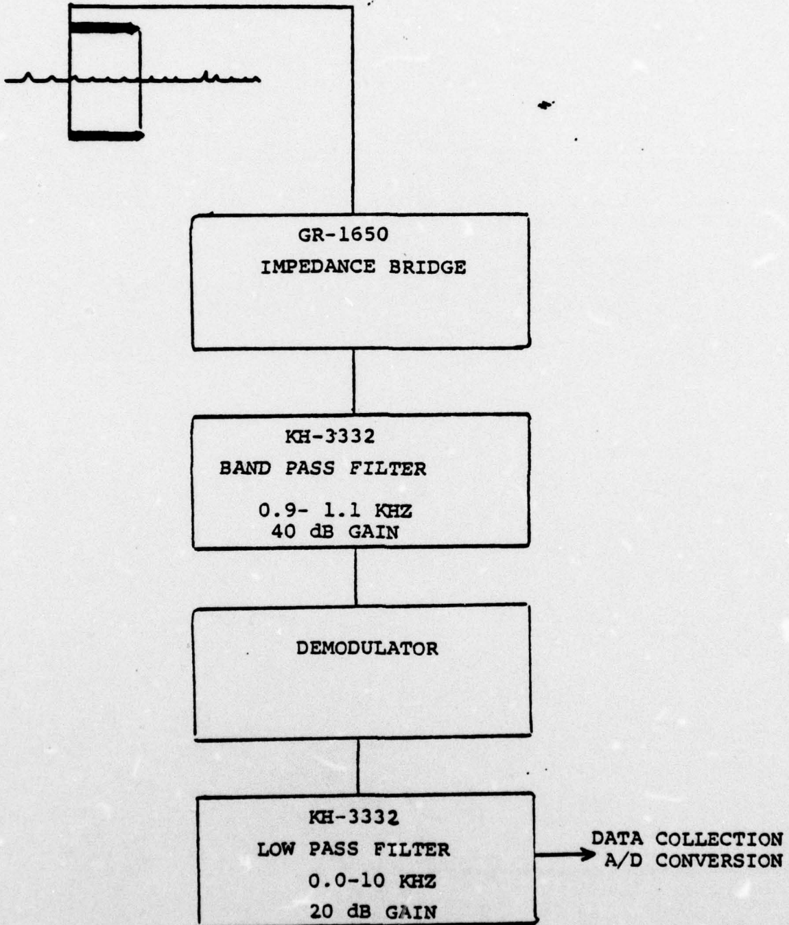
Figure 26. Wave Height Data Collecting Circuit
