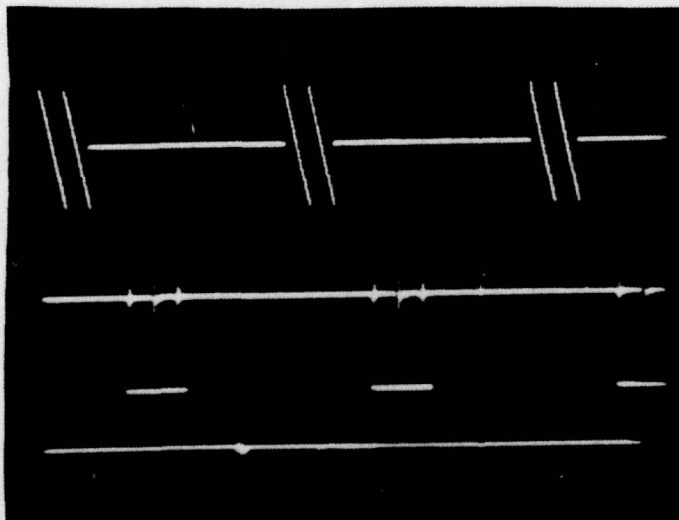
Figure 9. Series of Pulses and Reflections
