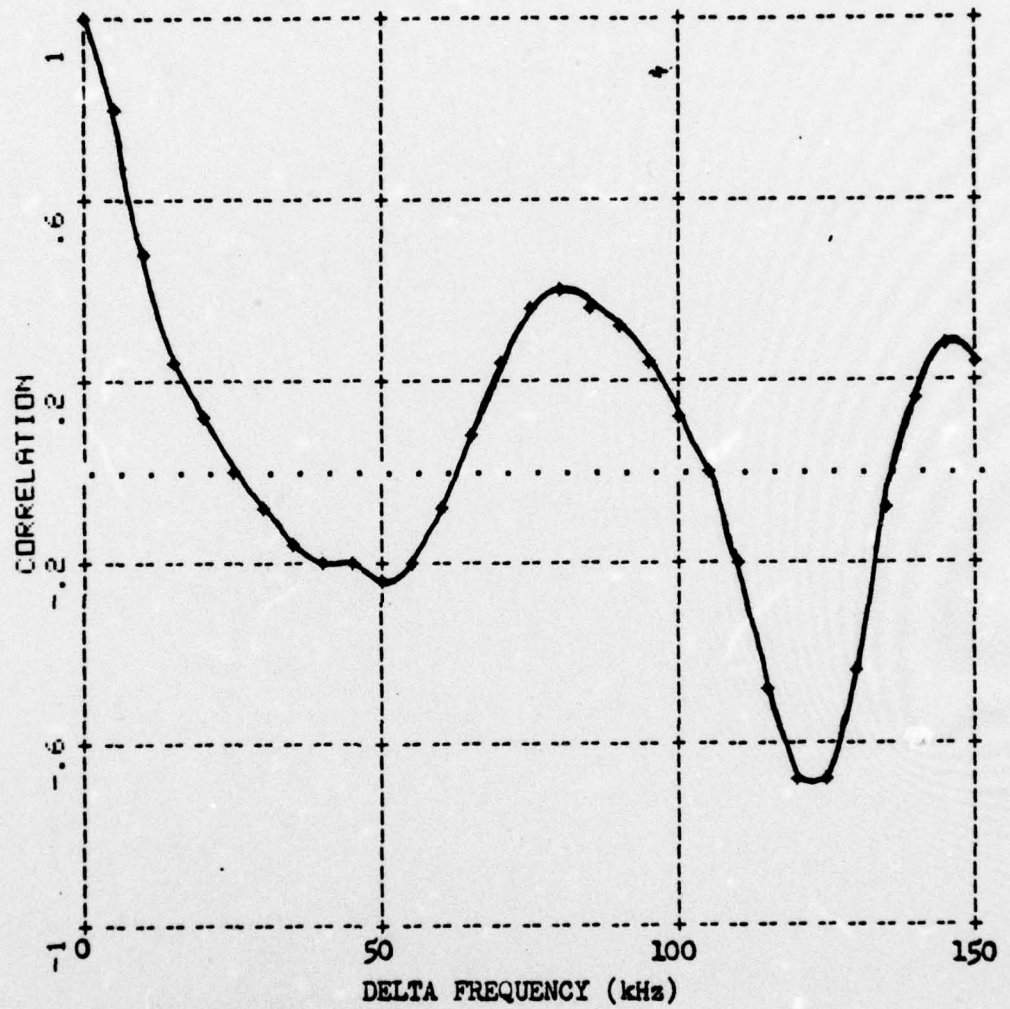
Figure 19. Interfrequency Correlation vs. Delta Frequency
