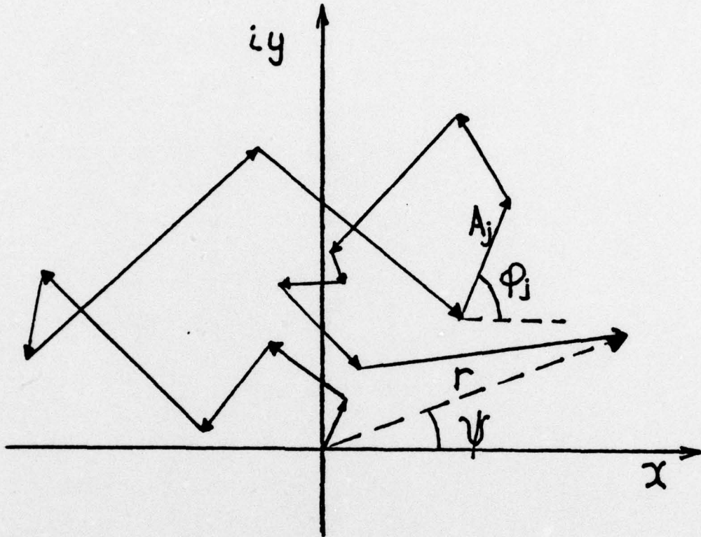
Figure 17a. Instantaneous Received Signal
