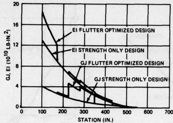
(a) Stiffness Distribution
