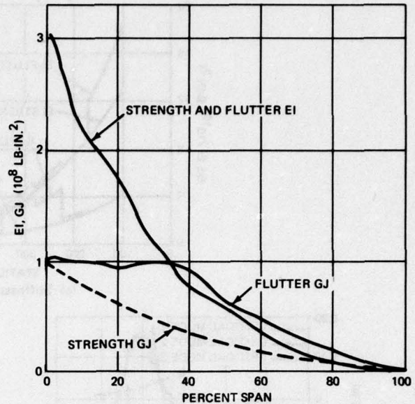
1921-3 FIGURE 3. Vertical Tail Stiffness Distribution
