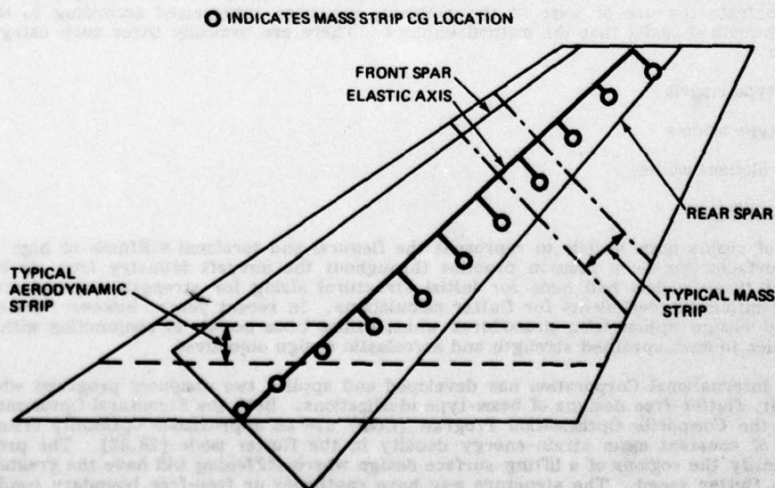
FIGURE 1. Vertical Tail of High-Performance Fighter
