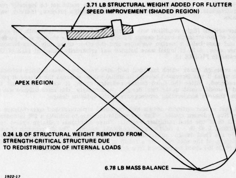
FIGURE 15. Design Changes in All-Movable Stabilizer with Combined Structural and Mass-Balance Design Variables
