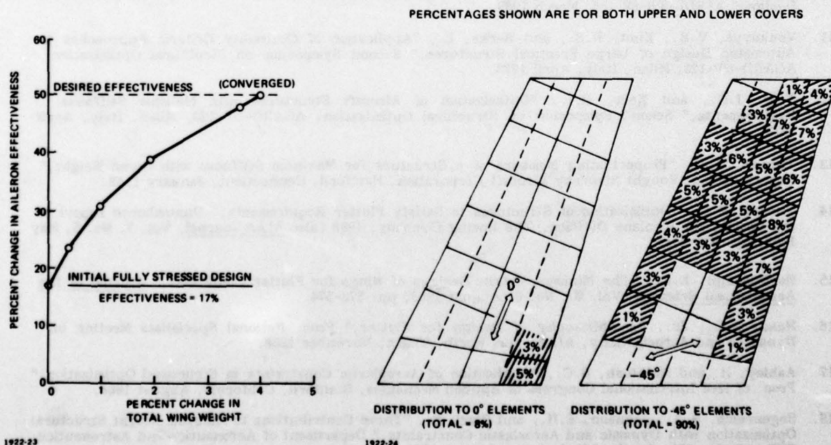
FIGURE 21. Summary of Resizing Steps for Increased Aileron Effectiveness
