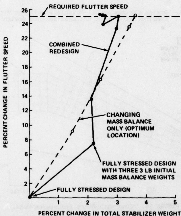
FIGURE 14. All-Movable Stabilizer Redesign by FASTOP
