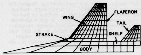
FIGURE 6. Aerodynamic Simulation of Fighter
