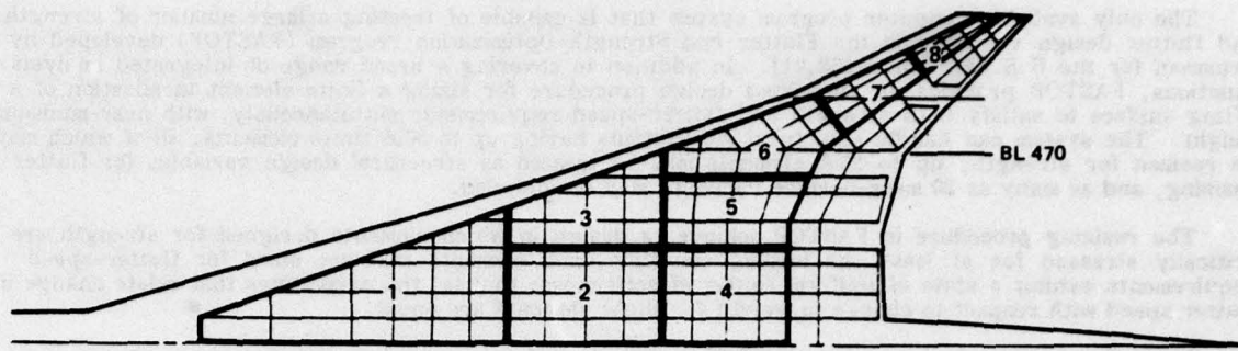
FIGURE 11. Design Regions for Flutter Optimization, Arrow Wing, Phase I
