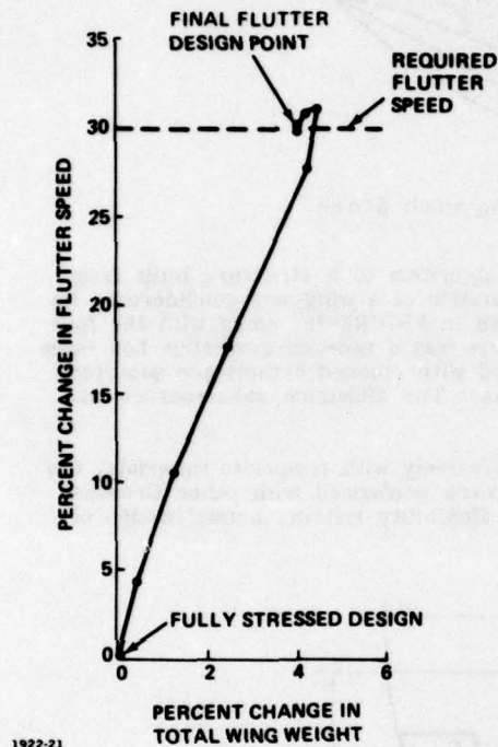
FIGURE 19. Composite-Wing Redesign by FASTOP
