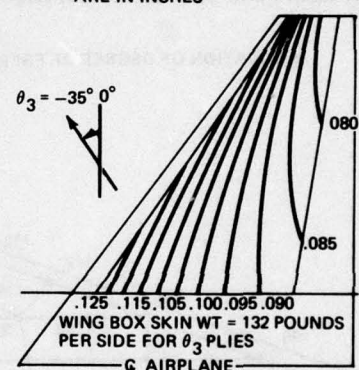
(c) Distribution for \theta = -35^\circ Plies
