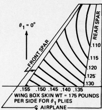
(a) Distribution for \theta = 0^\circ Plies
