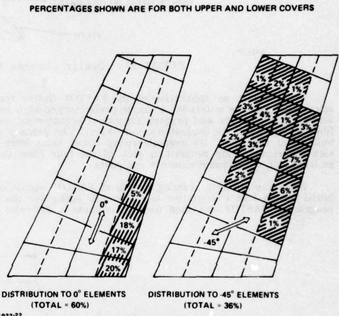
FIGURE 20. Distribution of Total Weight Increment Added to Composite Cover Skins for Increased Flutter Speed
