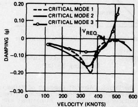
(c) Optimized Case - Strength Plus Flutter Constraints
