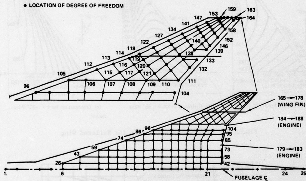
FIGURE 10. Structural Grid Point Network for Arrow-Wing Study
