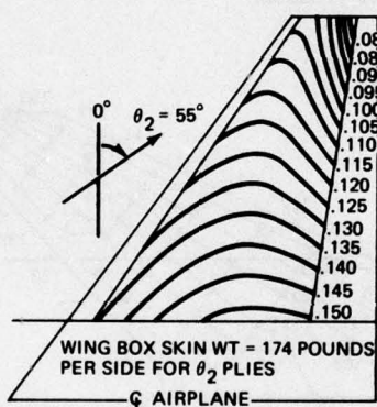
(b) Distribution for \theta = 55^\circ Plies
