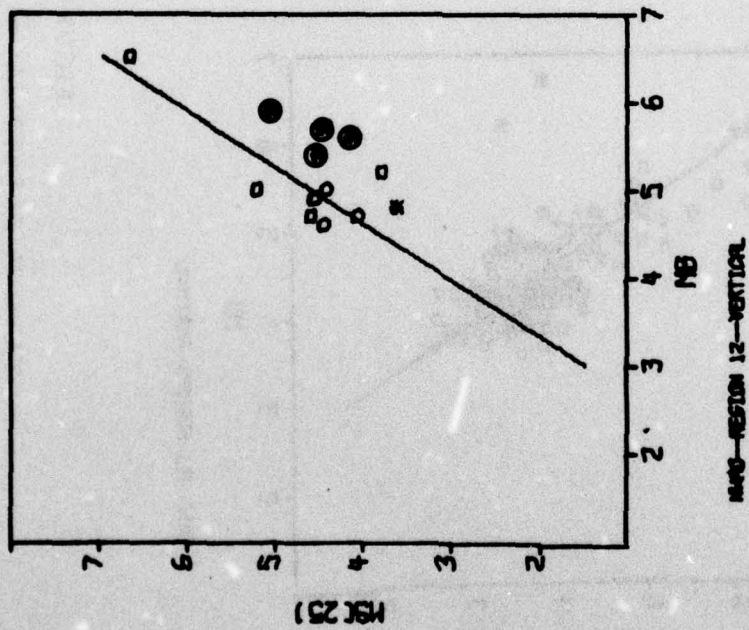
FIGURE VI-36 NAWO 25-SECOND M_s - m_b DATA FOR REGION 12
