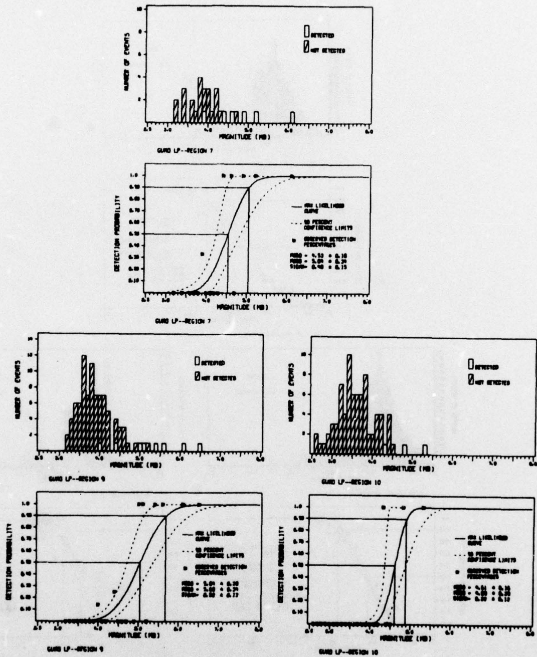
FIGURE V-14 GUM0 LONG-PERIOD DETECTION STATISTICS REGIONS 7, 9, AND 10
