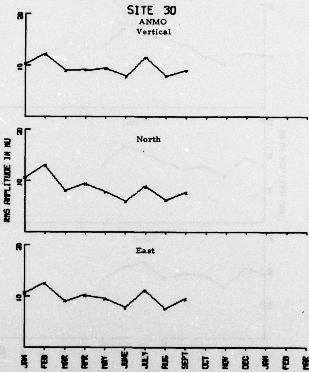
FIGURE IV-13 ANMO LONG-PERIOD RMS NOISE TRENDS
