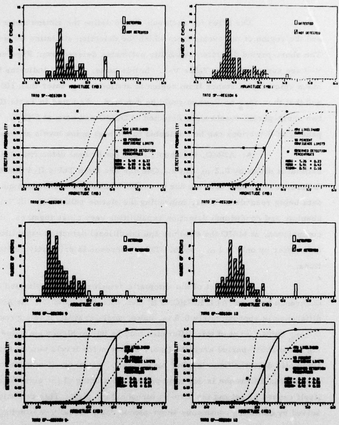
FIGURE V-8 TATO SHORT-PERIOD DETECTION STATISTICS REGIONS 5, 6, 9, 12
