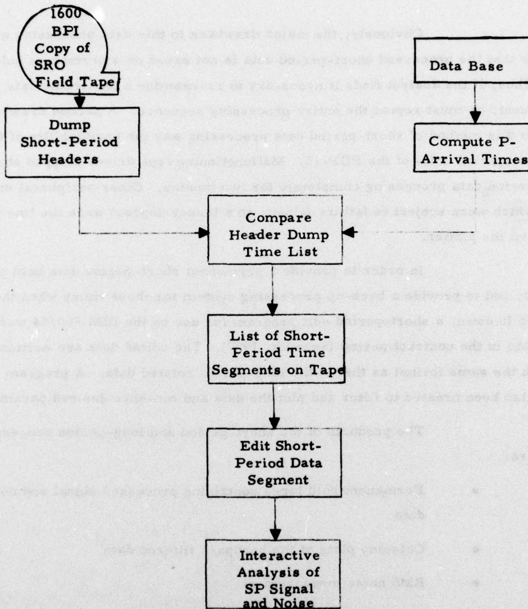
FIGURE II-5 SHORT-PERIOD DATA PROCESSING FLOW CHART (PDF-15 DATA PROCESSING)
