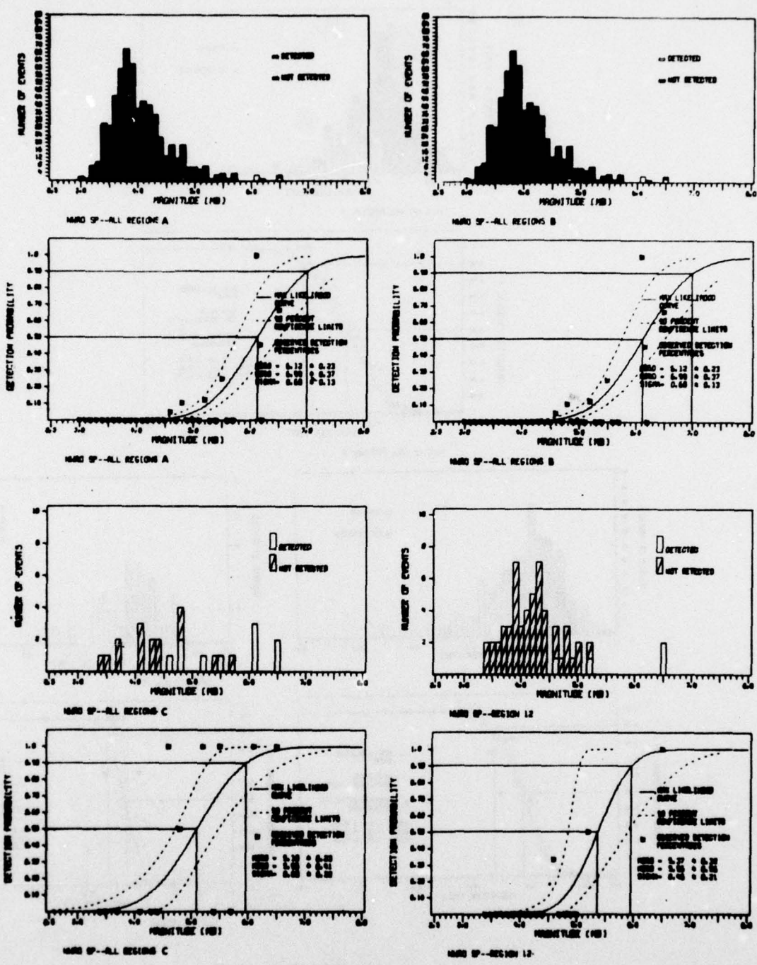
FIGURE V-6 NWAO SHORT-PERIOD DETECTION STATISTICS ALL REGIONS A, B, C AND REGION 12
