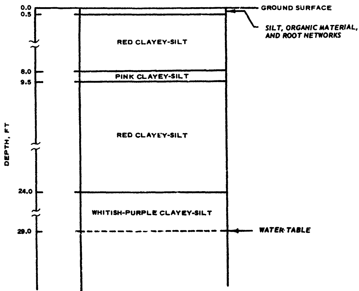
Figure 2.1 Site geology.
