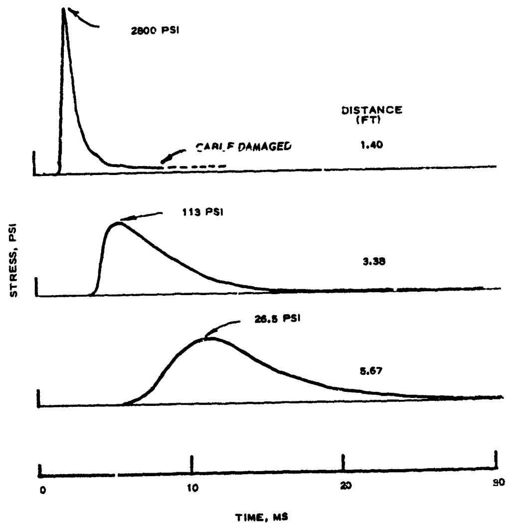
Figure A.7 Stress waveforms, Event 5 (DOB = 1.26 feet).
