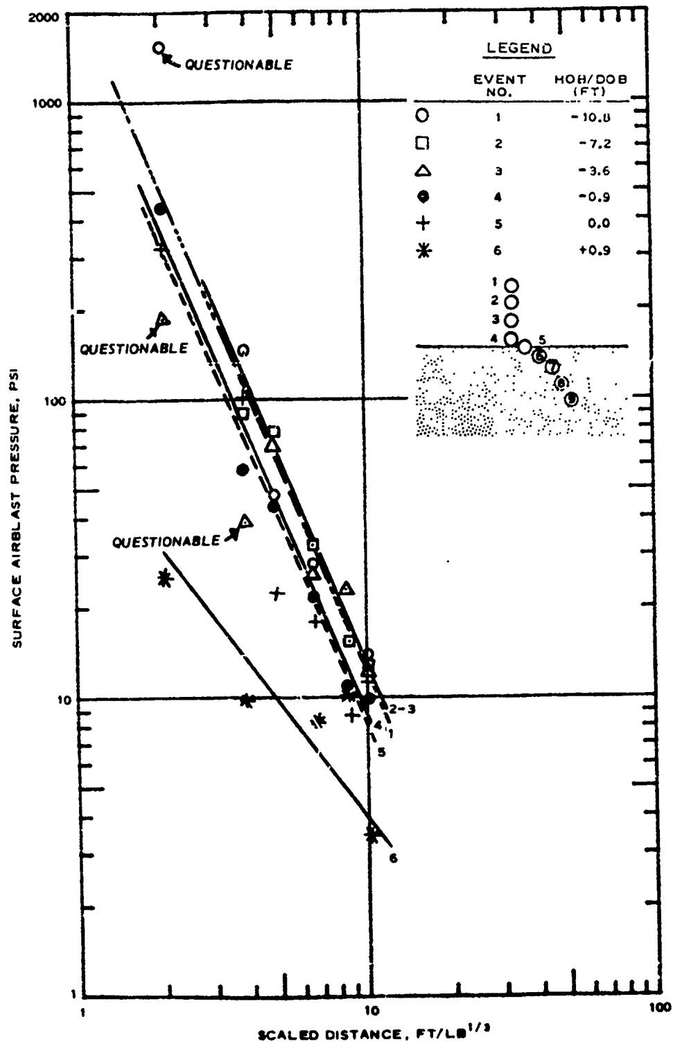
Figure 3.33 Peak surface airblast pressure versus scaled distance.
