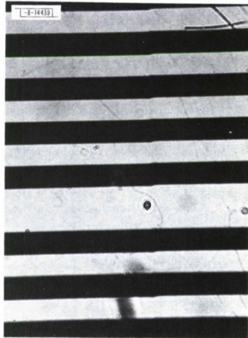
Fig. IV-5. Detail of double-width space on 10X "center" reticle. After a 10X reduction on a chromium-plated plate, linewidths are 6.35 \mu\text{m} , with equal size spaces between lines, except double-width space in center. Line discontinuity at butting of photocomposed images is about 0.6 \mu\text{m} . Because of relative size of features, no degradation in line edge acuity can be seen on lines adjacent to double space. Apparent defects seen in this figure are due to dust in inspecting microscope optics.
