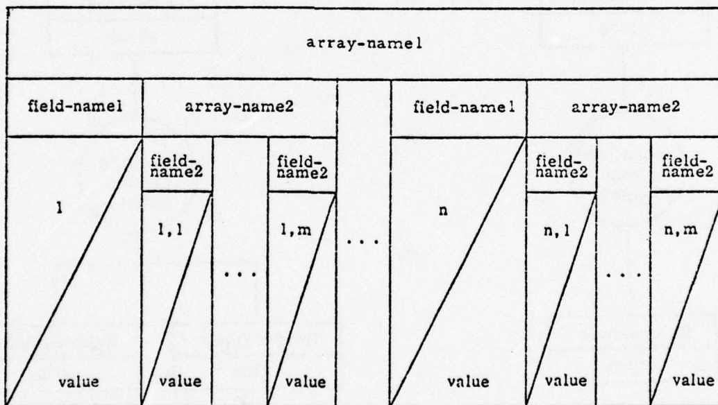
Figure 3. Logical Structure of an Array (two array levels are shown).
