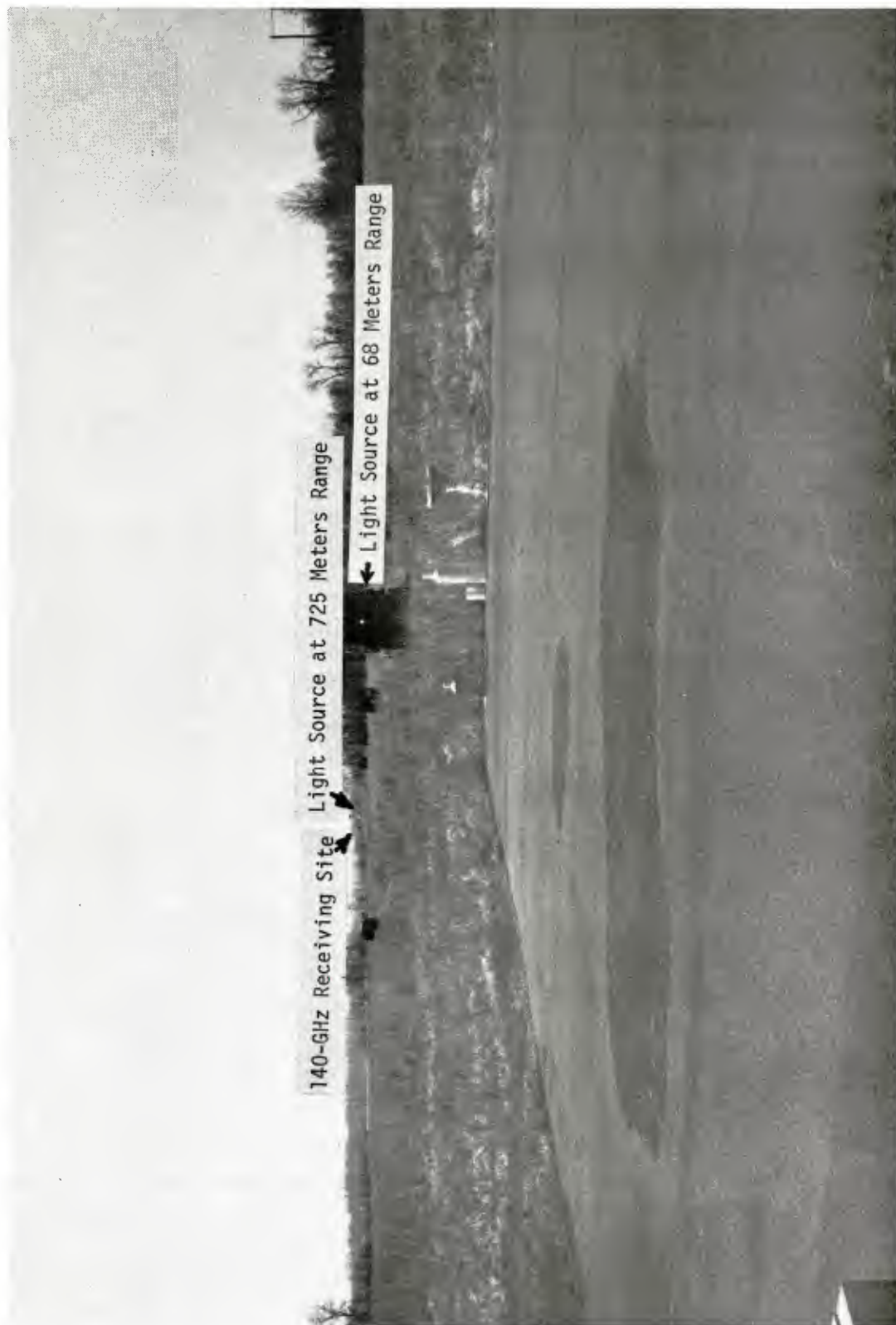
Figure 1. Field Site for 140 GHz Attenuation and Visibility Measurements
