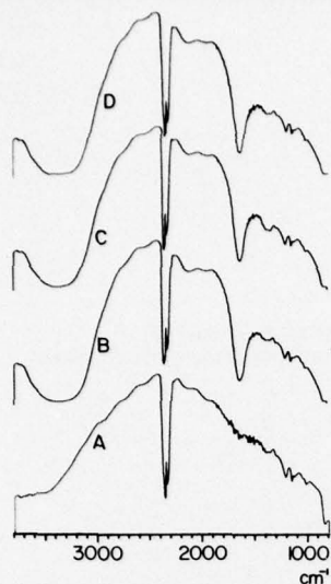
Figure 1. Single-beam spectra
