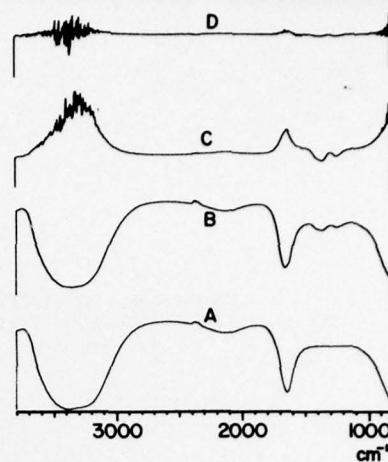
Figure 2. Ratioed spectra
