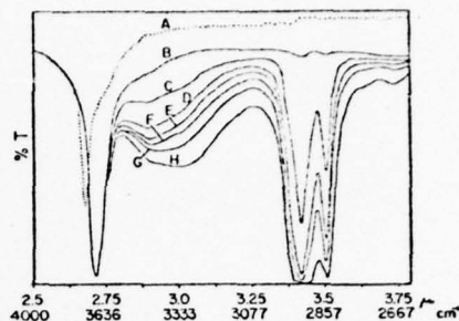
FIG. 1. Octadecanol adsorption. After the spectrum A of the degassed sample in vacuo was recorded, the sample was immersed in \text{CCl}_4 (B). A 0.5 \text{mM} octadecanol solution was then introduced and circulated, and spectra were recorded after 0.5 hr (C), 12 hr (D), and 36 hr (E). A 1 \text{mM} octadecanol solution was then introduced and circulated, spectrum F being recorded after 3.5 hr and spectrum G after 20 hr. Spectrum H was recorded 3.5 hr after a 5 \text{mM} solution had been introduced.
