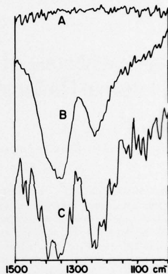
Figure 3. Scale-expanded spectra
