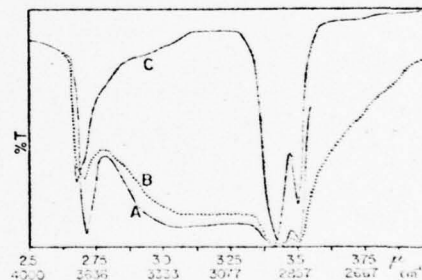
FIG. 3. Octadecylamine desorption. After spectrum O of Fig. 2 has been recorded, the solution was replaced by \text{CCl}_4 and after 24 hr, spectrum A was recorded. The \text{CCl}_4 was removed, the system degassed for 14 hr at 25^\circ\text{C} and spectrum B was recorded. Then, after degassing at 200^\circ\text{C} for 4 hr, spectrum C was recorded.
