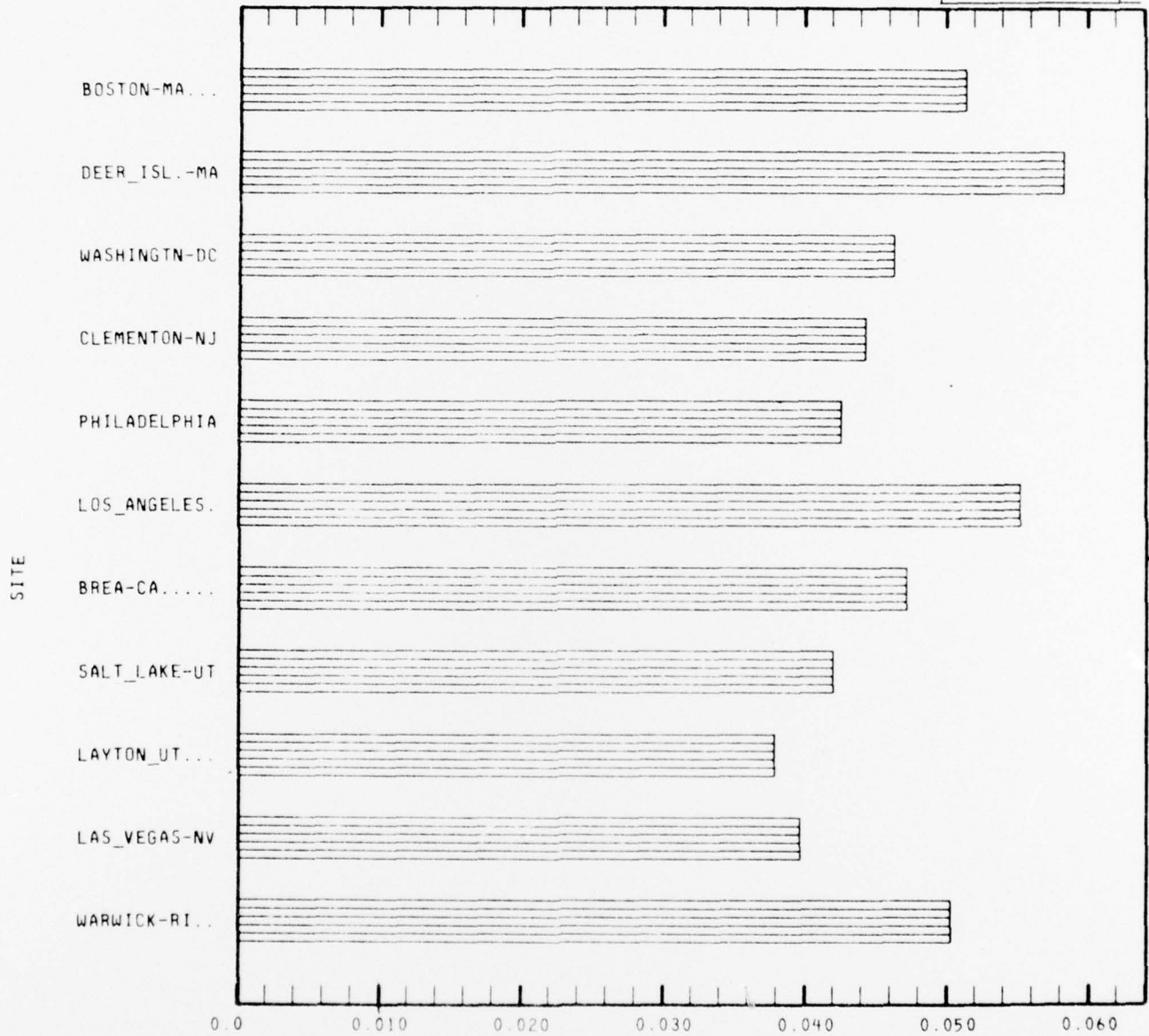
Fig. IV-12. Azimuth error (standard deviation in degrees).
