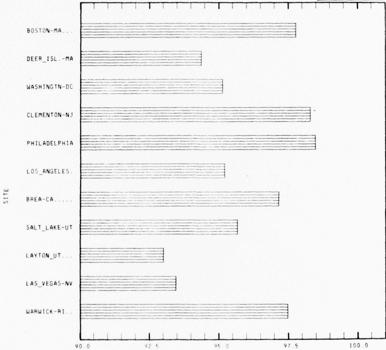
Fig. IV-3. Blip/scan ratio (crossing tracks; percent).
