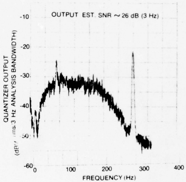
Figure 21. SNR Measurement: Signal in Transitional Region, Lowpass Filter Set at 200 Hz, Signal at 275 Hz; Reference Test Configuration 1
