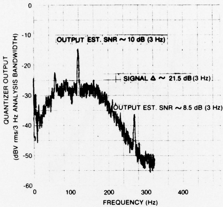
A. Passband Signal at -5 dBV rms, Transitional Signal at -20 dBV rms, Noise Signal at -3 dBV rms
