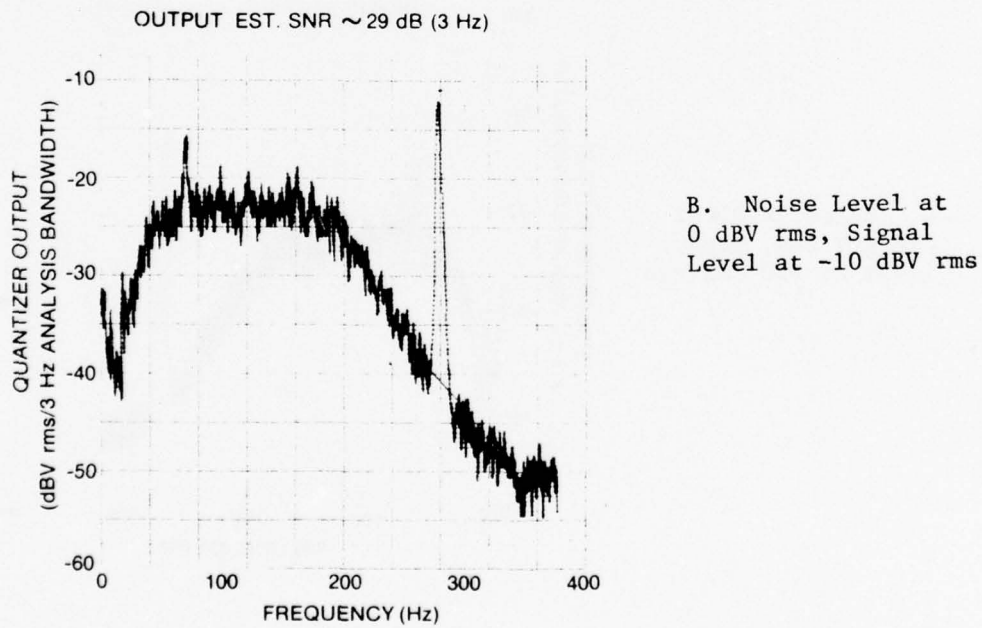
Figure 20. SNR Measurement: Signal in Transitional Region, Lowpass Filter Set at 200 Hz, Signal at 275 Hz; Reference Test Configuration 1
