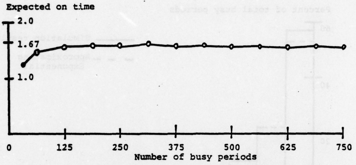
a. Expected on time for a switched busy period. Value calculated using approximations=1.67.
