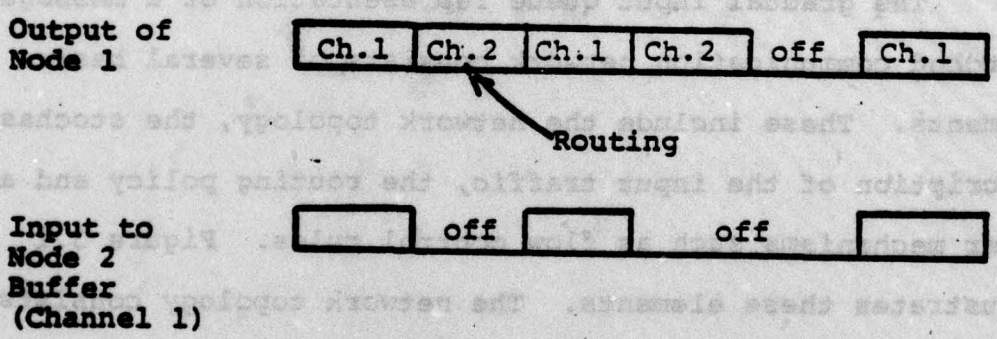
b. Typical Switched traffic sequence.
