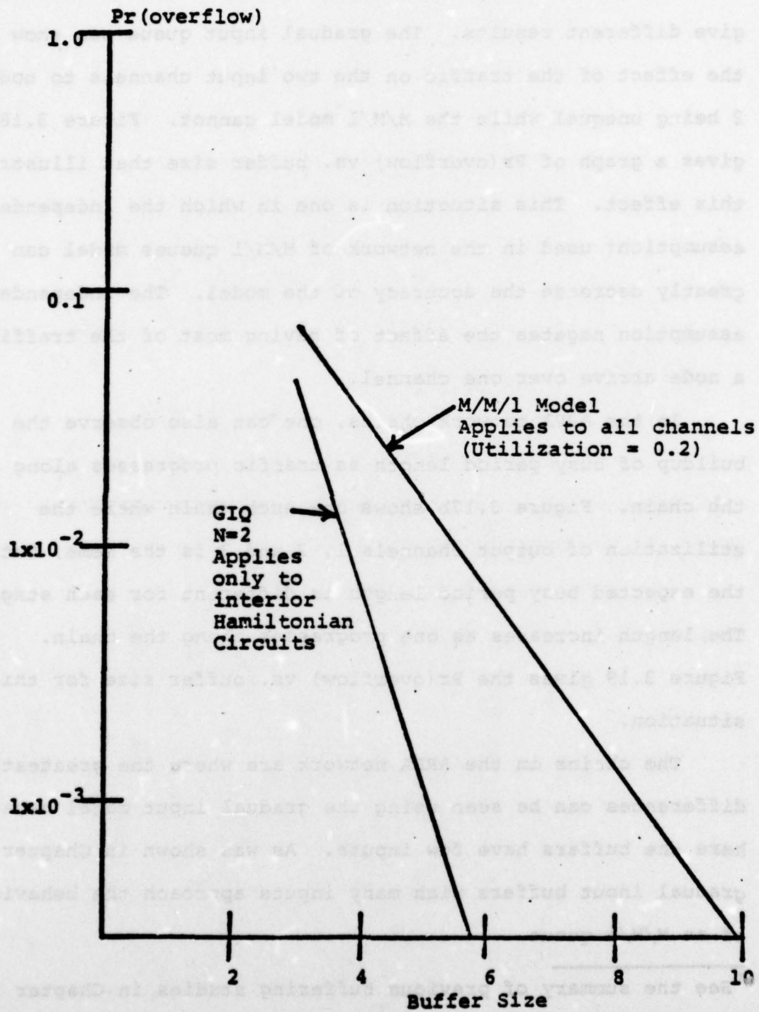
FIGURE 3.16 - Pr(overflow) for the seven node network.
