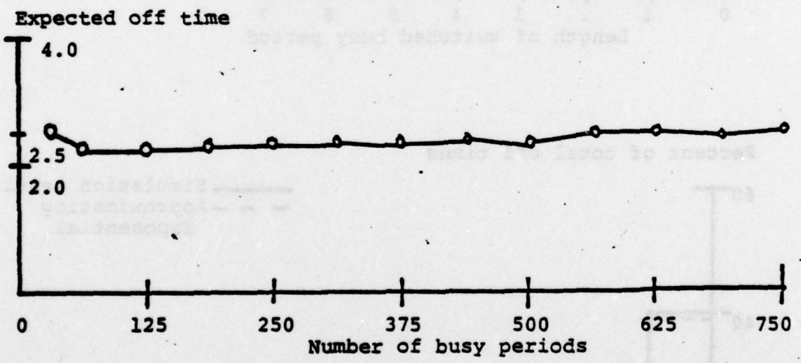
b. Expected off time for a switched traffic stream. Value calculated using approximations=2.50.
