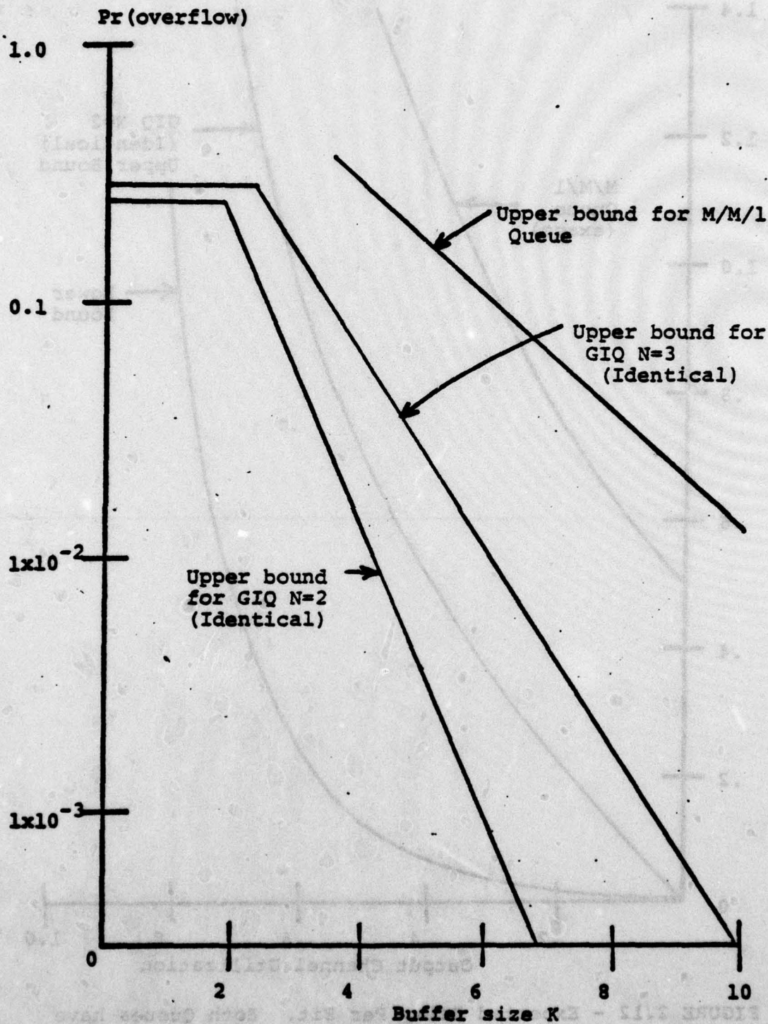
FIGURE 2.11 - Bounds on Pr(overflow). Mean on time for input channels=1. Queue utilization=0.5.
