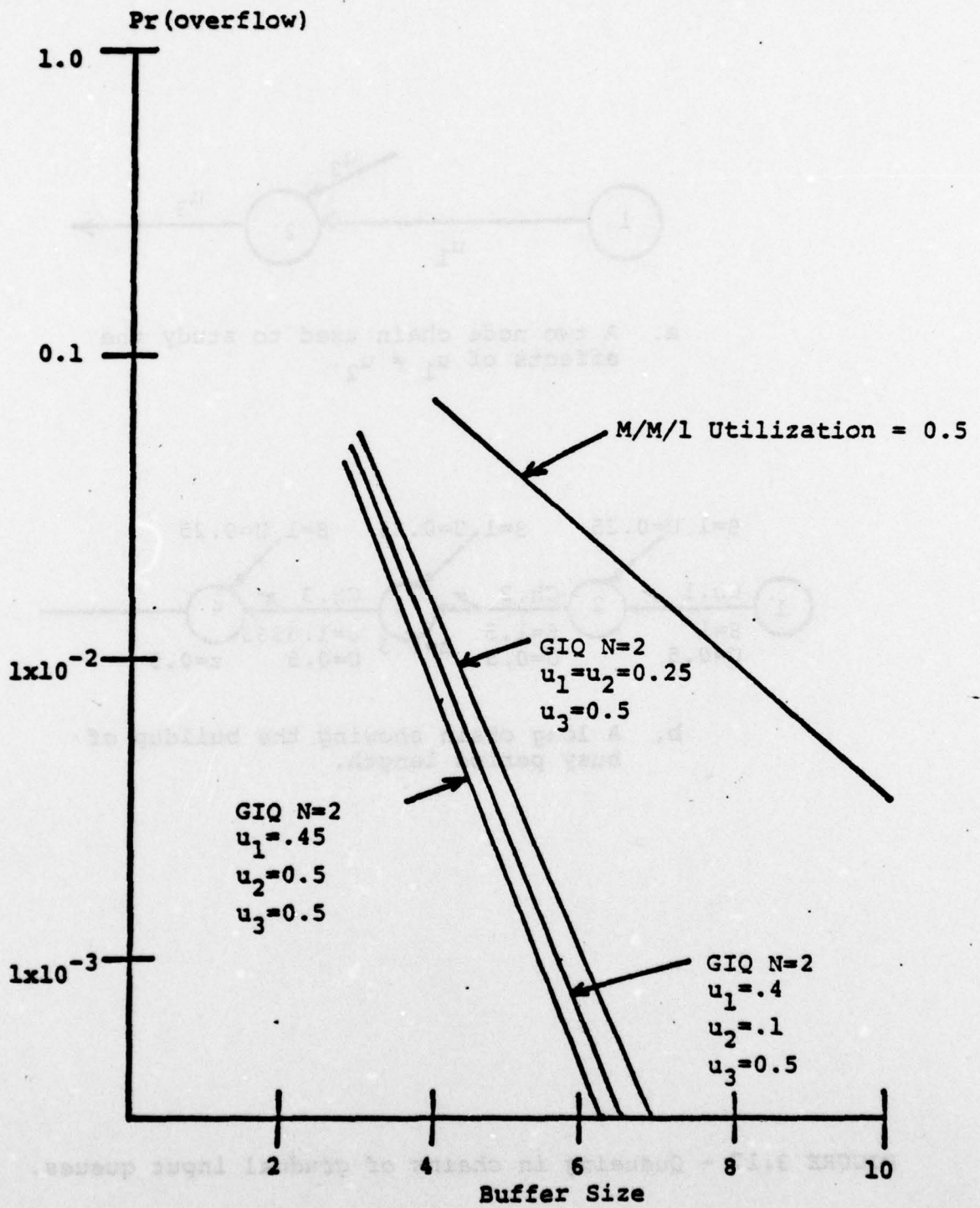
FIGURE 3.18 - Pr(\text{overflow}) for Figure 3.17a.
