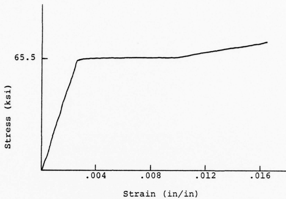
Fig. 5. Steel Stress-Strain Curve.
