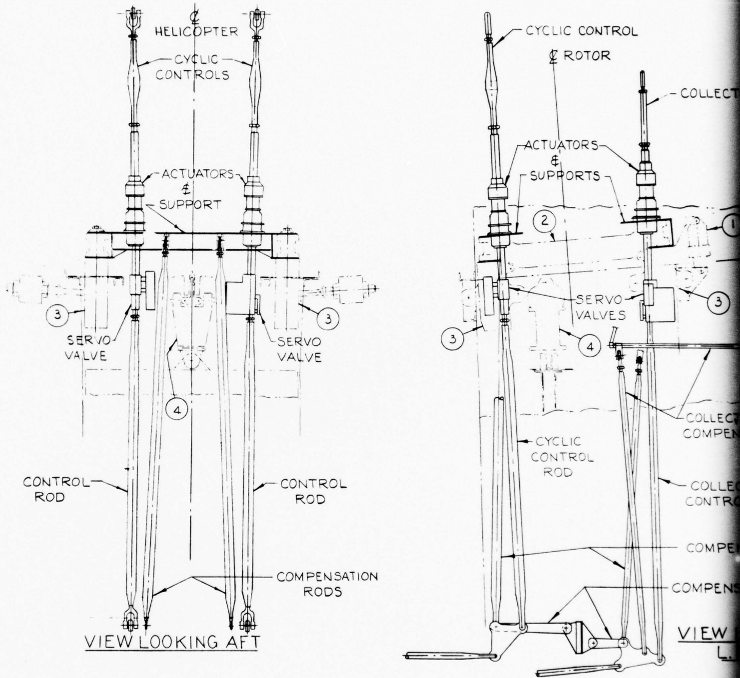
Figure 70. UH-1H Isolated Controls Rotor Isolation Program
