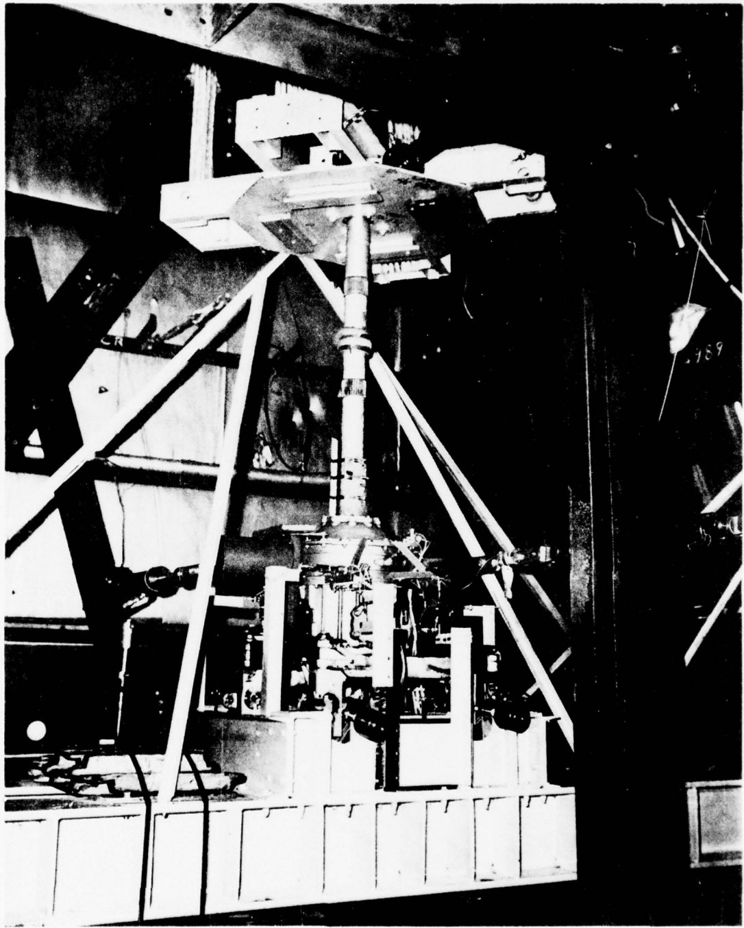
Figure 87. Endurance Rig
