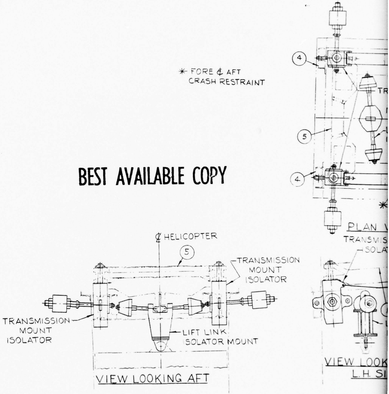
Figure 63. Rotor Isolation System UH-1H Modified
