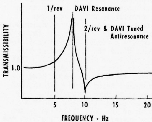
Figure 1. Two-Bladed Case
