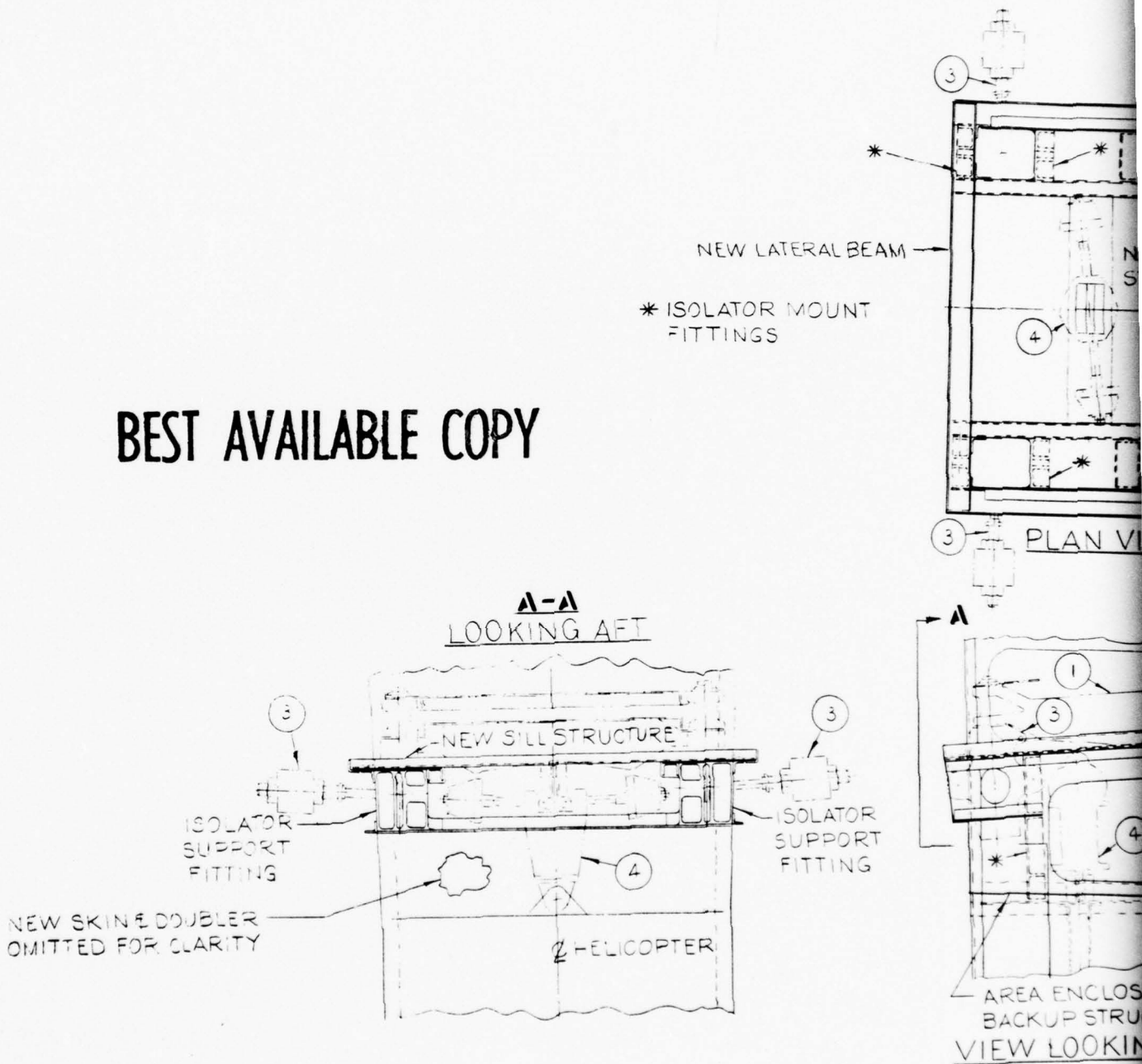
Figure 65. Modified Structure Rotor Isolation System
