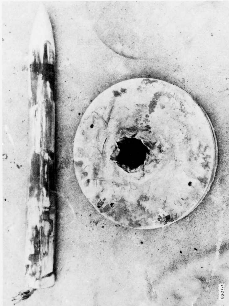
Figure 46. Model PSA-2 post test condition and media projectile aluminum base.
