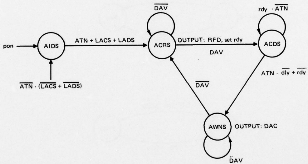
Figure A35. GPIB Acceptor Handshake state diagram.
