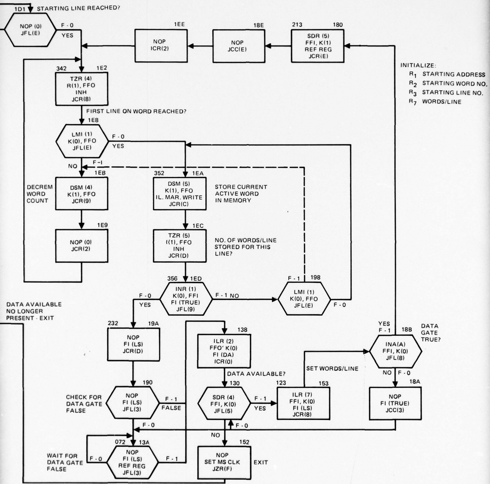
Figure A46. CAPTURE microprogram flowchart.
