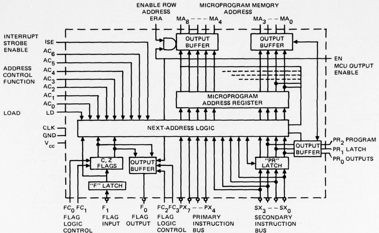
Figure A43. 3001 block diagram.
