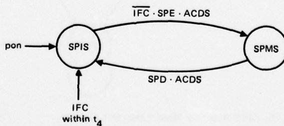
Figure A36. GPIB Talker Extended state diagram.
