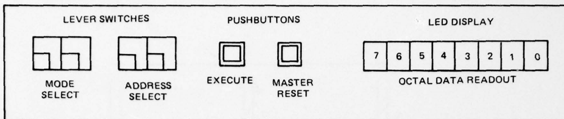
Figure A31. DIA front-panel controls.
