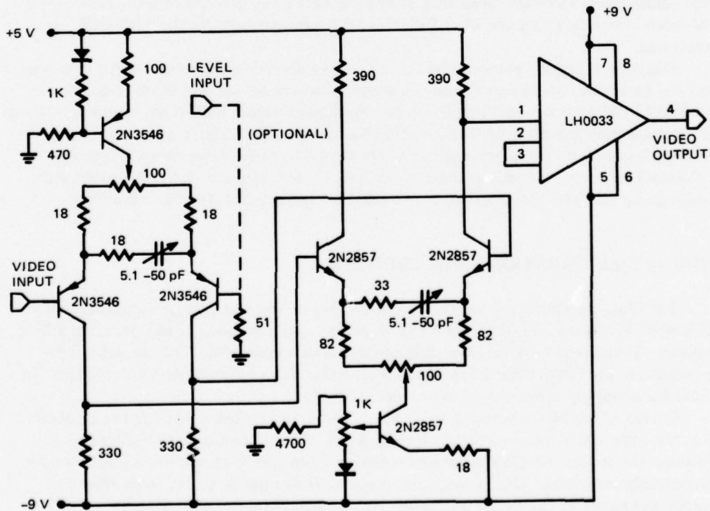
Figure A10. Two-stage video amplifier.
