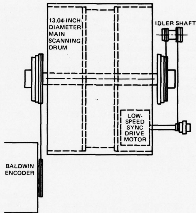
Figure B10. Variable resolution with existing drum design.
