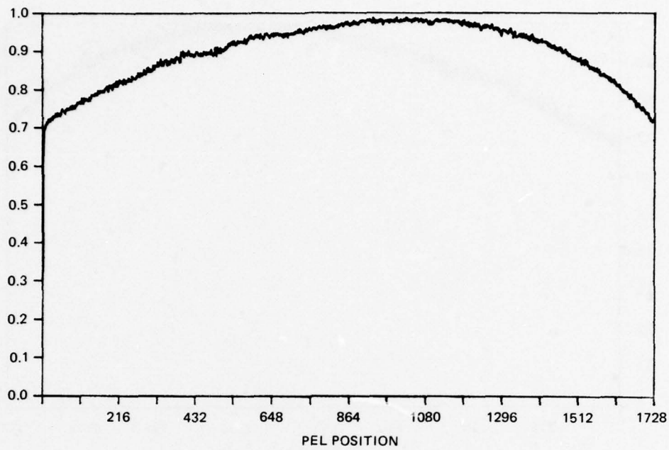
Figure D3. Smoothed illumination profile, 10-bit, 3 pels averaged, 09/15/77.
