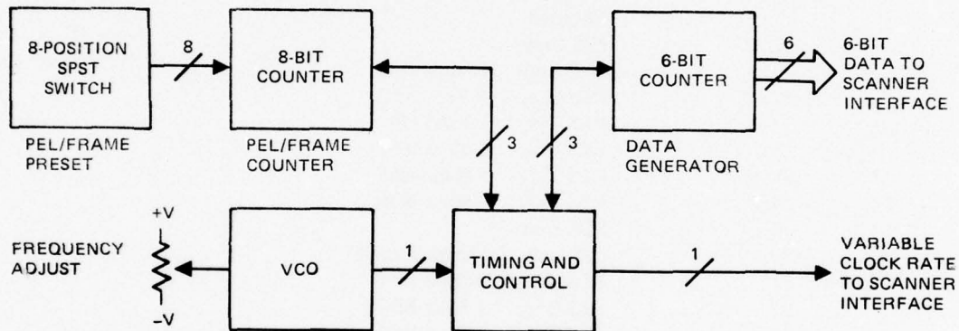
Figure A30. DIA built-in test equipment.
