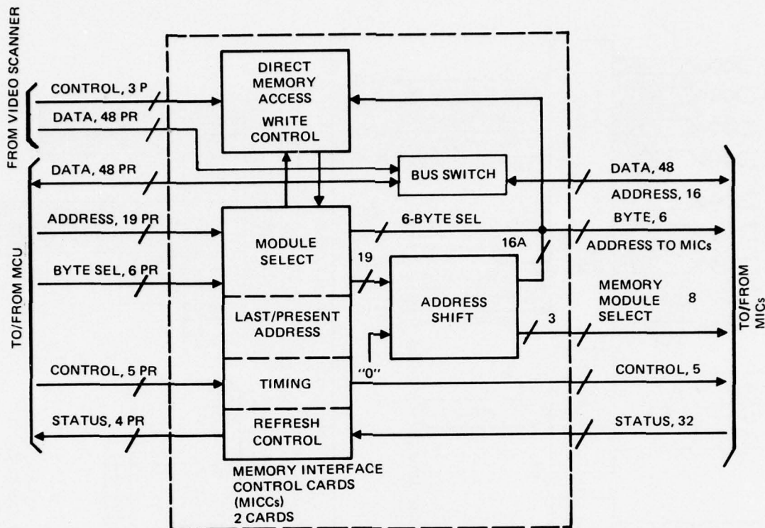
Figure A23. Memory interface control card block diagram.
