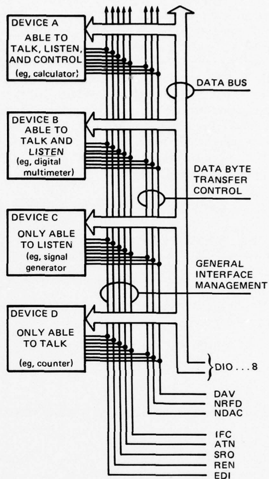
Figure A33. GPIB interface capabilities and bus structure.
