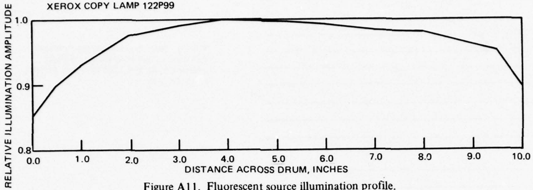
Figure A11. Fluorescent source illumination profile.
