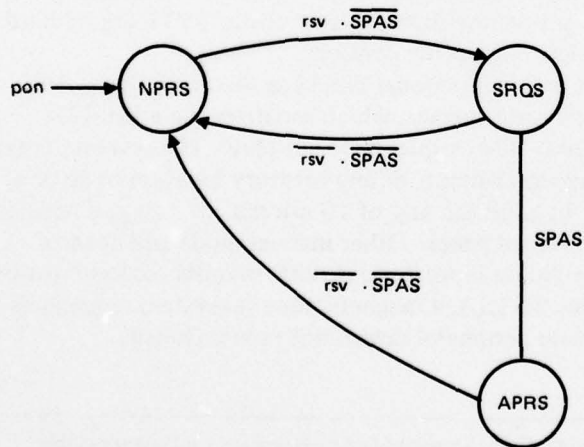
Figure A38. GPIB Service Request state diagram.
