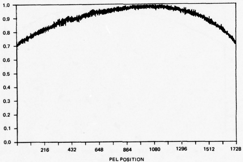
Figure D2. Illumination profile, 10/03/77, 10-bit, defocused, NOSC #35, file 3.
