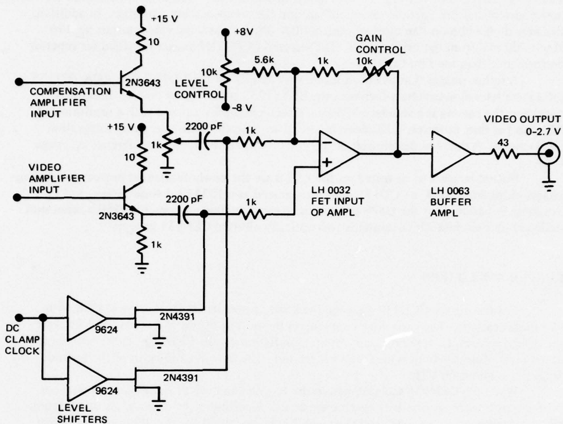
Figure A5. Buffer amplifier for CCD121H.
