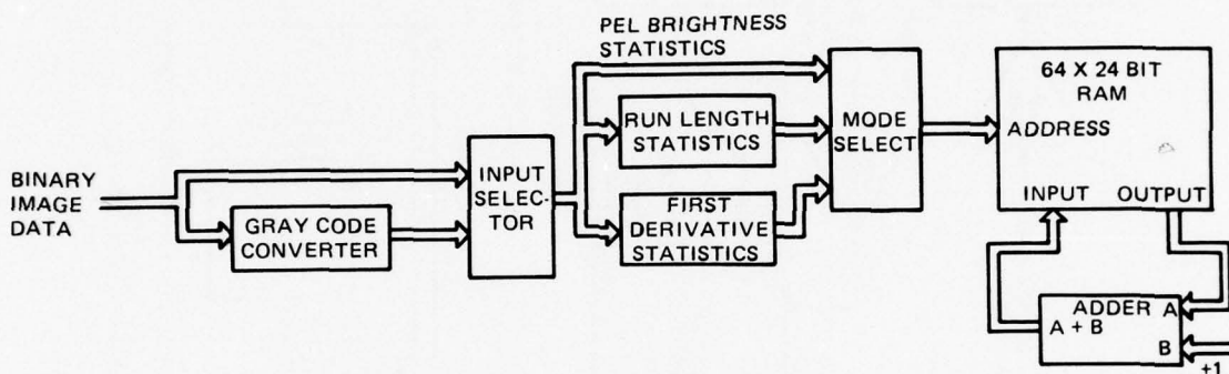
Figure A27. DIA simplified block diagram.
