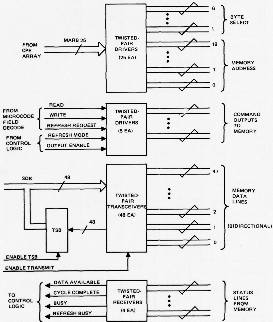
Figure A19. Memory interface.
