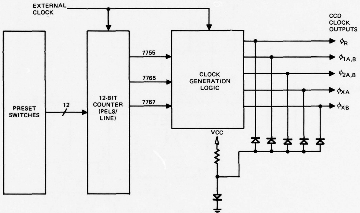
Figure A7. Clock driver circuit.
