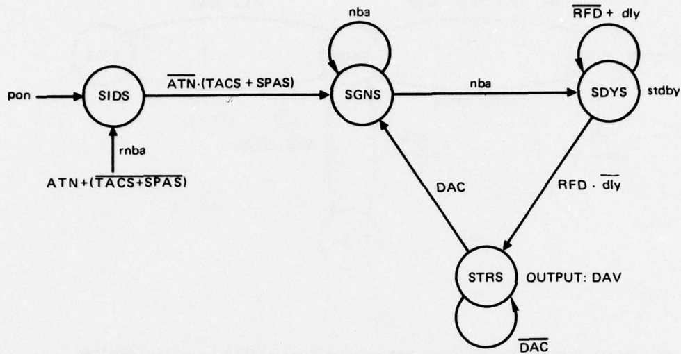
Figure A34. GPIB Source Handshake state diagram.
