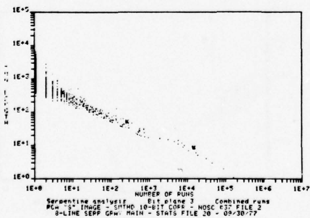
Figure D25. Run length statistics.
