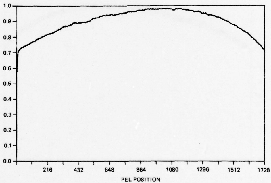
Figure D4. Smoothed illumination profile, 10-bit, 11 pels averaged, 09/27/77, NOSC tape #35, file 01.
