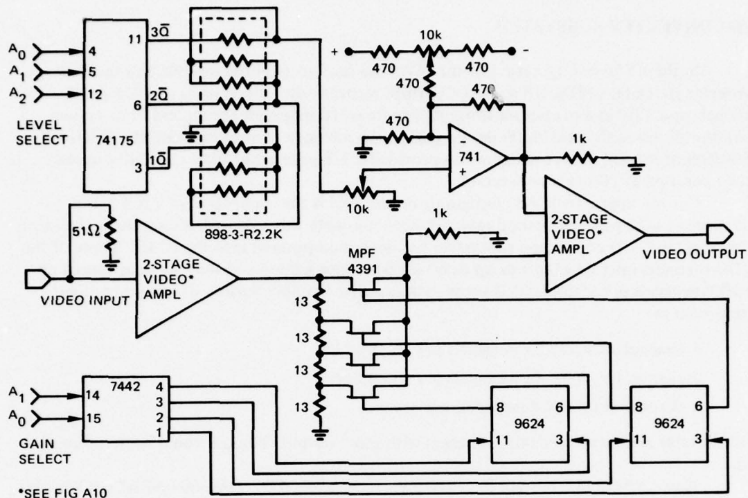
Figure A9. Gain and level amplifier with digital control.
