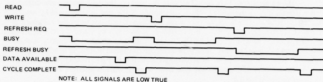
Figure A20. Memory timing.
