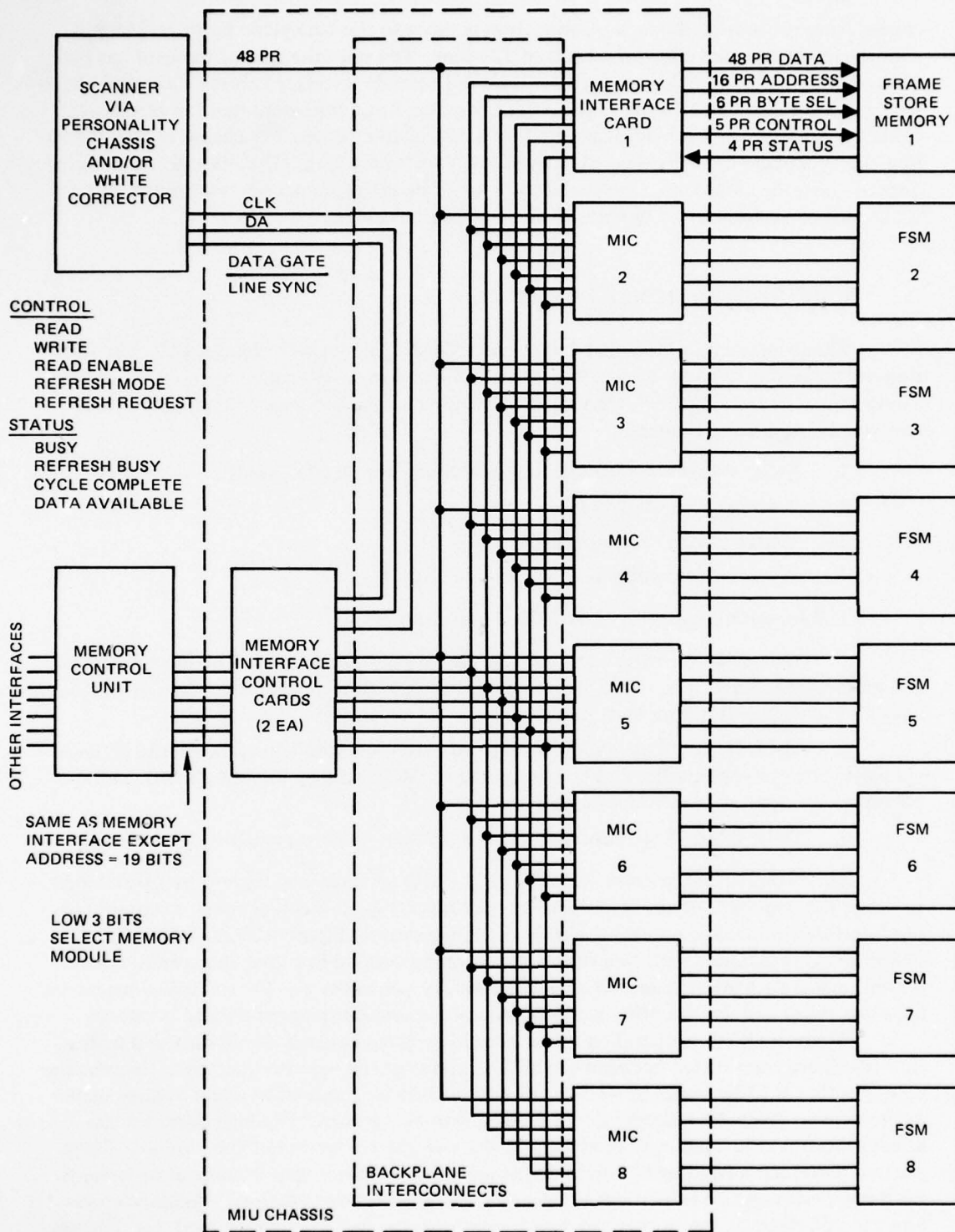
Figure A21. Memory Interface Unit.
