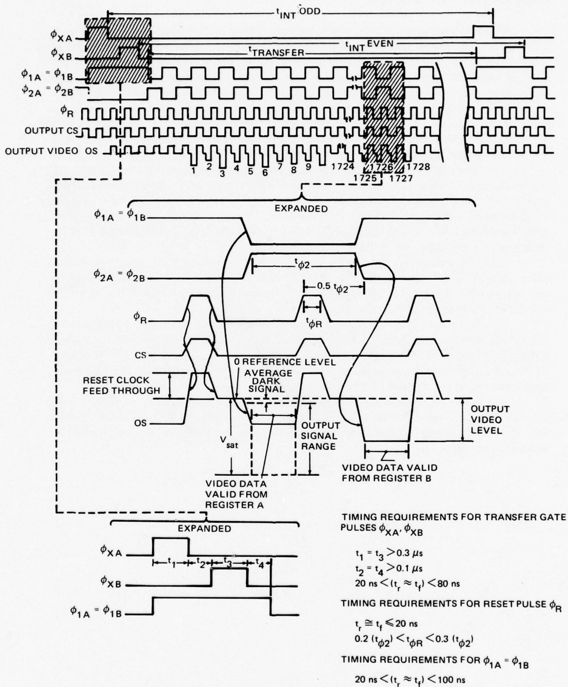
Figure A8. Transfer gate timing diagram.
