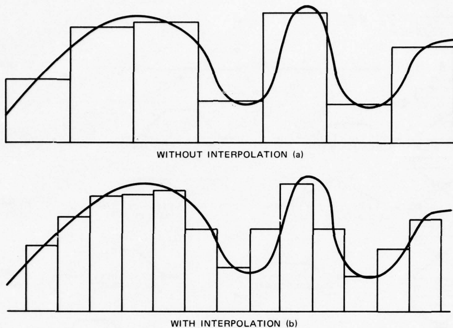
Figure C14. Effect of linear interpolation on a video waveform.
