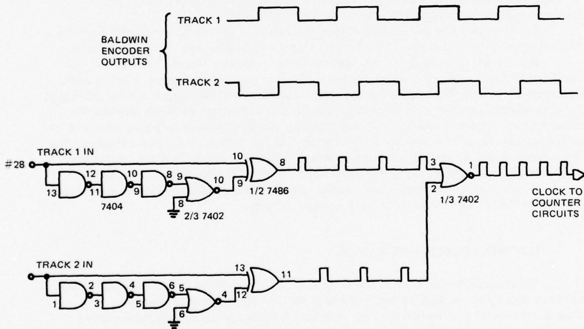
Figure B11. Clock track pulse generator logic diagram.
