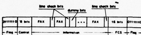
Fig.5 Frame structure
