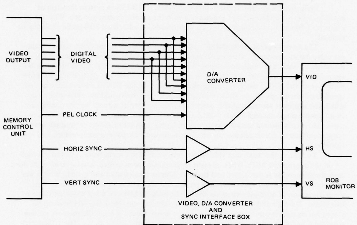
Figure A24. Video output interface.
