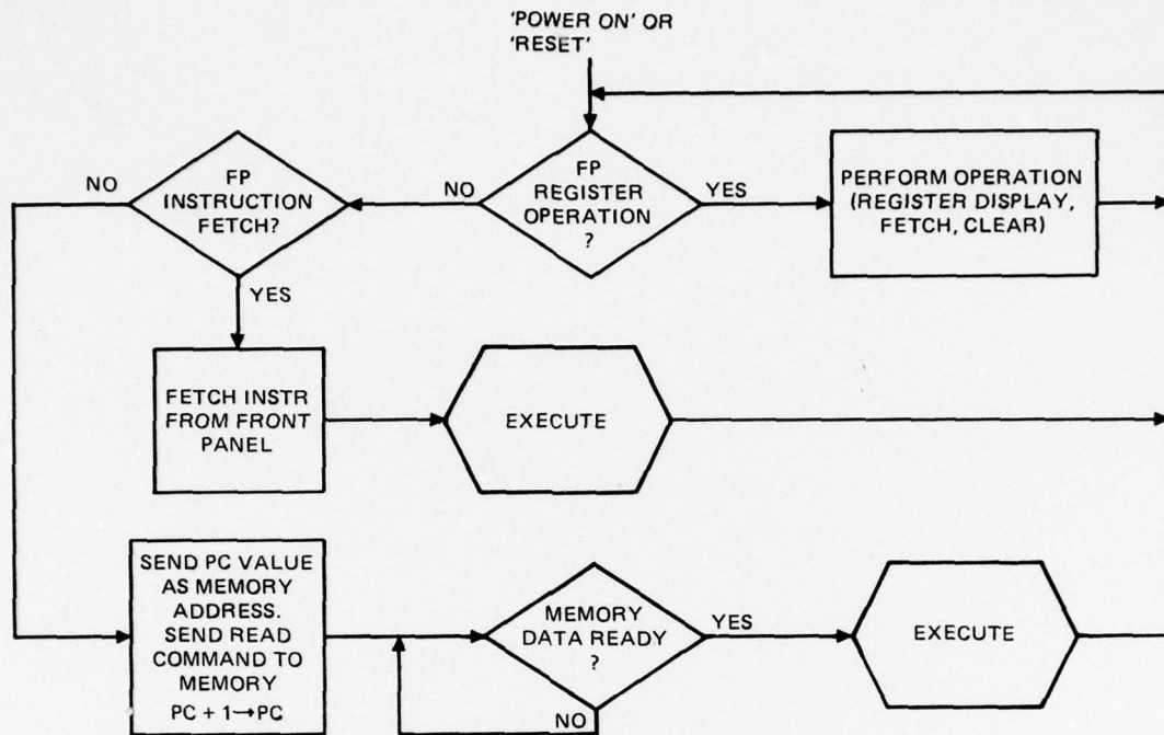
Figure A45. Microprogrammed fetch cycle.
