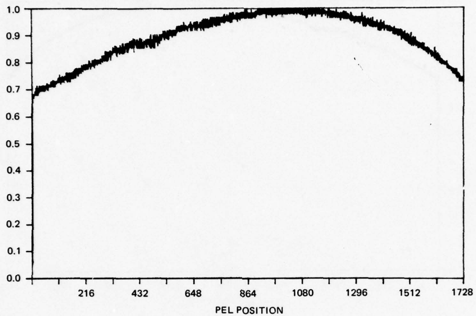
Figure D1. Illumination profile, 09/12/77, 10-bit, focused, NOSC #34, file 0.
