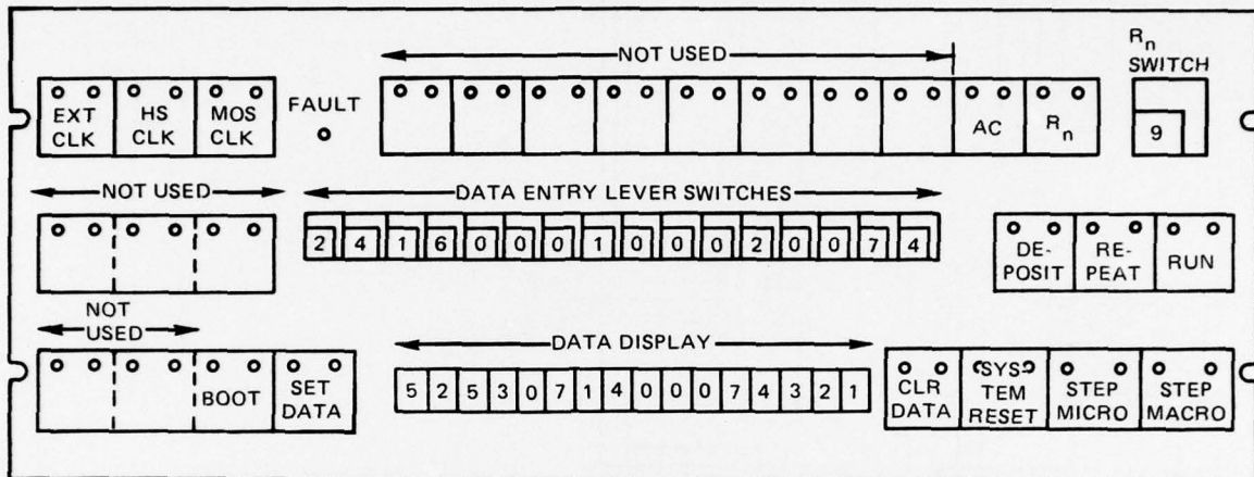
Figure A42. MCU manual control panel.
