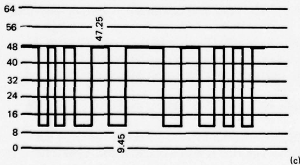
Figure A12. Illumination correction.
