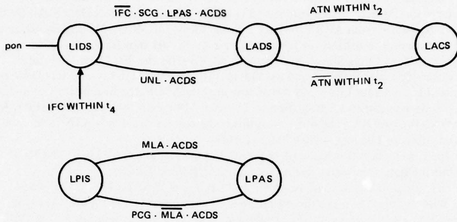
Figure A37. GPIB Listener Extended state diagram.
