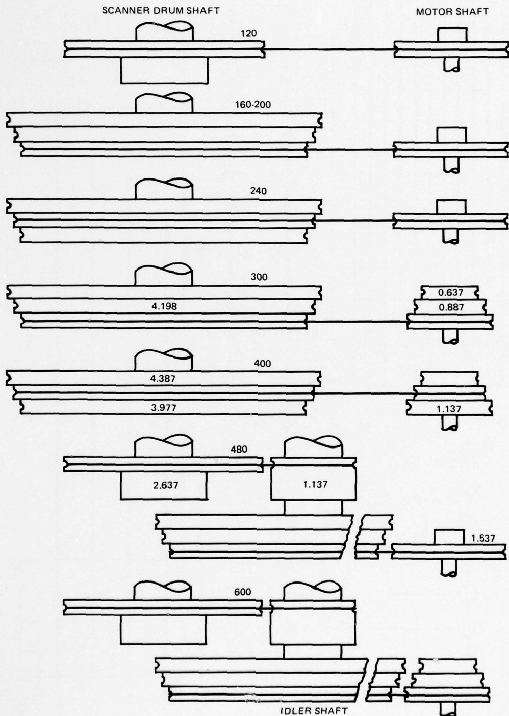
Figure B13. Variable resolution pulley connections.
