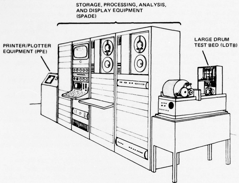
Figure A3. Image capture and analysis system (ICAS).
