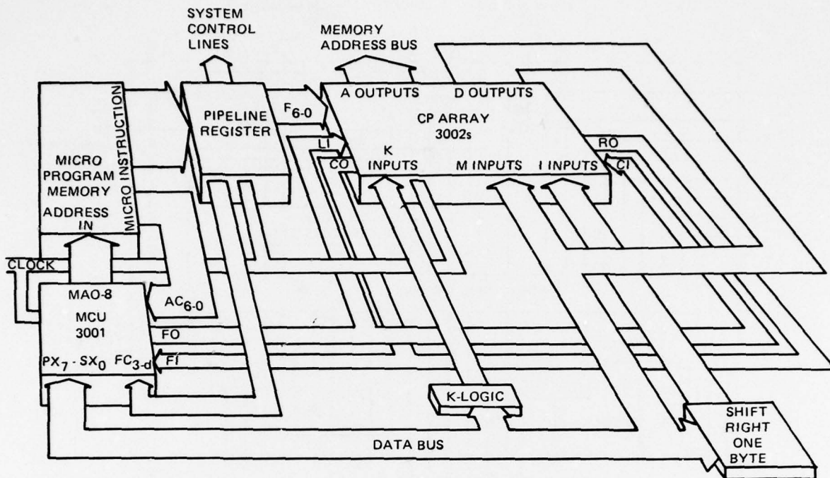
Figure A44. Microcontrol block diagram.
