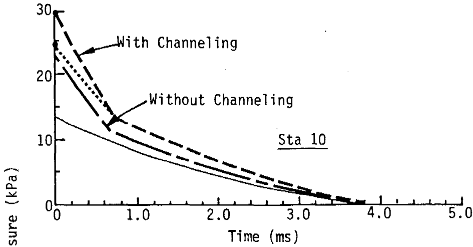
A. Overpressures along Line C-1 from a Burst over GZ "C".
