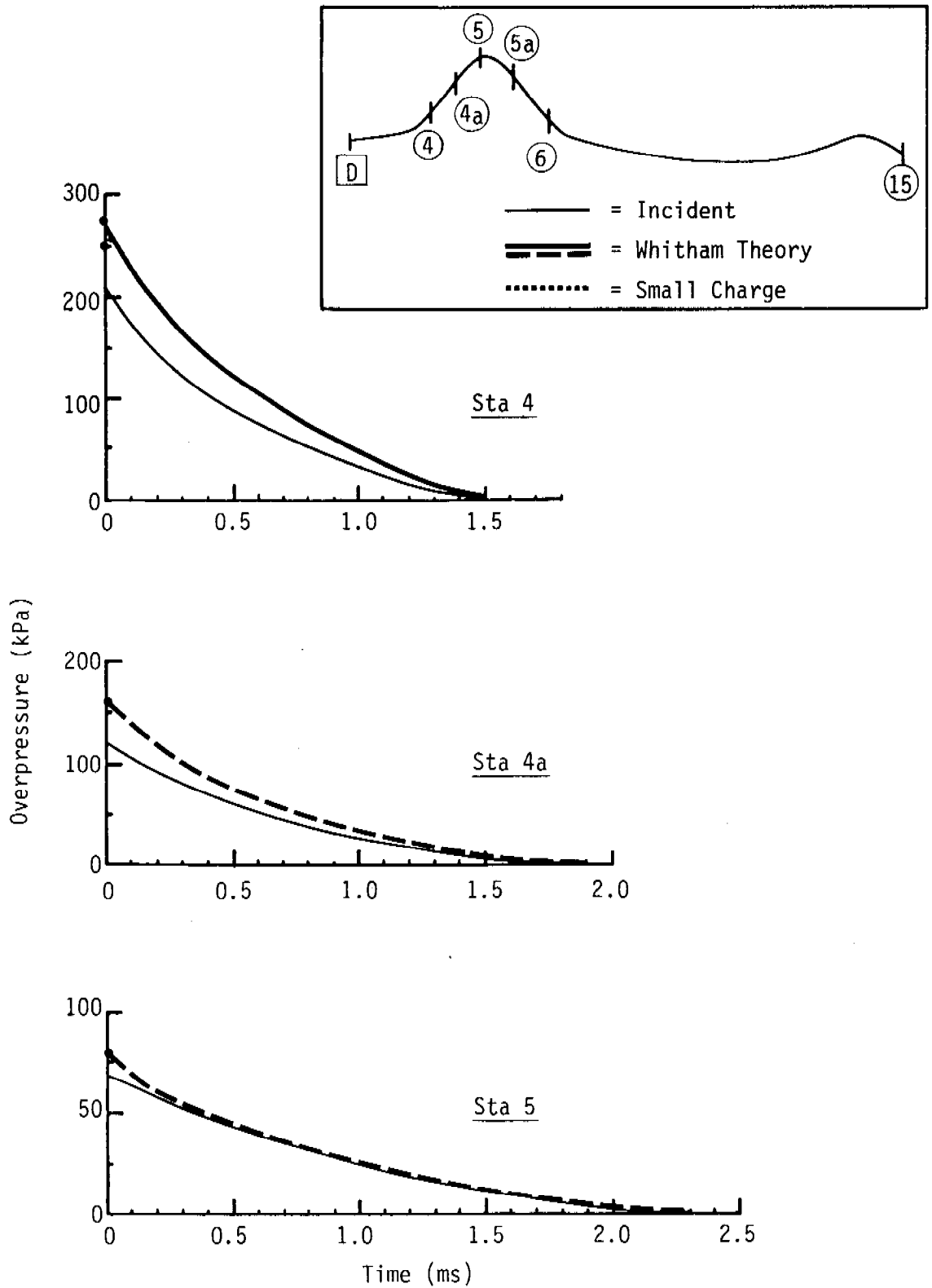
Fig. A-10a. Overpressures along Line D-1 from a Burst over GZ "D".
