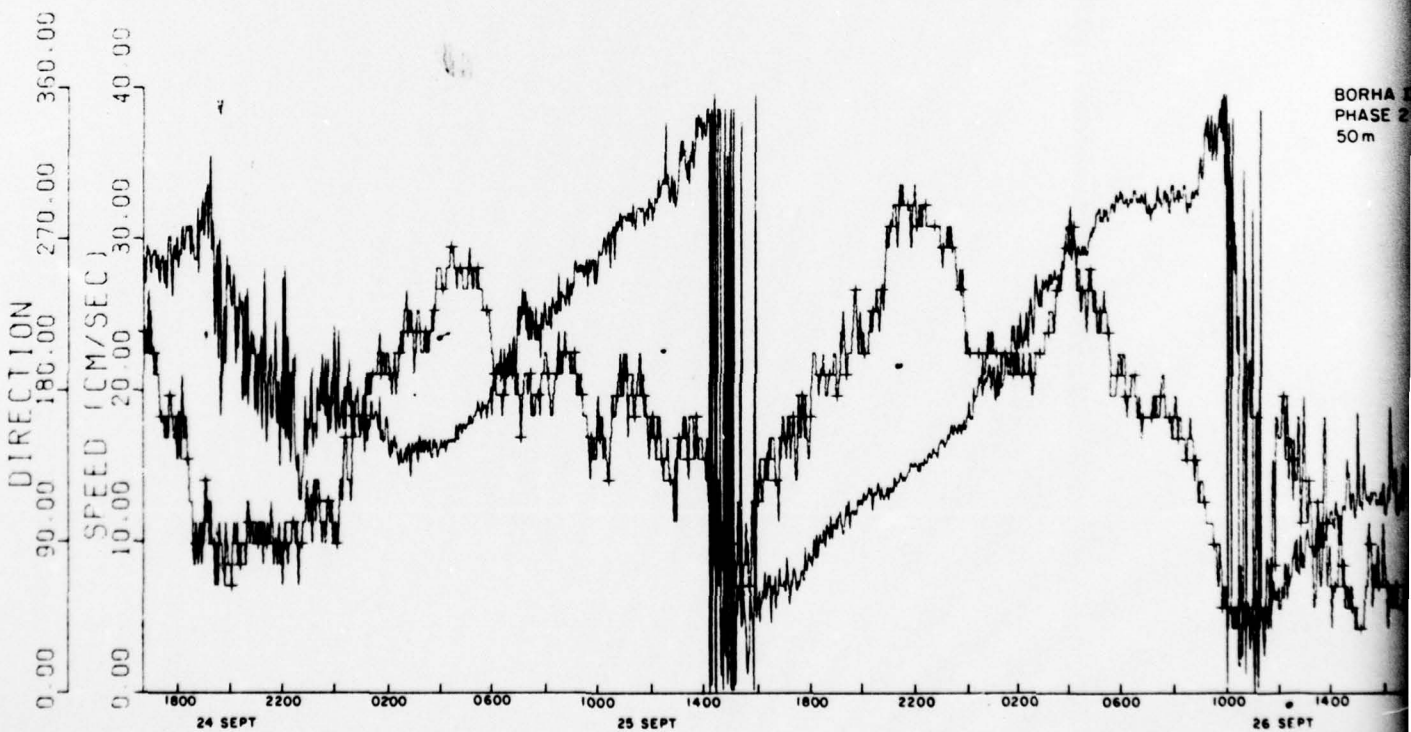
CURRENT SPEED AND DIRECTION, BORHA II, PHASE II.
