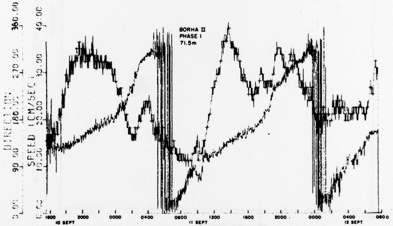
FIGURE 28. CURRENT SPEED AND DIRECTION, BORHA II, PHASE I.
