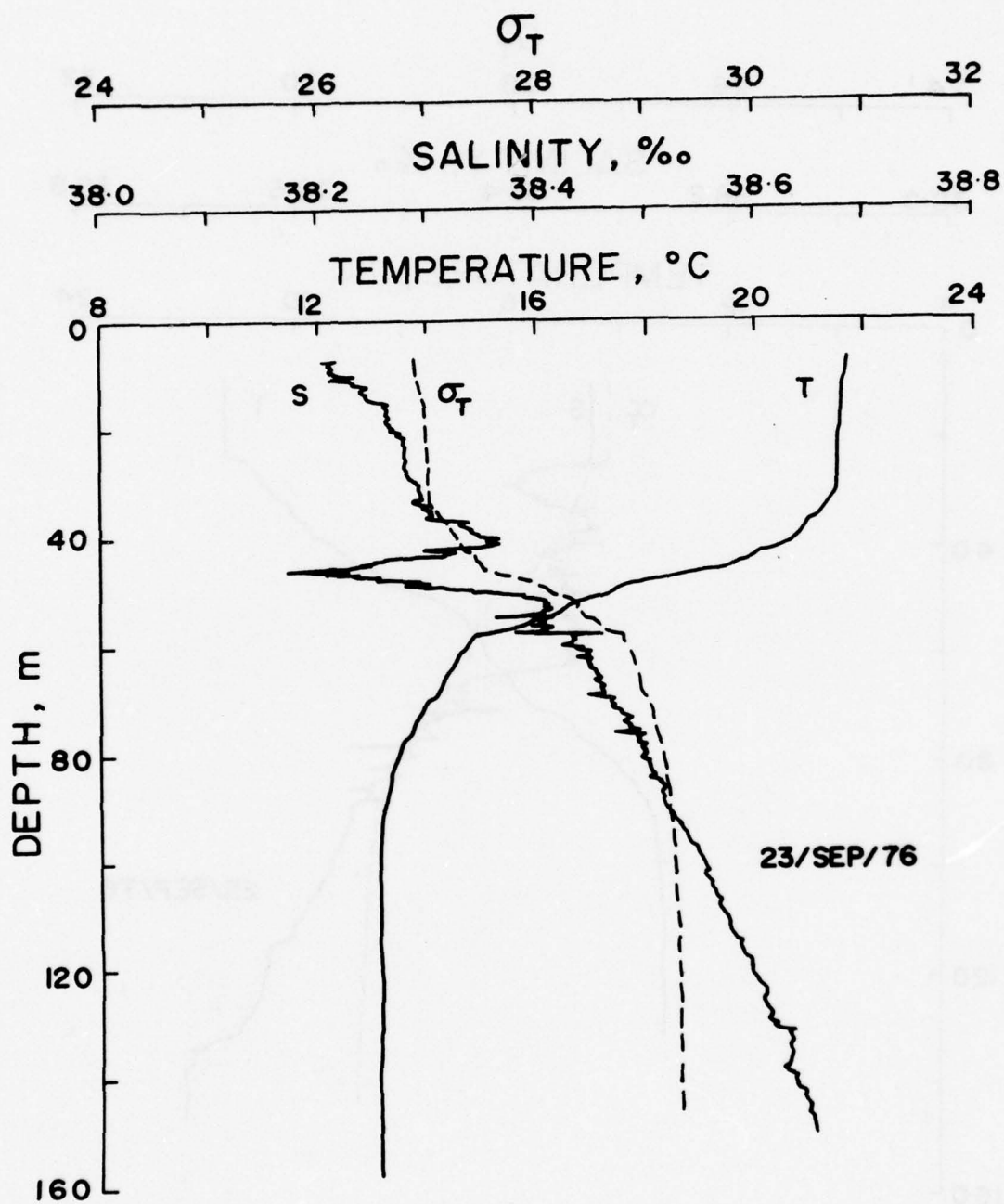
FIGURE 17. CTD PROFILE FROM THE MAGNAGHI, 1850(A+1)/23/SEP/76
