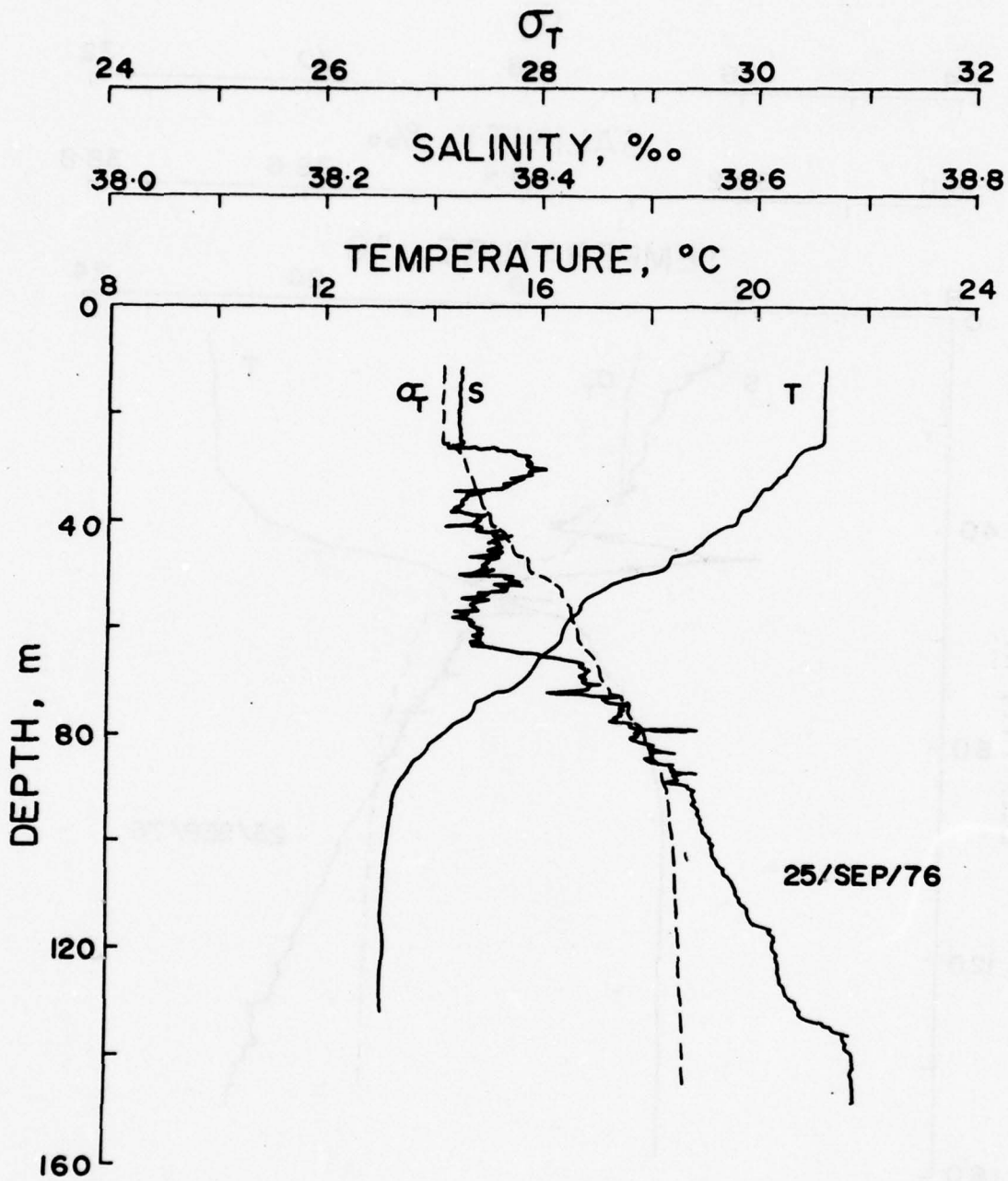
FIGURE 18. CTD PROFILE FROM THE MAGNAGHI, 0925(A+1)/25/SEP/76
