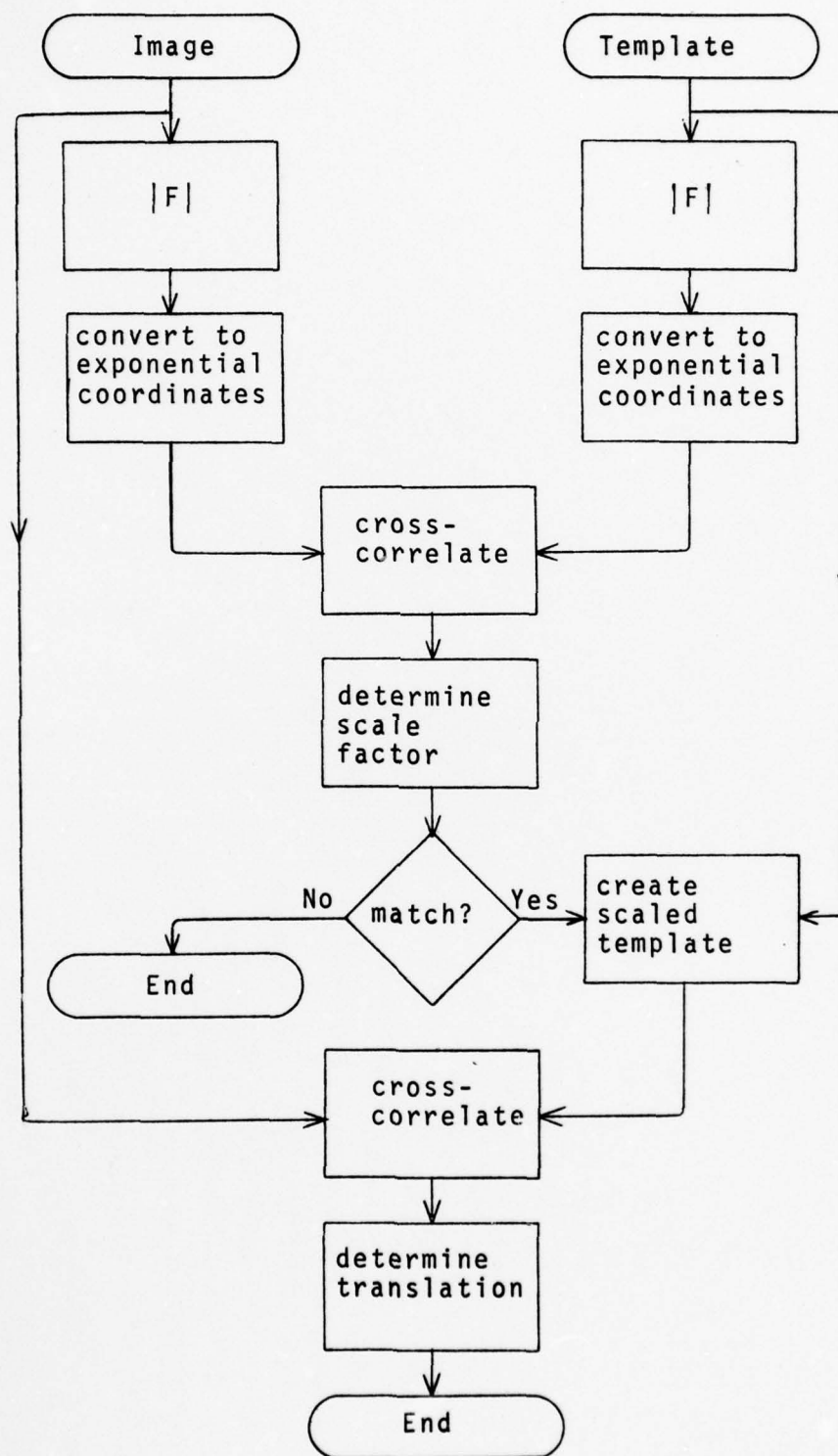
Figure 2 One-dimensional generalized correlation. Magnitude method.
