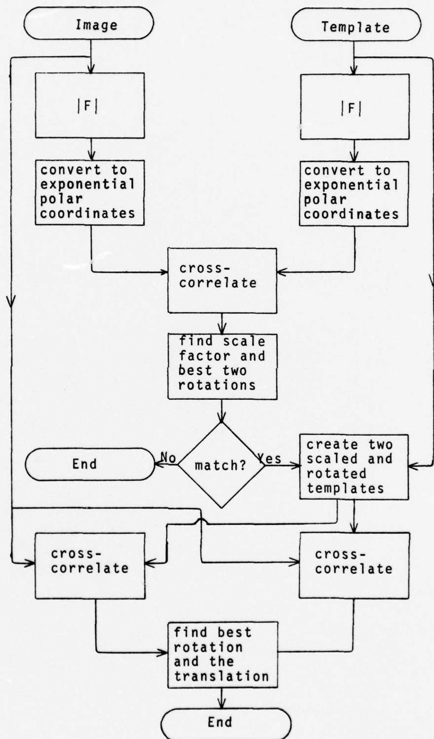
Figure 3 Two-dimensional generalized correlation. Magnitude method.
