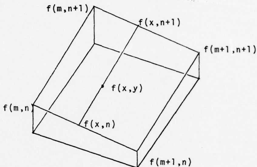
Figure 5. Bilinear interpolation.
