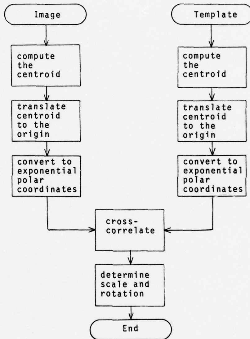
Figure 4 Two dimensional generalized correlation. Centroid method.
