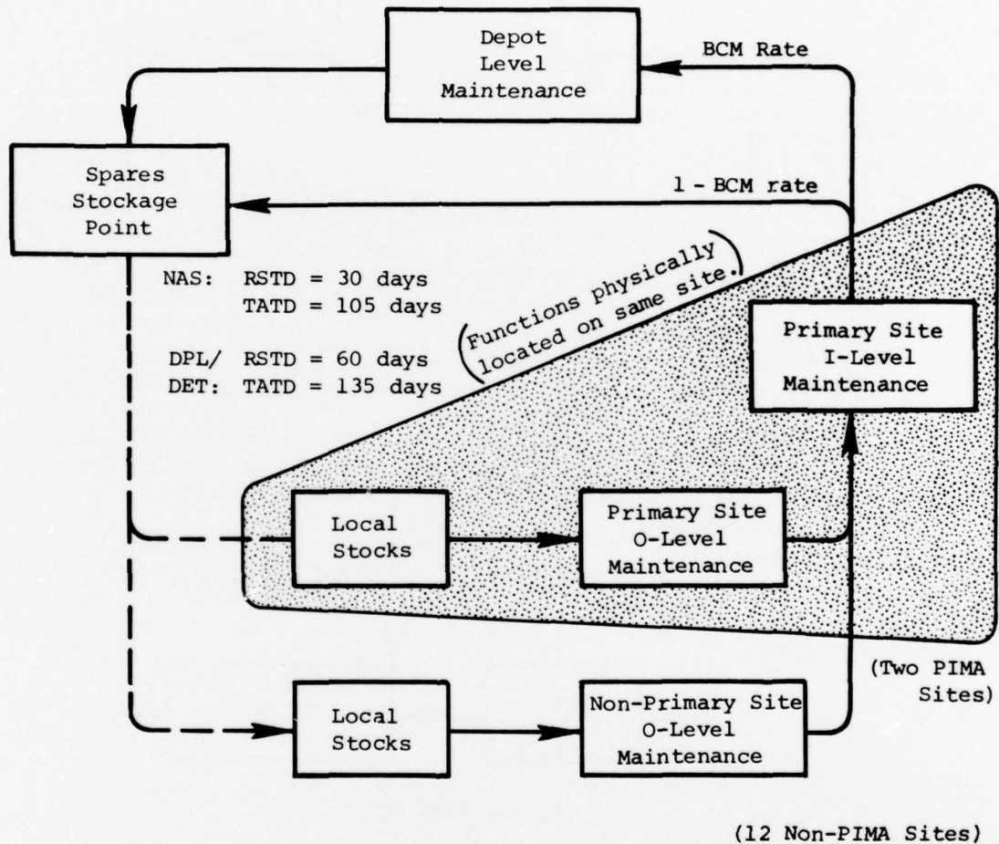
Figure 4. SPARES INVENTORY FLOW DIAGRAM, OPTION 4 (TWO PIMAs)
