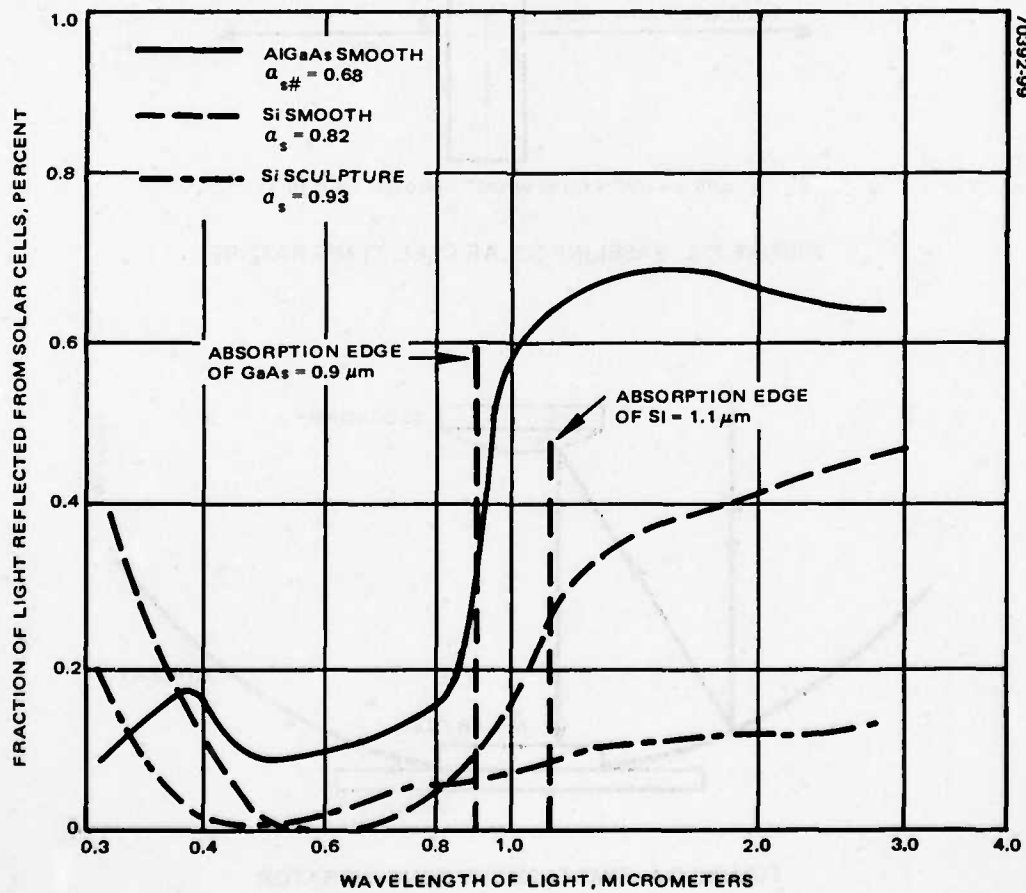
FIGURE C-2. SOLAR ABSORPTIVITY OF SOLAR CELLS
