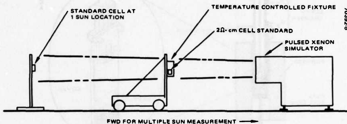
FIGURE 5. TEST METHOD FOR DETERMINING SOLAR CELL CURRENT-VOLTAGE CHARACTERISTICS
