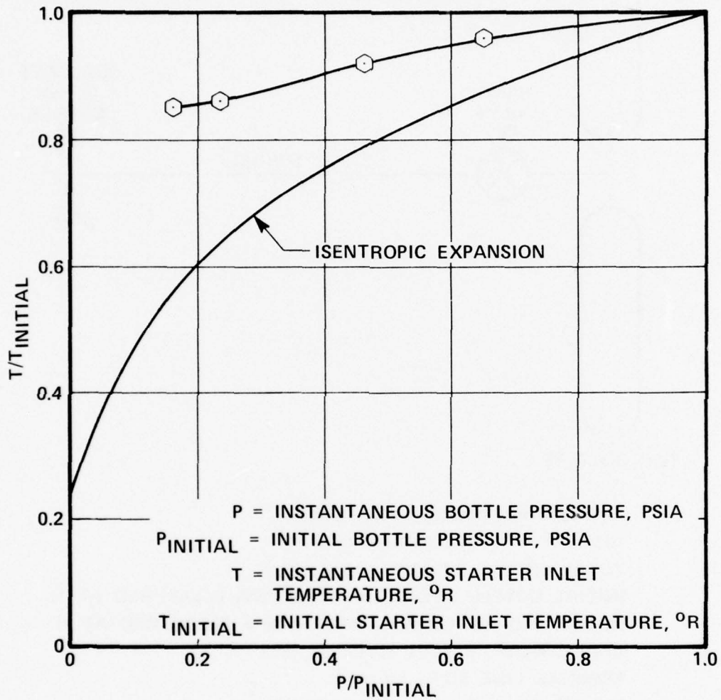
Figure A-20. Comparison of experimental bottle blowdown test data with isentropic expansion.
