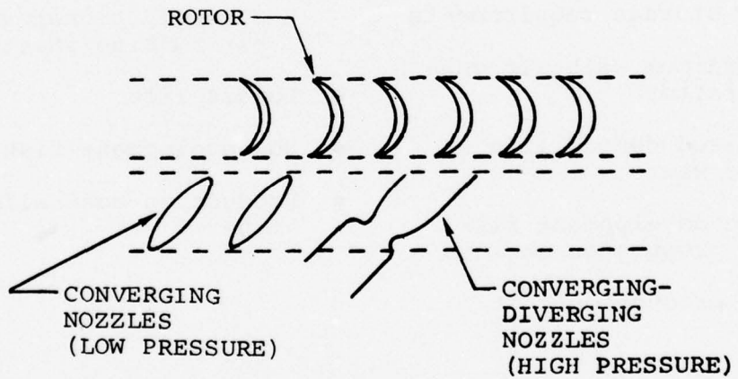
AIR TURBINE STARTER
