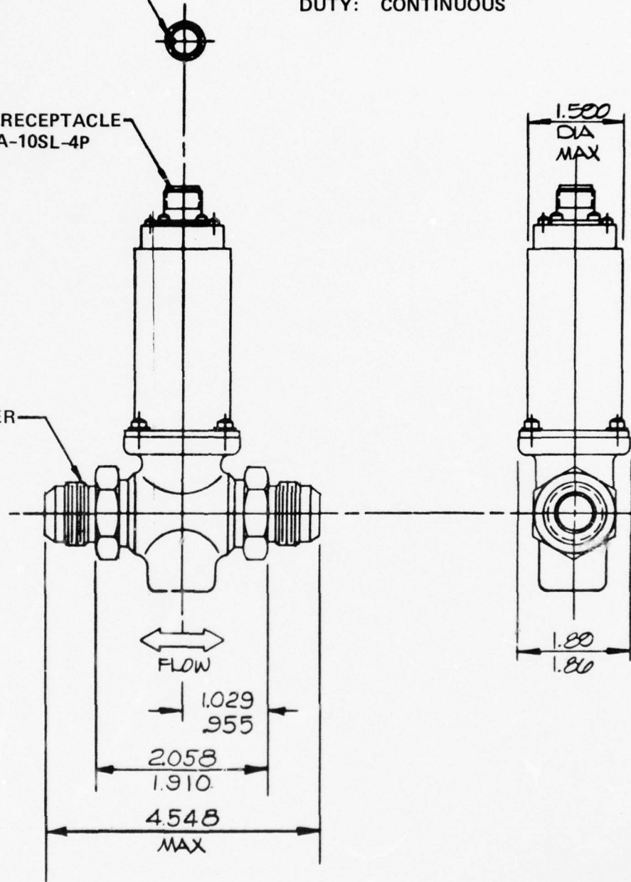
Figure B-9. Solenoid shutoff valve.
