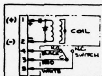
WIRING DIAGRAM (SHOWN DE-ENERGIZED)
