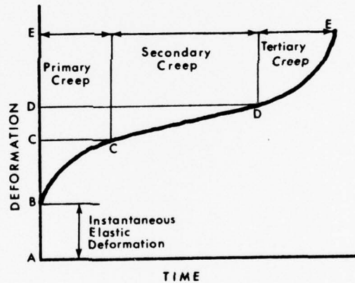
Figure 1. Typical creep curve at constant temperature and stress.
