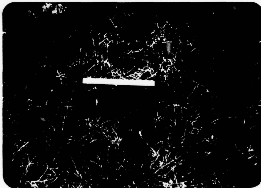
Figure 18 - Fissuring of soil along upper wall of a shrinkage crack.
