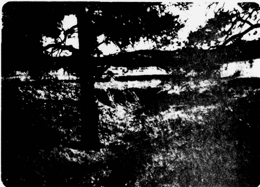
Figure 10. Two concentric vertical headcuts. The upper one may be a result of subsurface piping.
