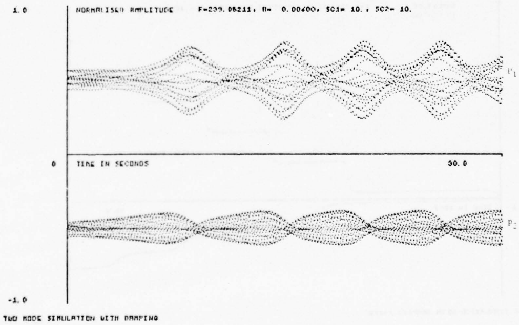
Fig. 4.5.7. Excitation at 2\omega_2 , full equations
