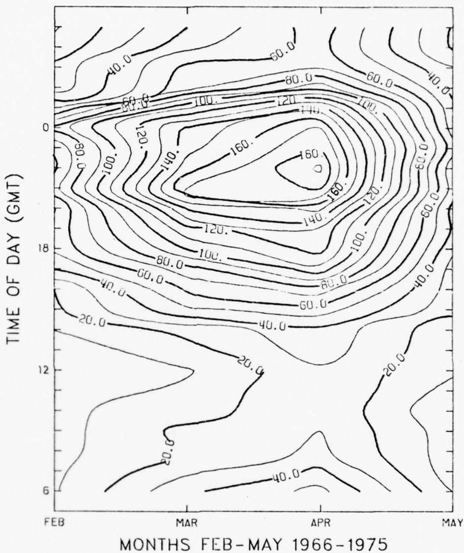
Fig. 19. Contoured frequency graph depicting the comparison of monthly dust observations with time of day of occurrence. Contours are labeled in number of observations and the data base includes 5056 dust reports from 34 Southern Great Plains stations during February-May 1966-1975.
