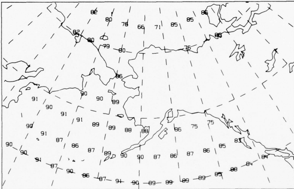
Figure 71. Base coverage reliability map (top) and coverage reliability map (bottom) for the following: additional stations - Adak and Barrow, 4, 6, and 8 MHz, summer night and high solar activity.
