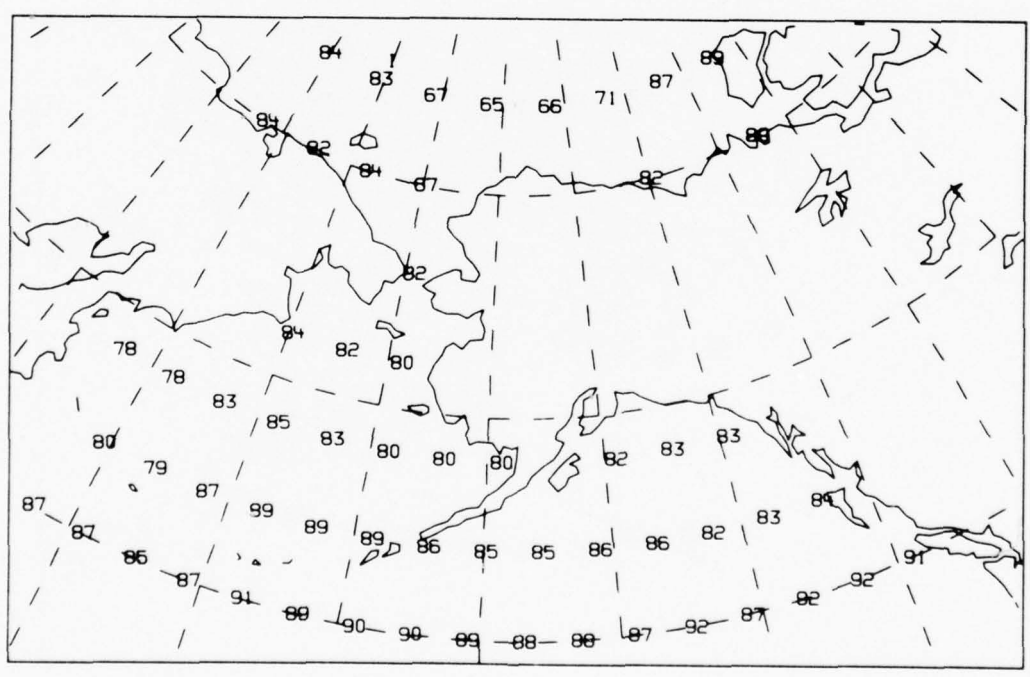
Figure 59. Base coverage reliability map (top) and coverage reliability map (bottom) for the following: additional station - Barrow, 4, 6 and 8 MHz, summer night and low solar activity.
