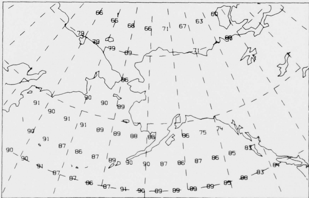
Figure 65. Base coverage reliability map (top) and coverage reliability map (bottom) for the following: additional station - Adak, 4, 6, and 8 MHz, summer night and high solar activity.
