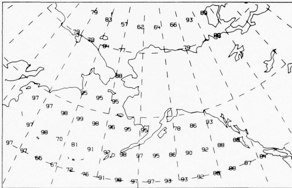
Figure 46. Base coverage reliability map (top) and coverage reliability map (bottom) for the following: additional stations - Adak and Barrow, 8 MHz, summer day and low solar activity.
