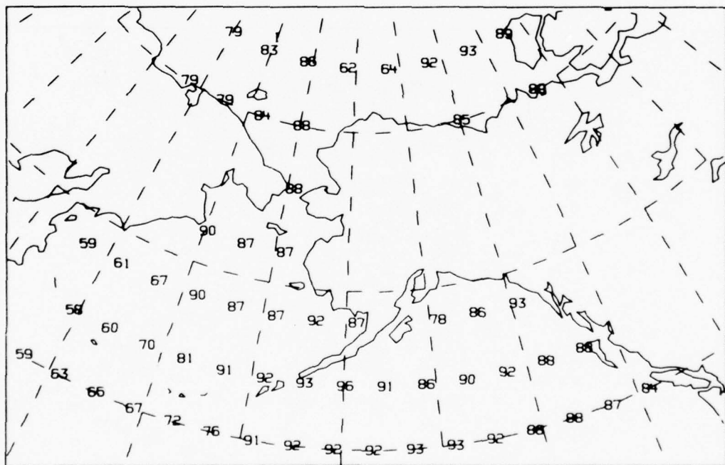
Figure 42. Base coverage reliability map (top) and coverage reliability map (bottom) for the following: additional station - Barrow, 6 and 8 MHz, summer day and low solar activity.
