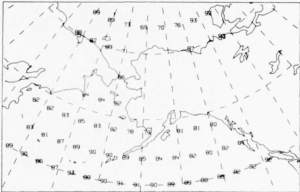
Figure 33. Base coverage reliability map (top) and coverage reliability map (bottom) for the following: additional station - Barrow, 4 and 6 MHz, winter night and high solar activity.
