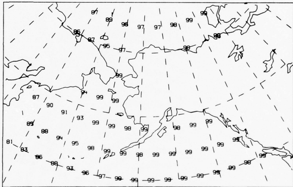
Figure 5. Base coverage reliability map (top) and coverage reliability map (bottom) for the following: additional station - Barrow, 4, 6, and 8 MHz, winter day and low solar activity.
