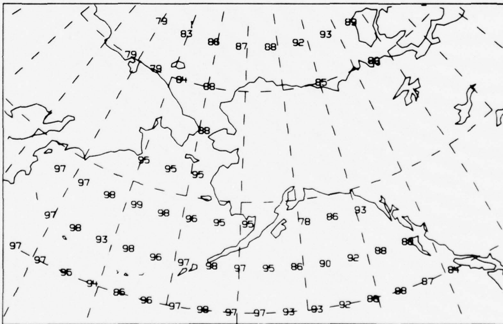
Figure 44. Base coverage reliability map (top) and coverage reliability map (bottom) for the following: additional stations - Adak and Barrow, 4, 6, and 8 MHz, summer day and low solar activity.
