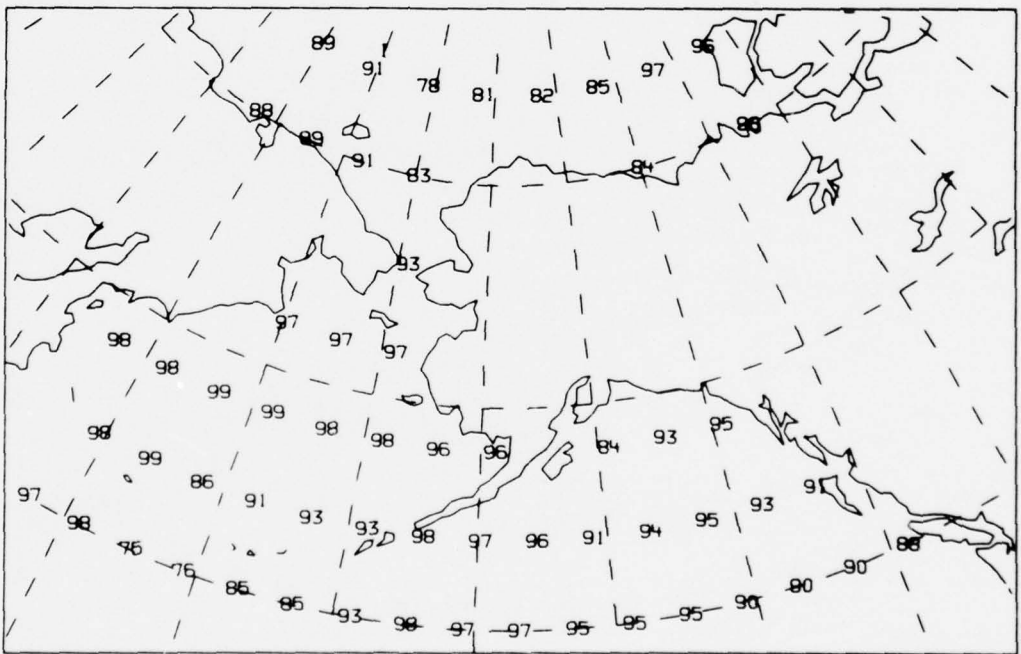
Figure 19. Base coverage reliability map (top) and coverage reliability map (bottom) for the following: additional stations - Adak and Barrow, 8 MHz, winter day and high solar activity.
