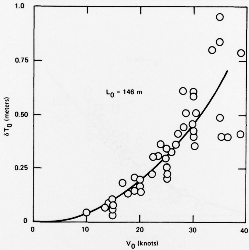
Figure 4 - Sinkage versus Ship Speed for Ships without Bow Domes
