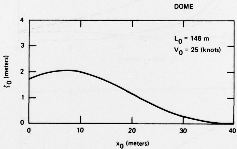
Figure 6 - Analytical Representation of Bow Wave Profile for Ships with and without Bow Domes
