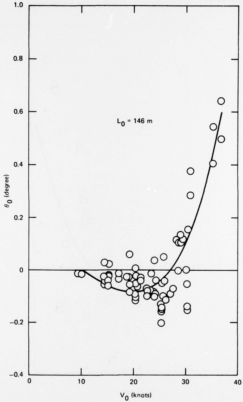
Figure 1 - Trim versus Ship Speed for Ships with Bow Domes
