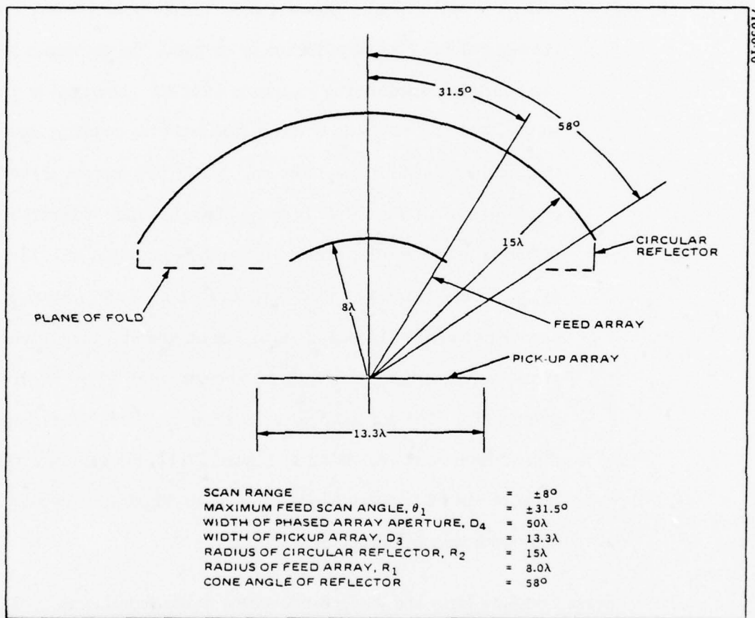
Figure IV.8. Pillbox Design for a 1^\circ Beamwidth and 3 dB Cross Over Level
