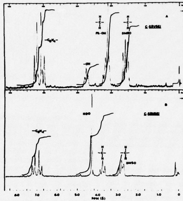
FIG. 2. (A) Nuclear magnetic resonance spectrum of \beta -(4-hydroxyphenyl)ethanol (isolated from C. krusei ) in DMSO-D 6 . (B) Nuclear magnetic resonance spectrum of \beta -(4-hydroxyphenyl)ethanol (isolated from C. krusei ) in DMSO-D 6 + D 2 O.
