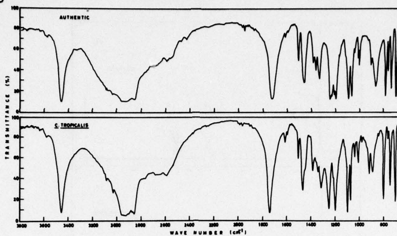
FIG. 4. INFRARED SPECTRA OF ISOLATED AND AUTHENTIC \beta -PHENYLACTIC ACID
