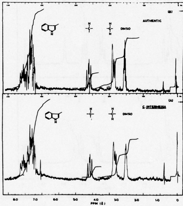
FIG. 5. Nuclear magnetic resonance spectra of (A) isolated and (B) authentic \beta -ILA.
