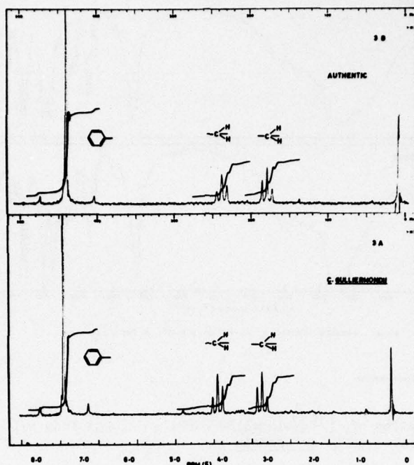
FIG. 5. NUCLEAR MAGNETIC RESONANCE SPECTRA OF ISOLATED (3A) AND AUTHENTIC (3B) \beta -PEA AFTER D_2O EXCHANGE
