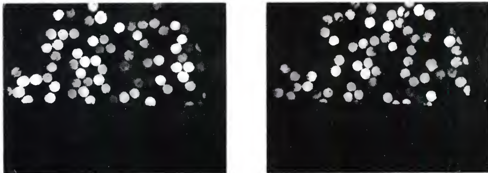
Figure 4. Fiber optic seal fingerprints: seal's fiber optic bundle consists of 180 plastic fibers of 125- \mu\text{m} nominal diam.
