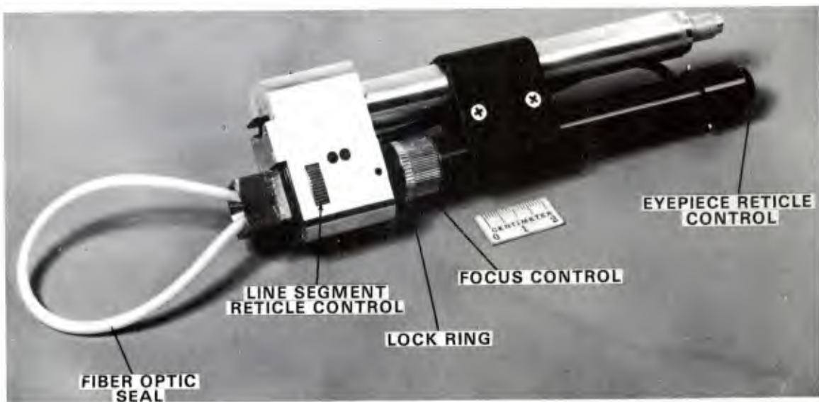
Figure 5. Hand-held viewer showing reticle controls. 0595-76
