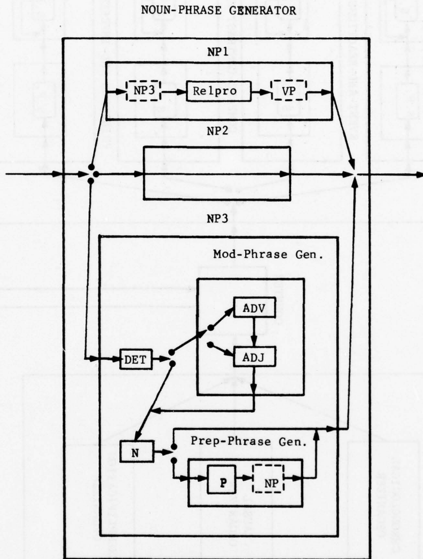
FIGURE 5. Diagram of a Faulty Noun-Phrase Generator Component of the Sentence Generator Device.
