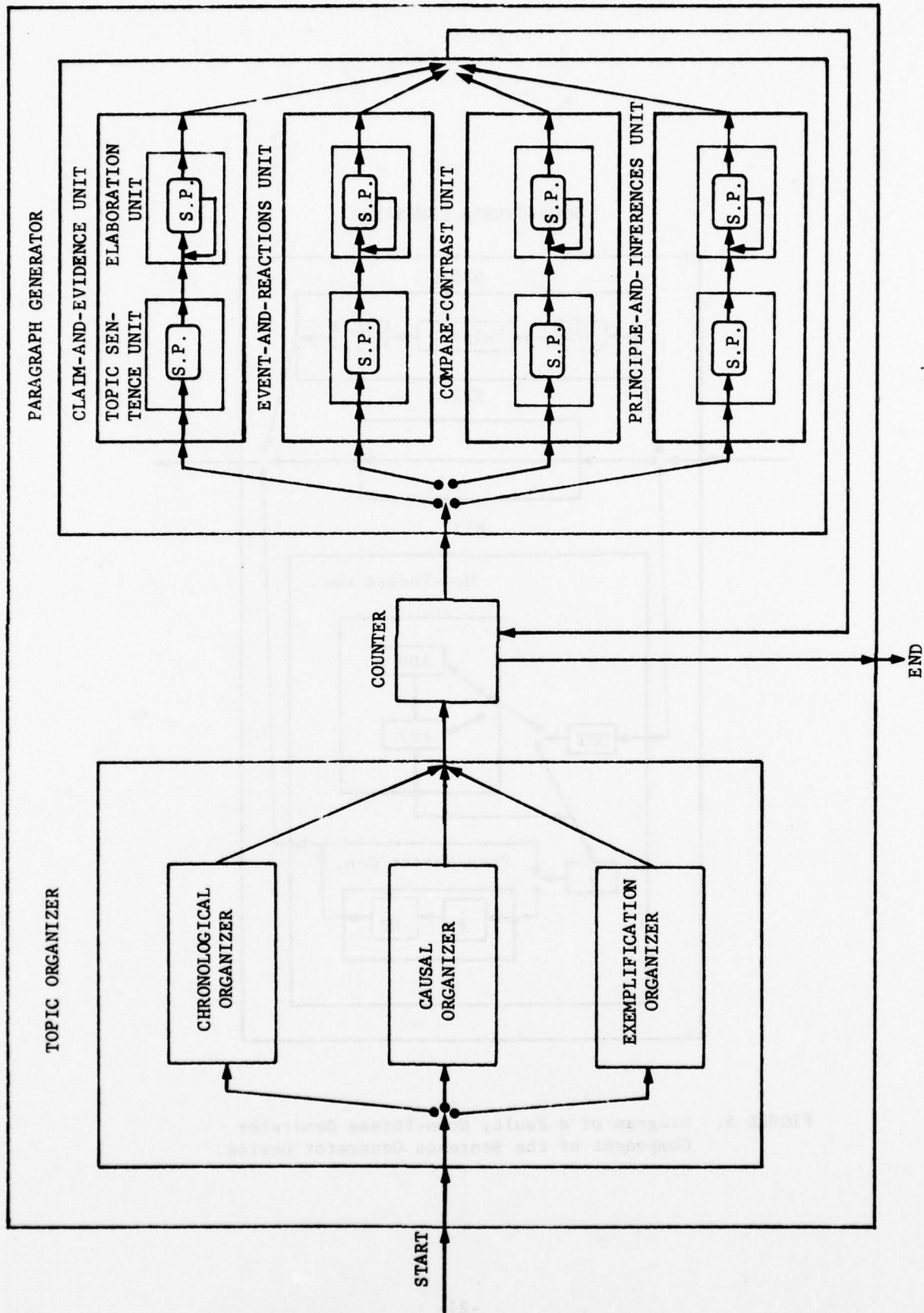
FIGURE 6. Essay Generator.
