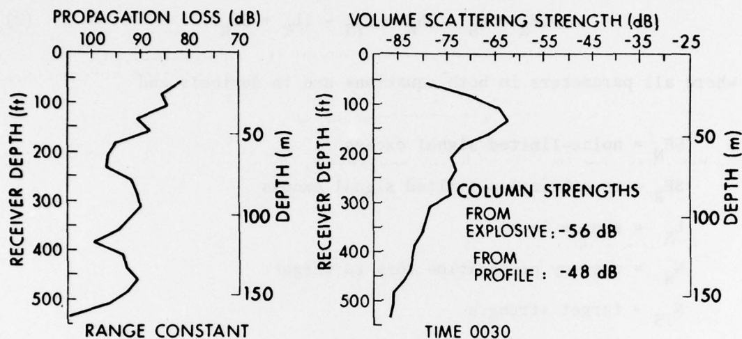
Figure 2. Depth-Dependent Propagation-Loss and Volume-Scattering-Strength Profiles
