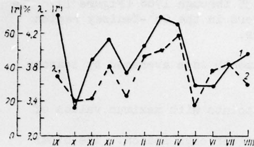
Figure 2. Modulus of correlation coefficients r between the dates of stable icing and the predictor P' (1) and the first eigen values \lambda_1 (2).
