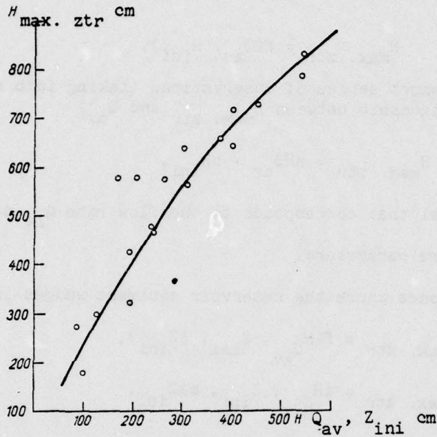
Figure 2. The relationship H_{max. ztr} = f(H_{Q_{av}}, Z_{ini}) for the upper part of the Kaunass reservoir near Birsh-tonas village.
