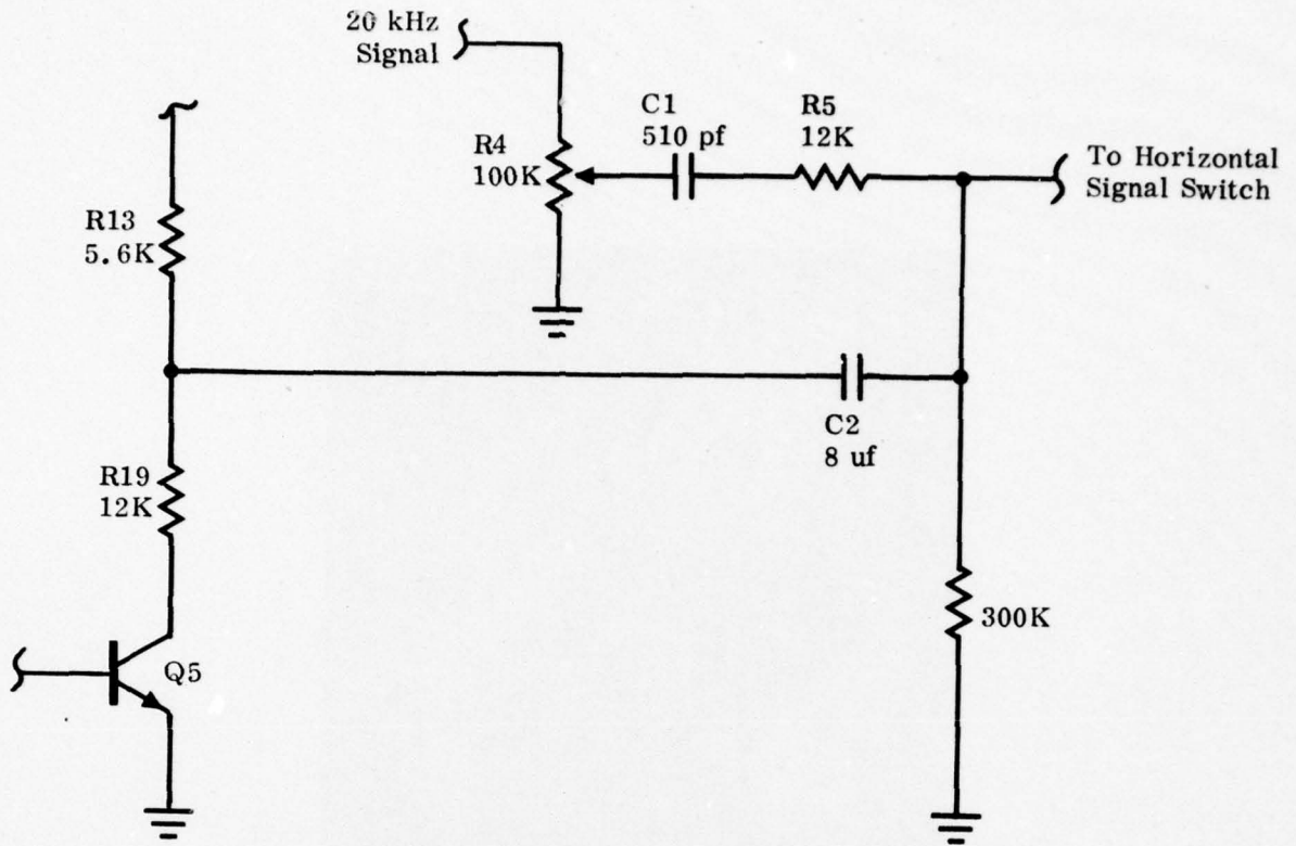
A. Configuration in APQ-100 (All components located on A3710.)
