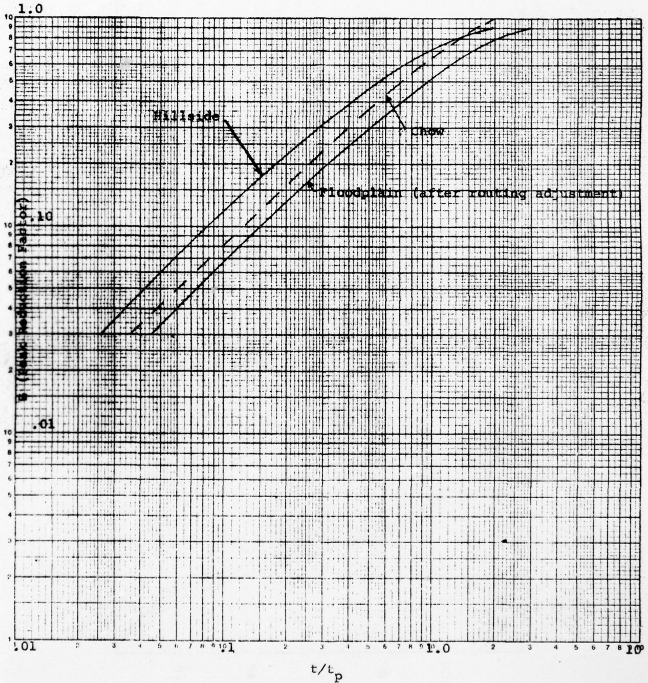
Fig. 23 K versus t/t_p
