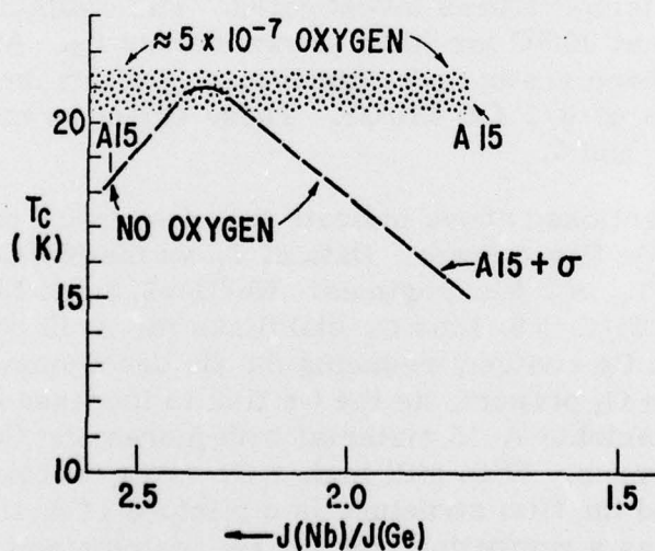
Figure 6. Critical Temperature of Nb 3 Ge PVD Films vs Nb/Ge Flux Ratio With and Without Oxygen. The presence of the oxygen greatly widens the range of flux ratios that yield critical temperatures.
