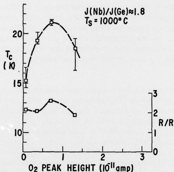
Figure 5. Critical Temperature of Nb 3 Ge PVD Films vs Oxygen Concentration in the Chamber Atmosphere (as measured by mass spectrometry) for a Particular Nb/Ge Flux Ratio
