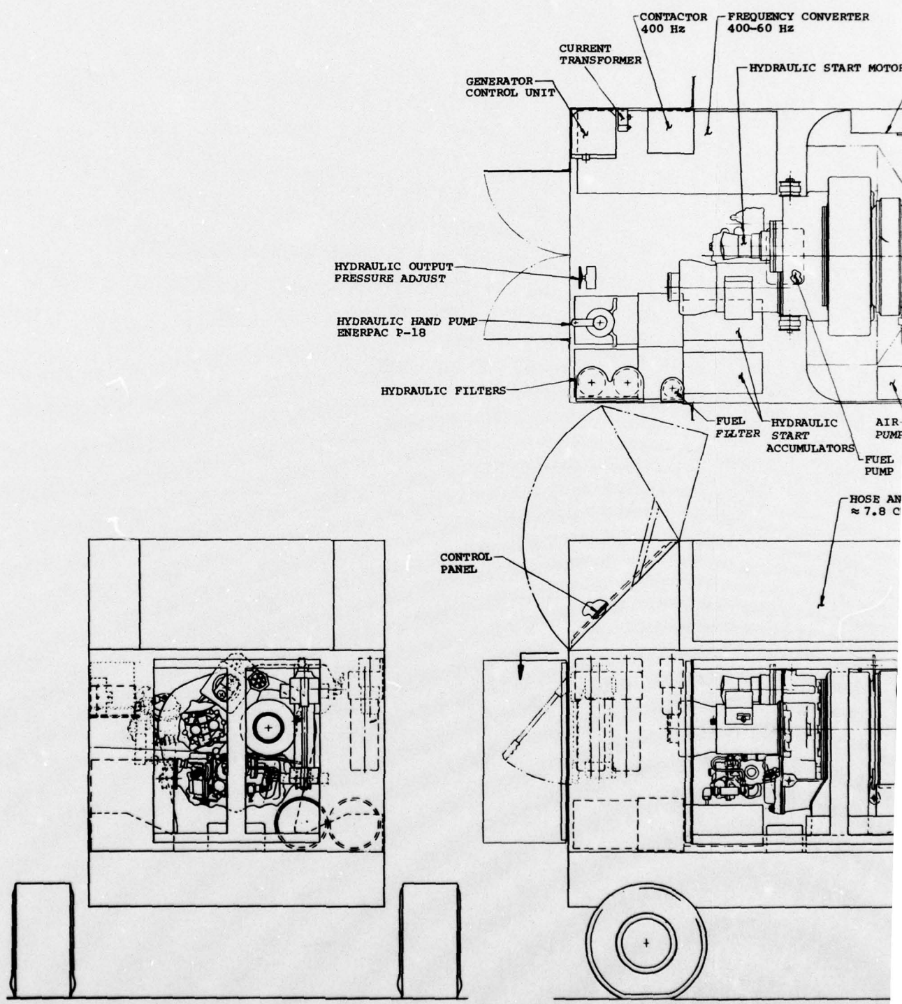
Figure 6. Baseline GPU layout.
