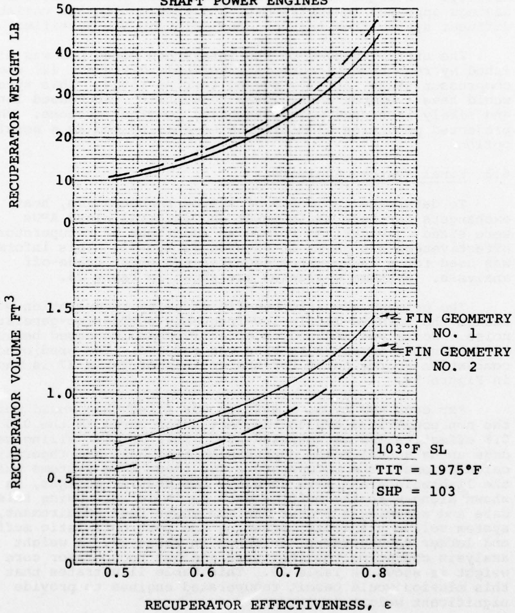
Figure 52. Recuperator sizing study.
