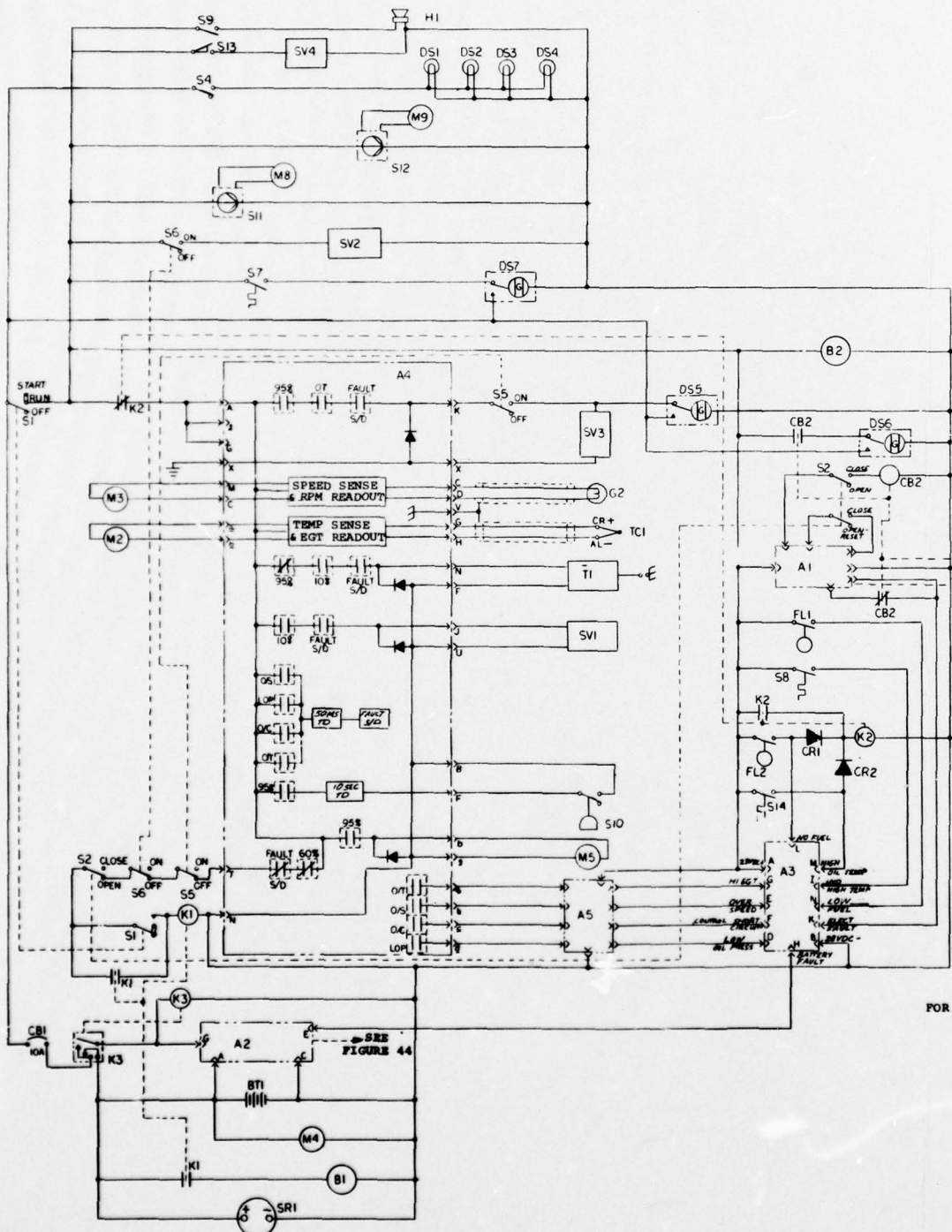
Figure 45. Selected ground power unit, DC circuit wiring schematic.
