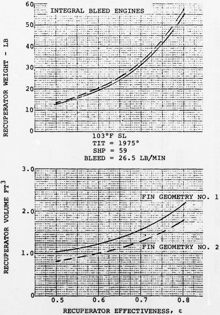
Figure 53. Recuperator sizing study.
