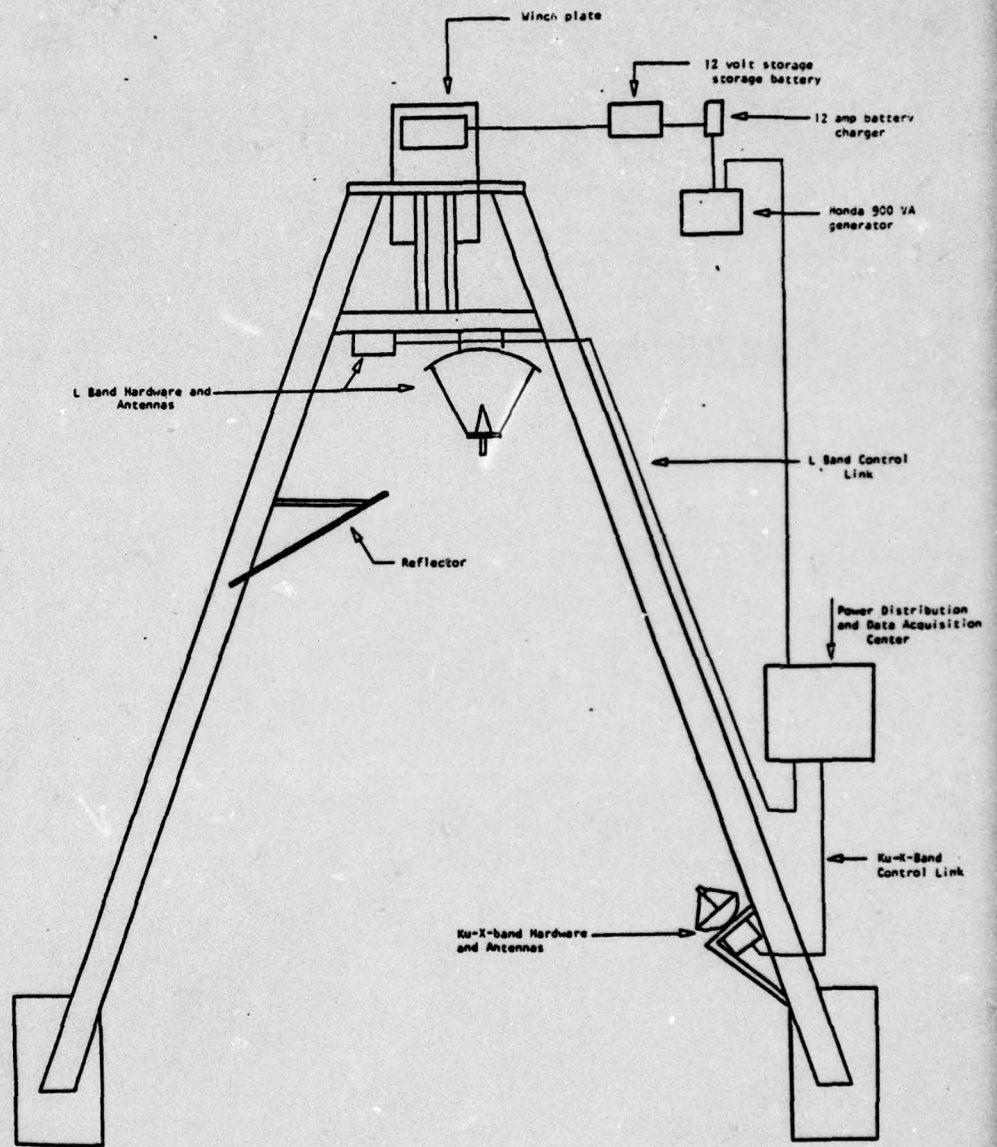
System Configuration
