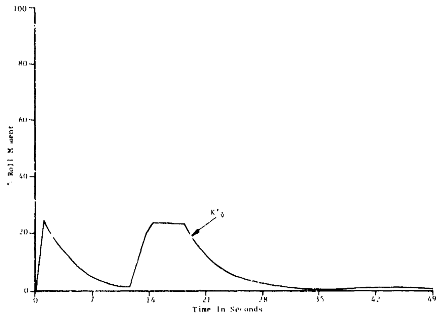
FIGURE 34. PERCENT CONTRIBUTION OF K'_{\psi} TO ROLL MOMENT DURING A \delta_r = \pm 30^\circ TURN REVERSAL MANEUVER
