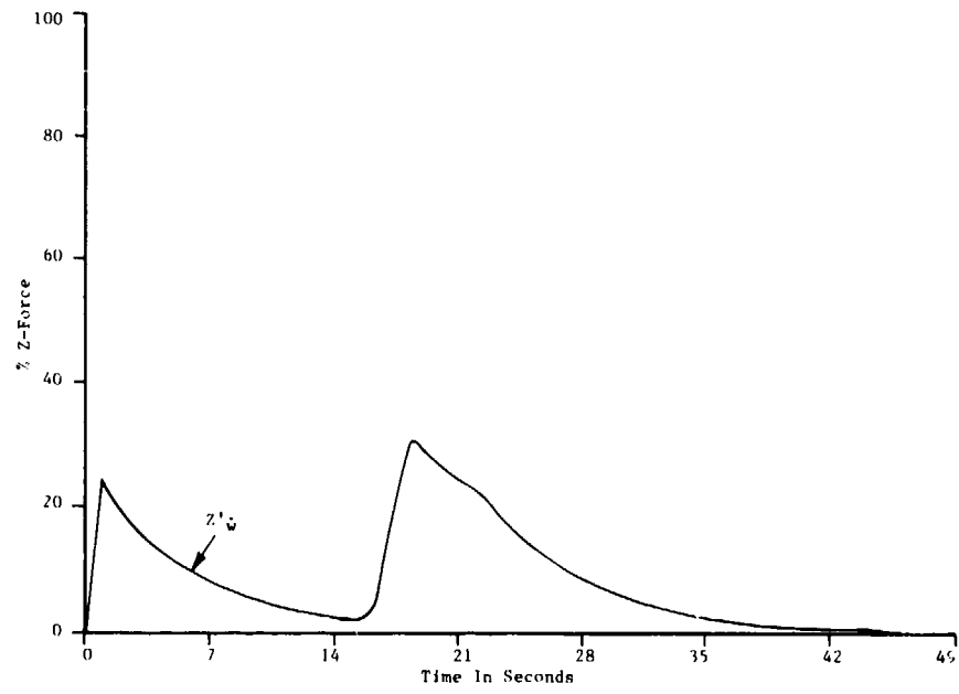
FIGURE 8. PERCENT CONTRIBUTION OF Z'_w TO Z-FORCE DURING A \delta_s = \pm 30^\circ DIVE/CLIMB MANEUVER
