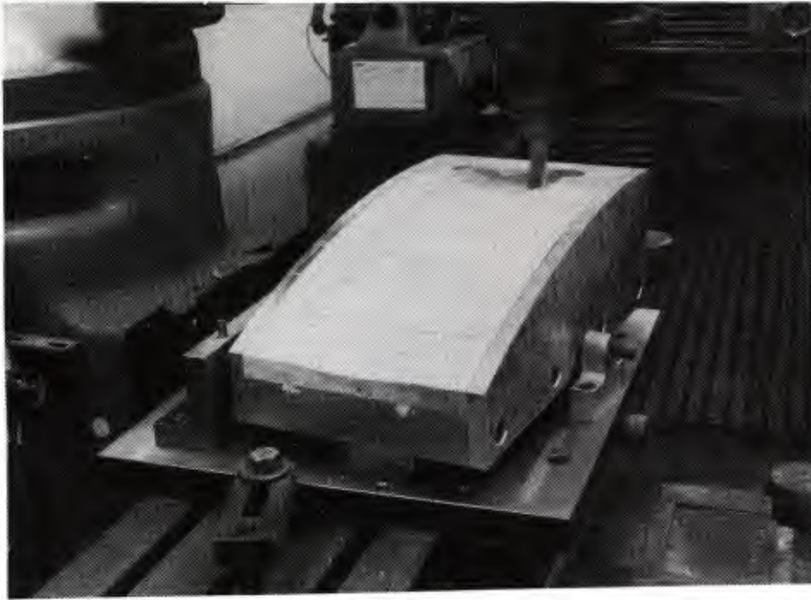
Figure 16. Milling Root Pocket in 4X Plaster Model (#76-5319)
