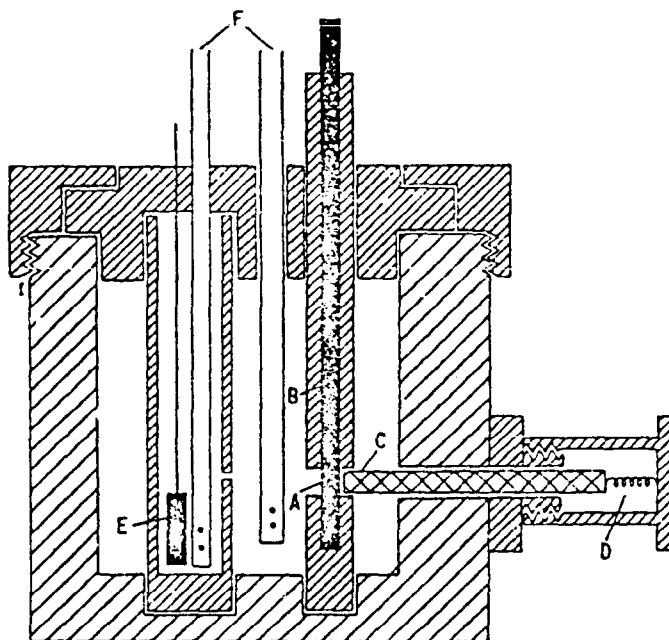
A—cadmium rod B—steel rod C—sapphire rod D—steel spring E—platinized Pt foil attached to Pt wire F—Teflon tubing with closed ends and small holes for gas stirring ■—made of Teflon
