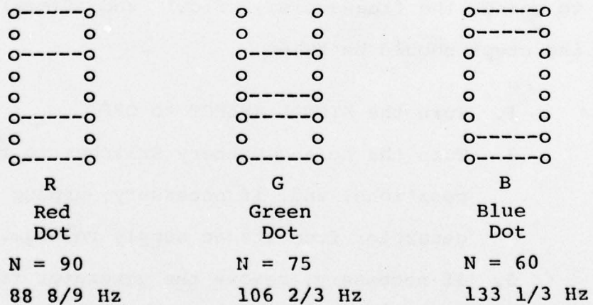
Figure 6. Divisor headers
