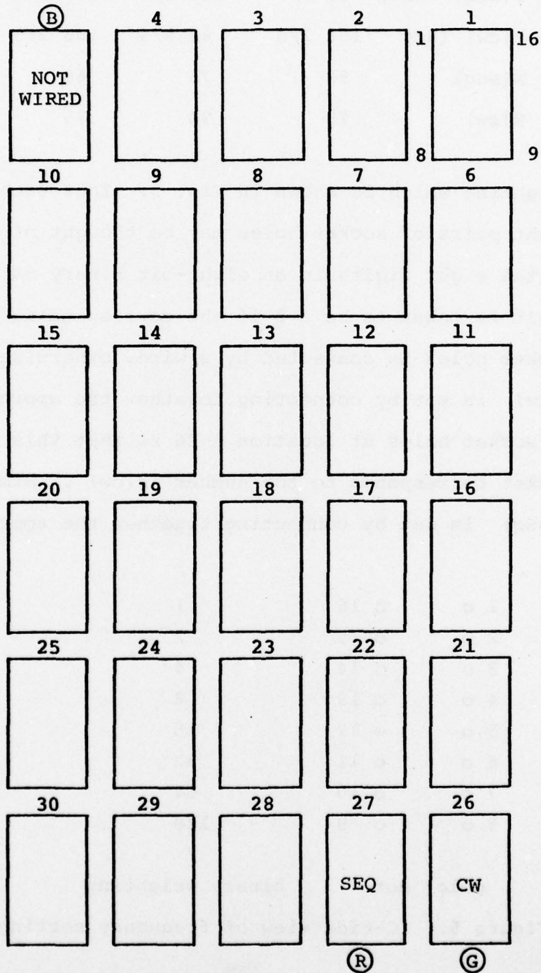
Figure 4. Header locations
