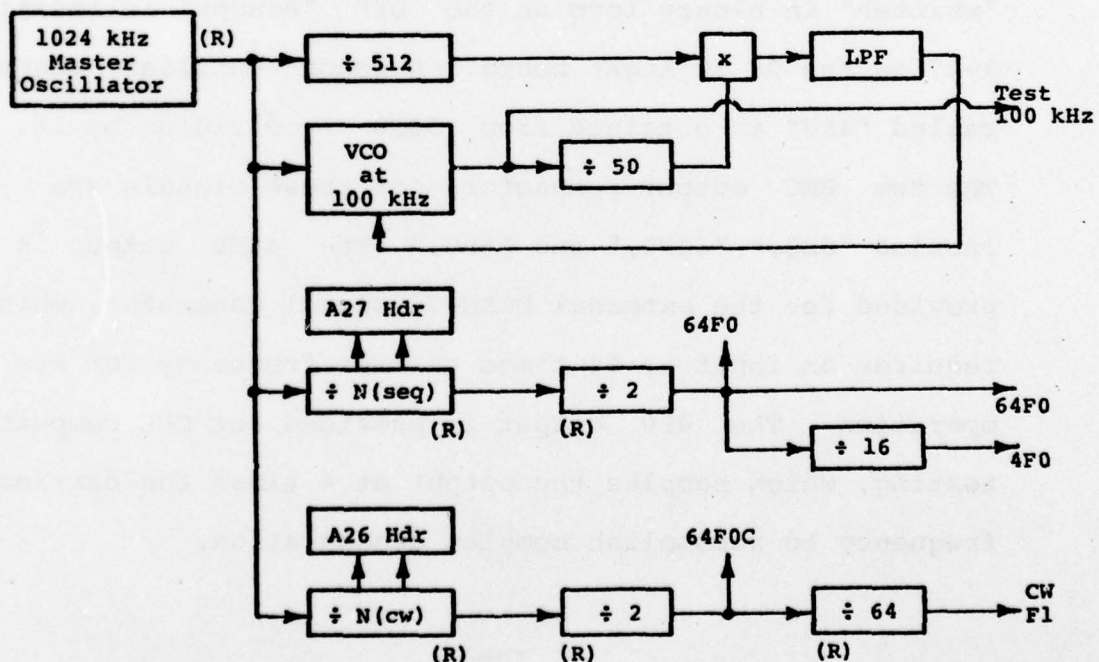
Figure 10. Master oscillator and reference frequencies
