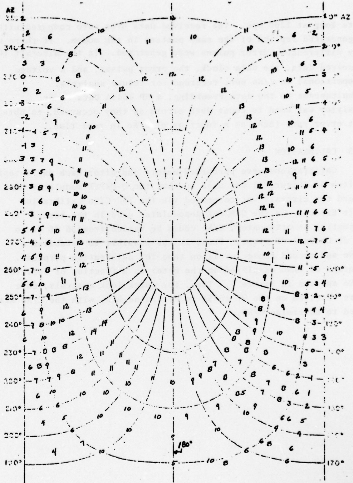
FIGURE 5 SUMMARY OF MEASURED GAIN RESULTS FOR PHASED ARRAY ANTENNA FROM 1975 AND 1976 TESTS
