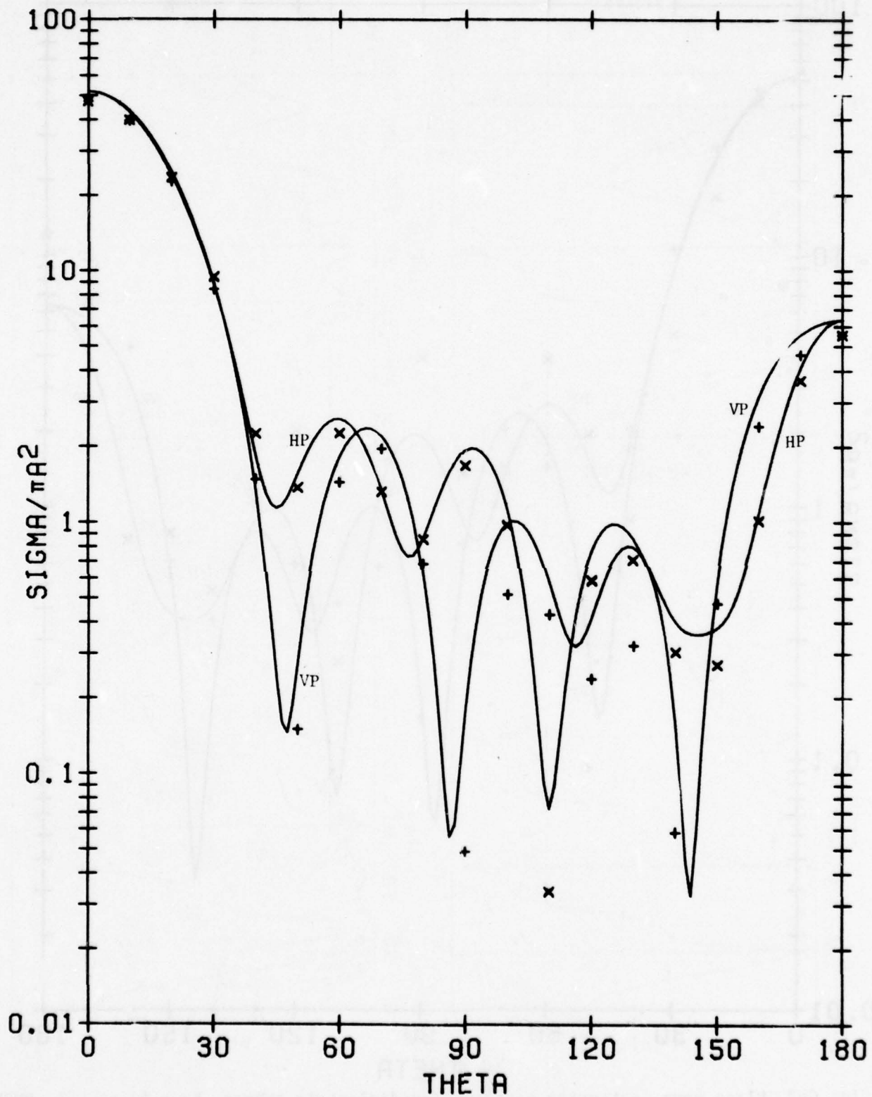
Fig. C-8. Plane wave scattering patterns for dielectric sphere, ka = 5 , r = 4 , Müller solution. Symbols \times and + denote horizontal polarization and vertical polarization respectively. Solid line denotes exact solution.
