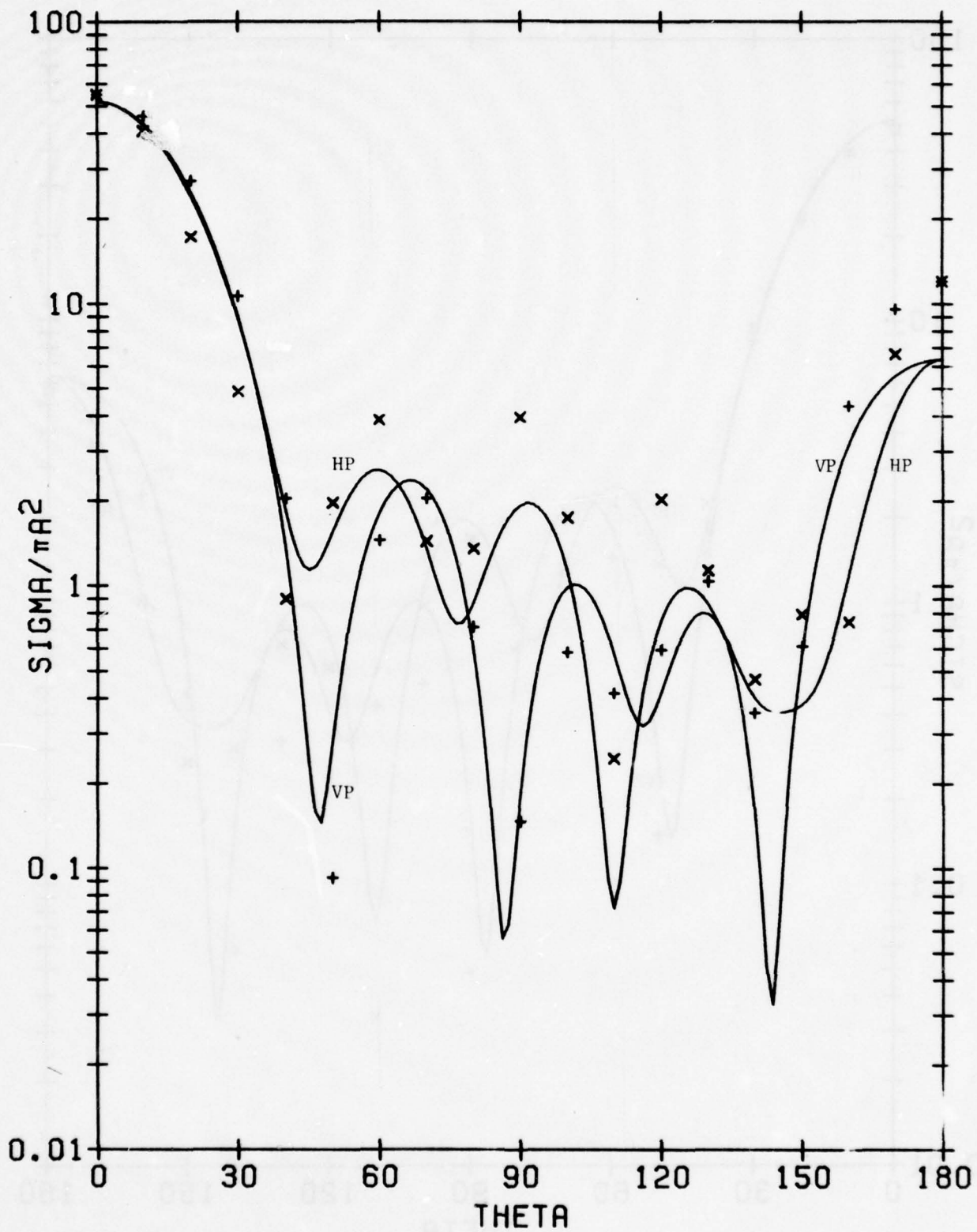
Fig. C-7. Plane wave scattering patterns for dielectric sphere, ka = 5 , \epsilon_r = 4 , PMCHW solution. Symbols \times and + denote horizontal polarization and vertical polarization respectively. Solid line denotes exact solution.
