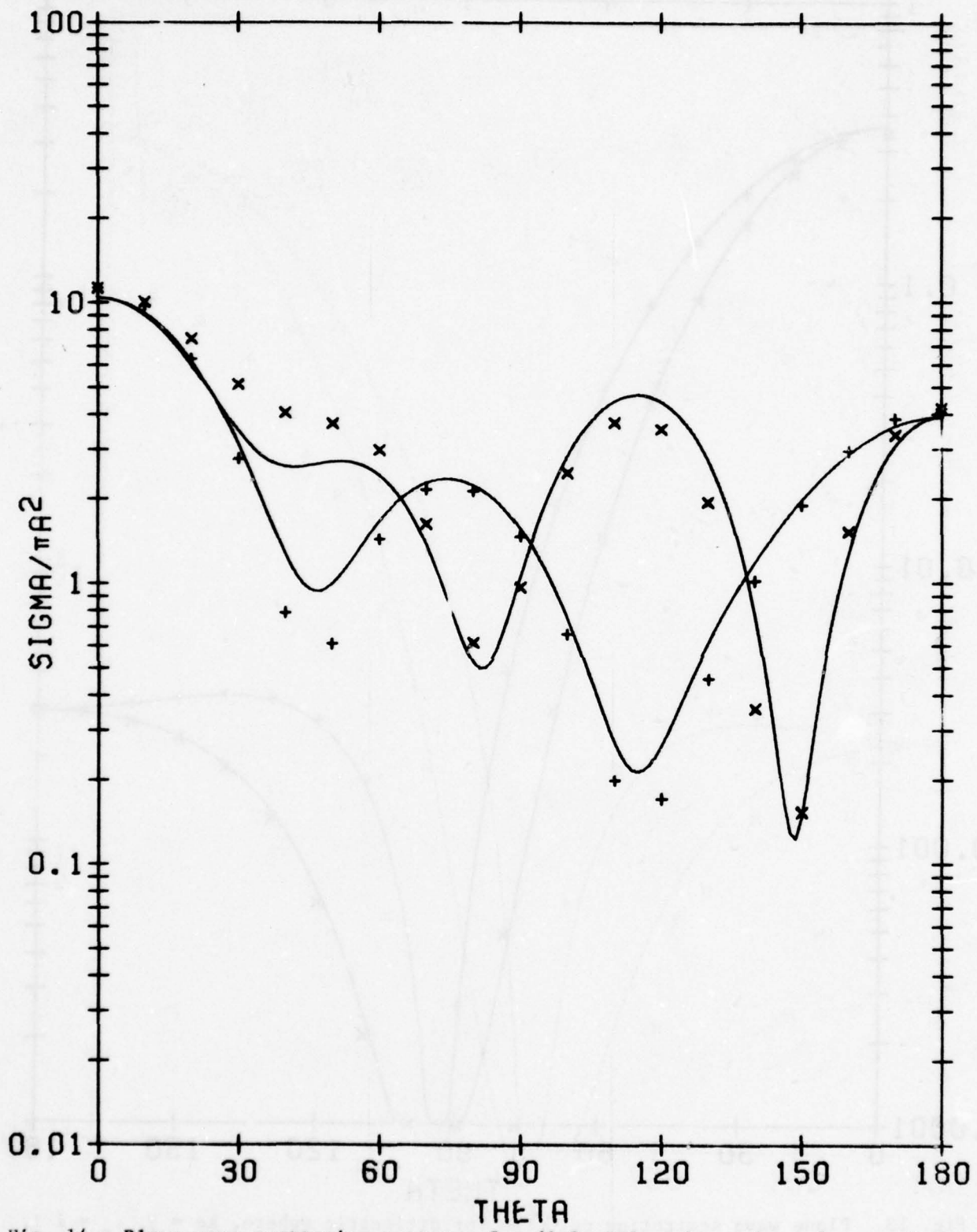
Fig. 14. Plane wave scattering patterns for dielectric sphere \epsilon , ka = 3 , \epsilon_r = 1 , PMCHW solution. Symbols \times and + denote horizontal polarization and vertical polarization respectively. Solid line denotes exact solution.
