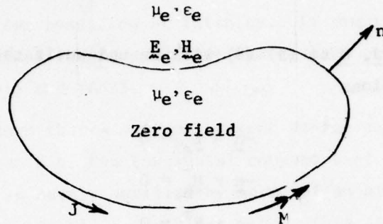
Fig. B-1. Radiation of \underline{J}, \underline{M} according to (B-1) and (B-2).
