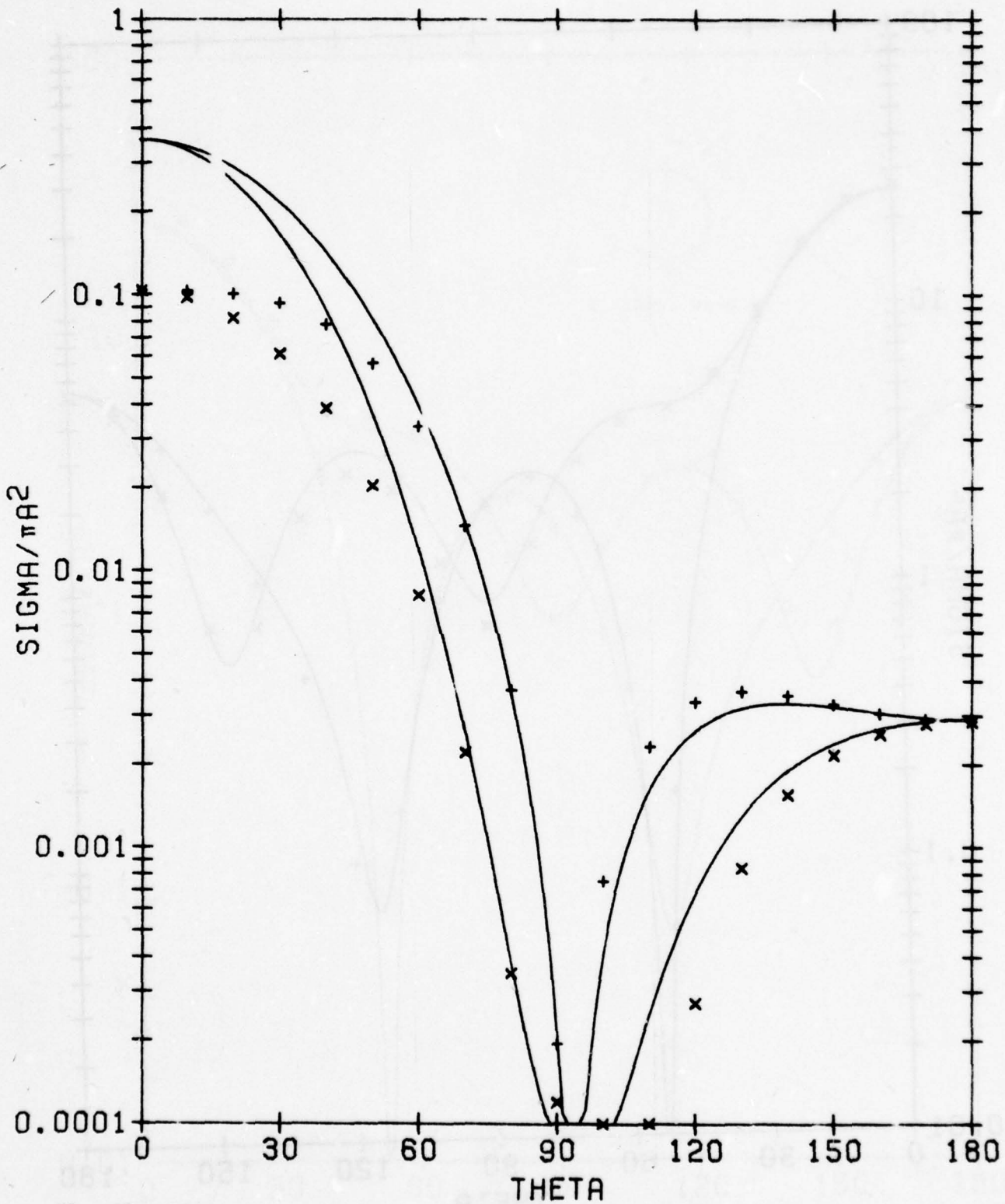
Fig. 12. Plane wave scattering patterns for dielectric sphere, ka = 3 , \epsilon_r = 1.1 , PMCHW solution. Symbols \times and + denote horizontal polarization r and vertical polarization respectively. Solid line denotes exact solution.
