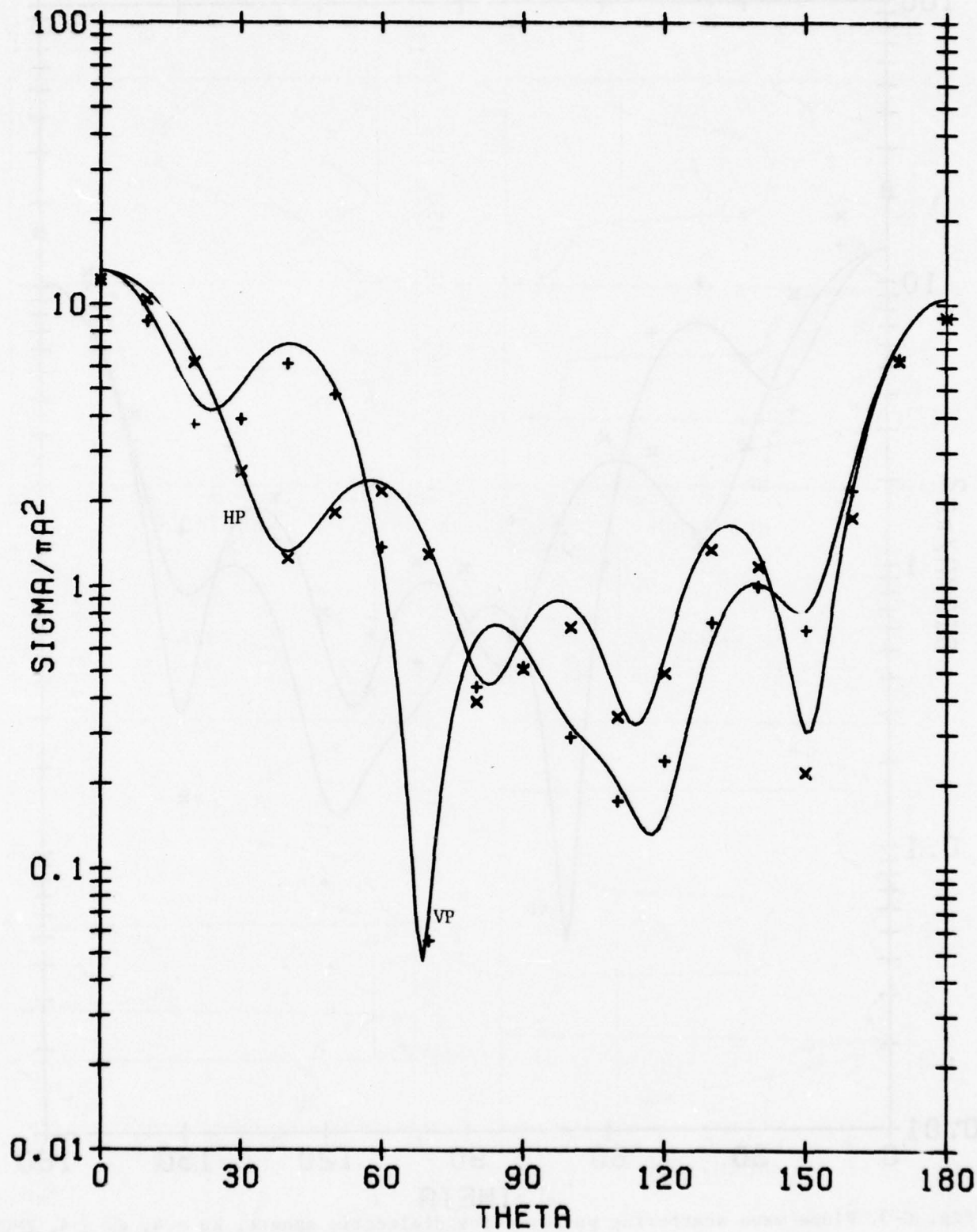
Fig. C-4. Plane wave scattering patterns for dielectric sphere, ka = 1 , \epsilon_r = 4 , Müller solution. Symbols \times and + denote horizontal polarization and vertical polarization respectively. Solid line denotes exact solution.
