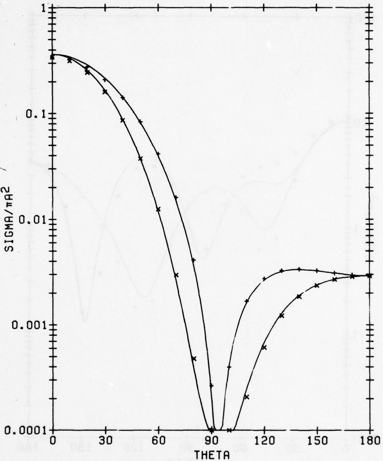
Fig. 13. Plane wave scattering patterns for dielectric sphere, ka = 3 , \epsilon_r = 11 , Müller solution. Symbols \times and + denote horizontal polarization and vertical polarization respectively. Solid line denotes exact solution.
