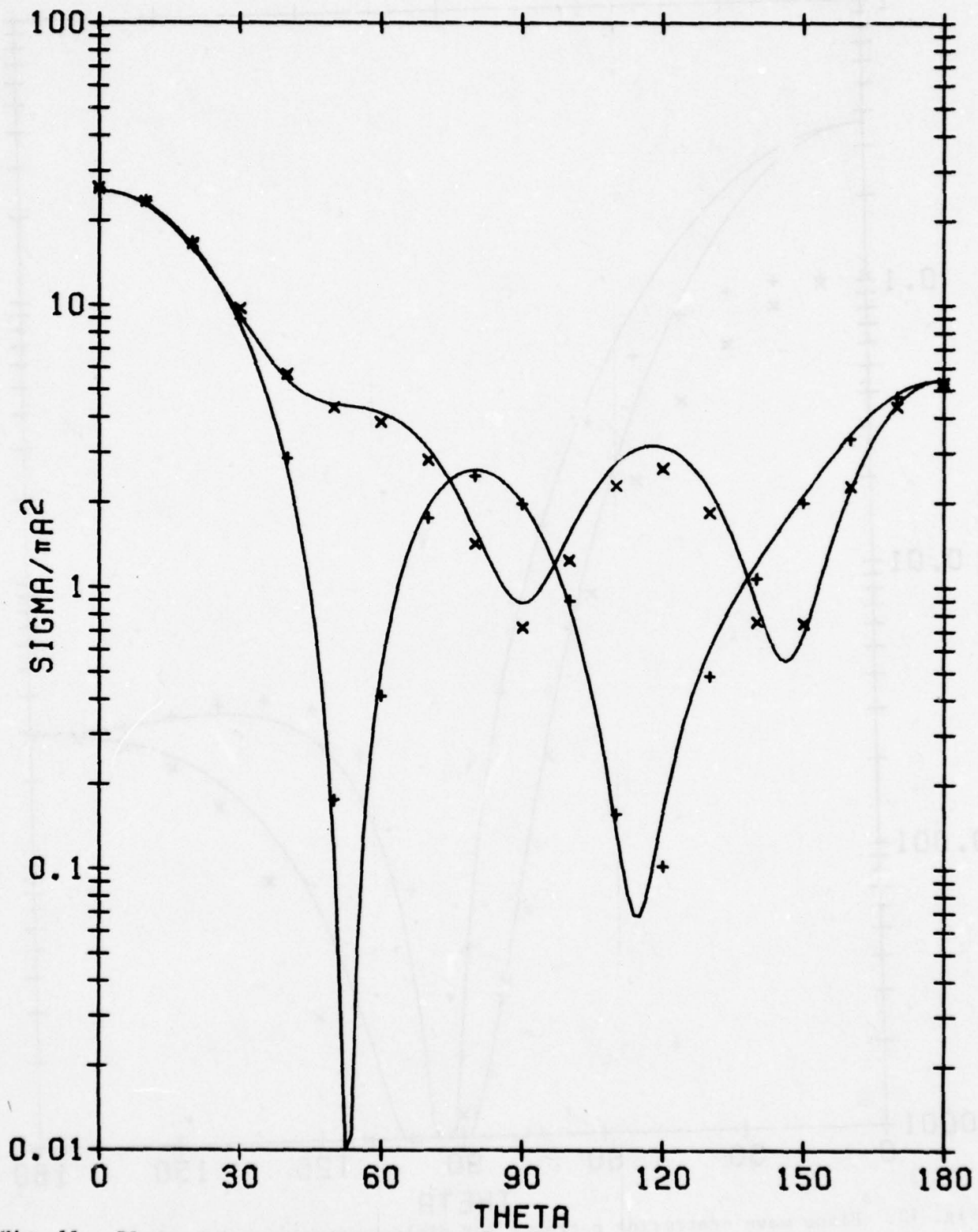
Fig. 11. Plane wave scattering patterns for dielectric sphere, k_1 = 3 , \epsilon = 4 , Müller solution. Symbols \wedge and + denote horizontal polarization and vertical polarization respectively. Solid line denotes exact solution.
