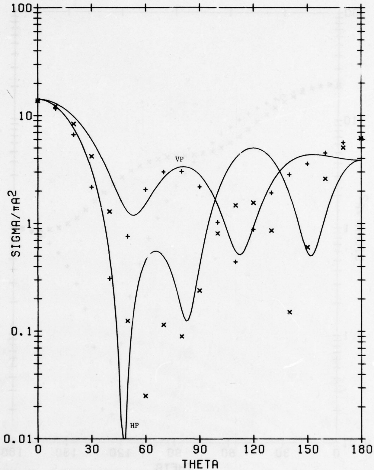
Fig. 17. Plane wave scattering patterns for dielectric sphere, ka = 1 , \epsilon_r = 20 , Müller solution. Symbol: \times and + denote horizontal polarization and vertical polarization respectively. Solid line denotes exact solution.
