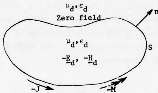
Fig. B-2. Radiation of -\underline{J}, -\underline{M} according to (B-3) and (B-4).
