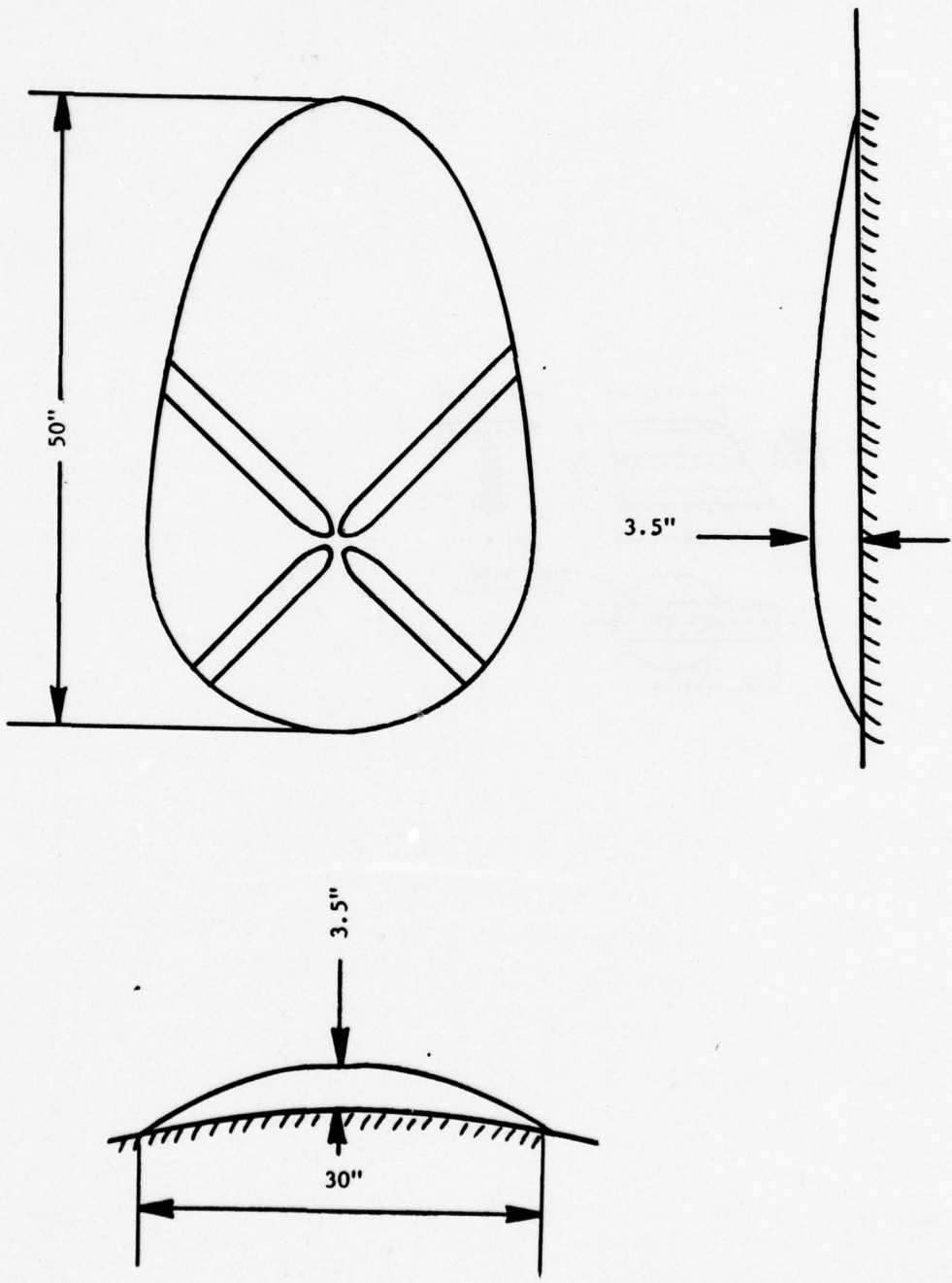
FIGURE 11.2 BOEING CROSSED LOOP ANTENNA
