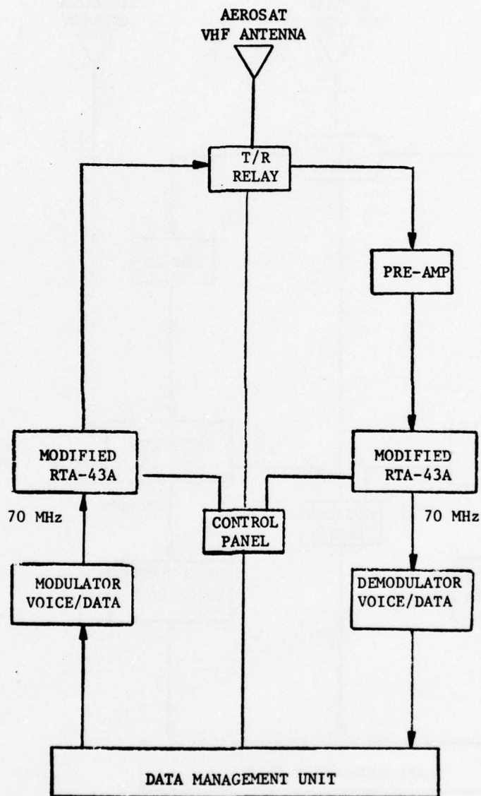
FIGURE 4.1. AEROSAT VHF TEST AVIONICS TYPE I SYSTEM (CONFIGURATION #1) HALF-DUPLEX WITHOUT TERRESTRIAL COMMUNICATION CAPABILITY
