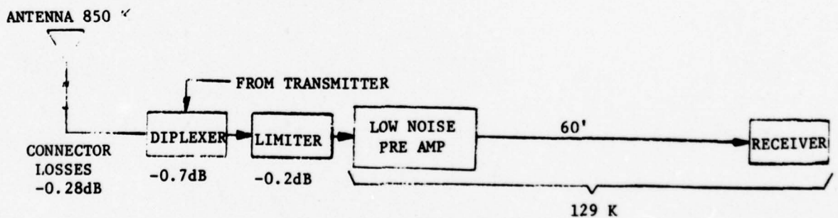
(c) LOW NOISE PRE-AMP AT ANTENNA
