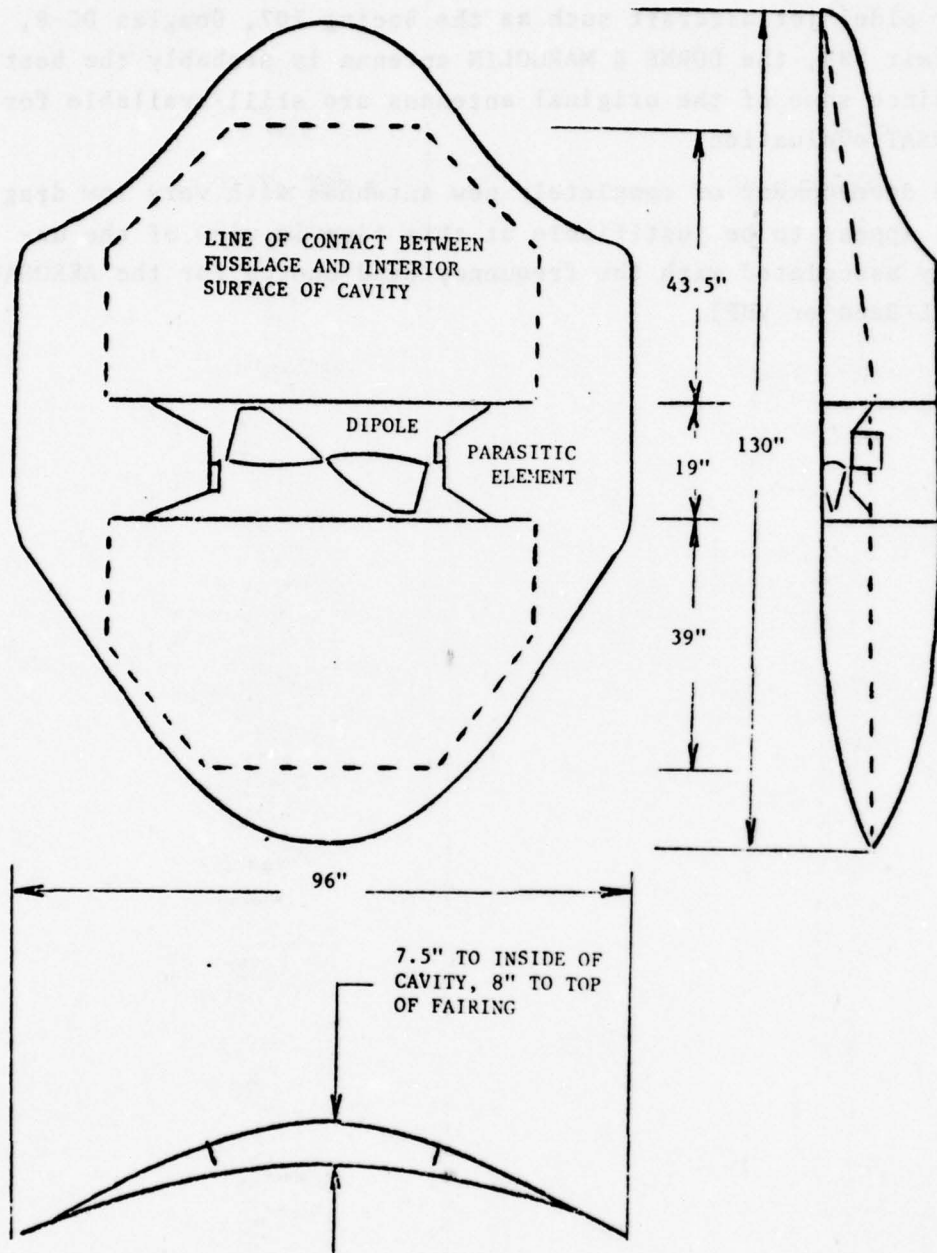
FIGURE 11.1. BOEING 747 SLOT DIPOLE ANTENNA COPY OF BOEING SKETCH
