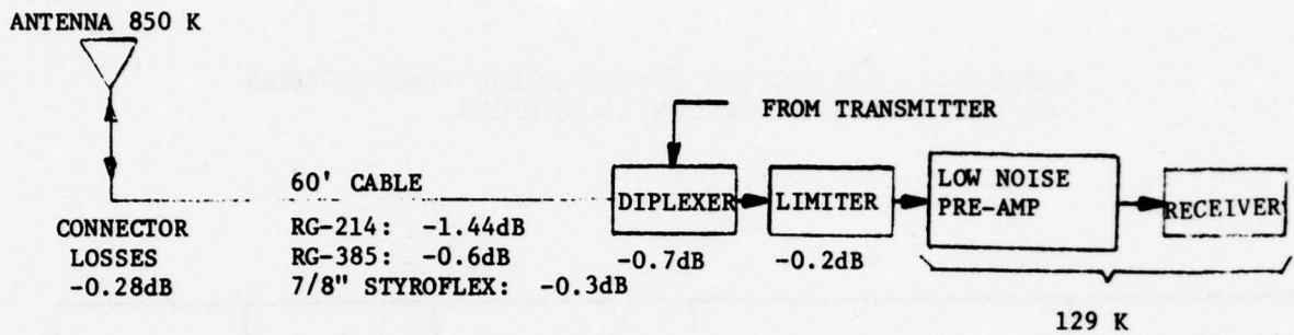
(a) LOW NOISE PRE-AMP IN RECEIVER
