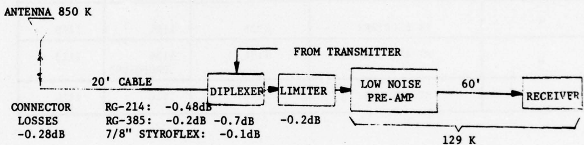
(b) LOW NOISE PRE-AMP AT AFT BULKHEAD (PROPOSED)
