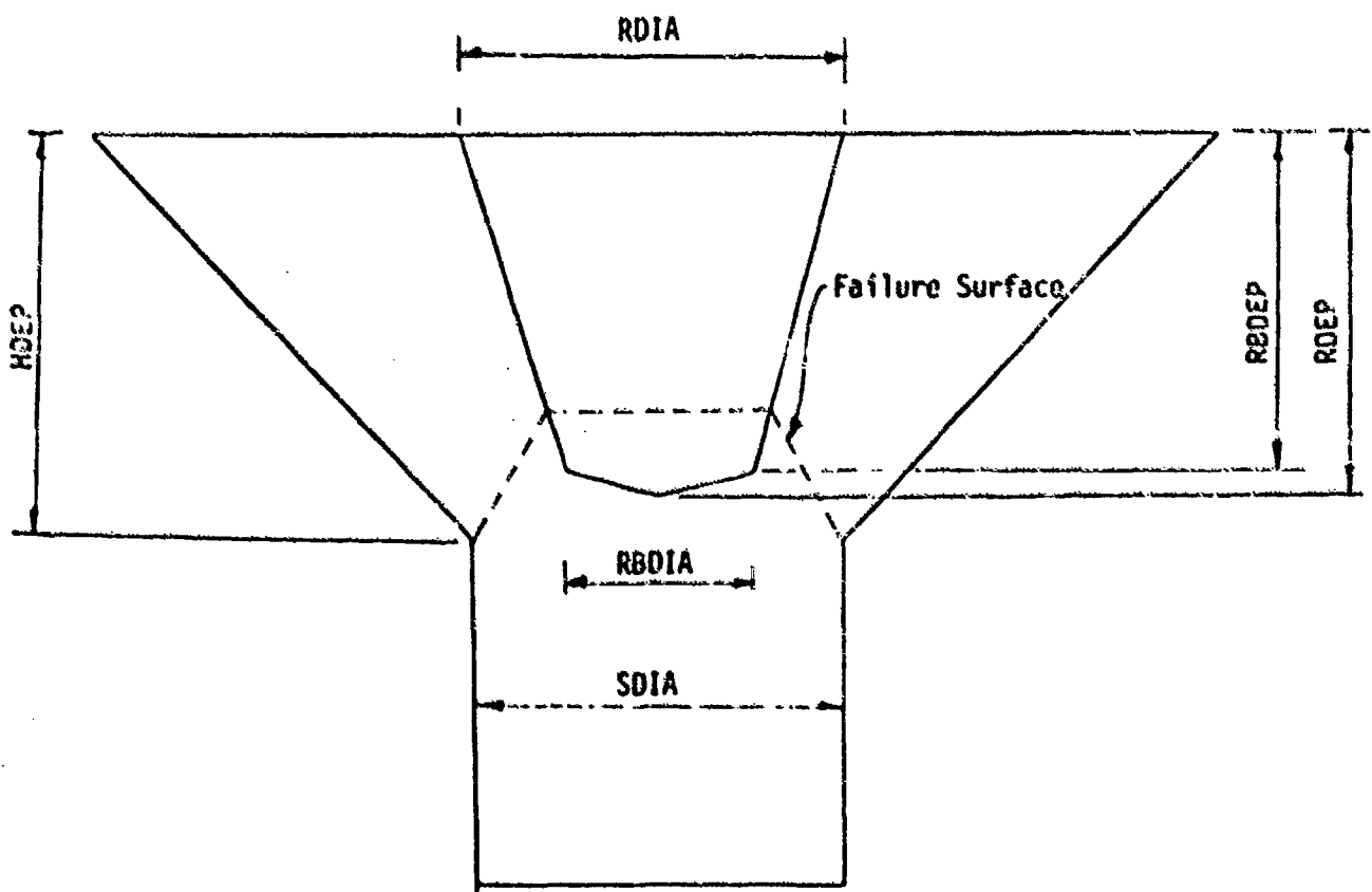
Figure 83 - Idealized Recess
