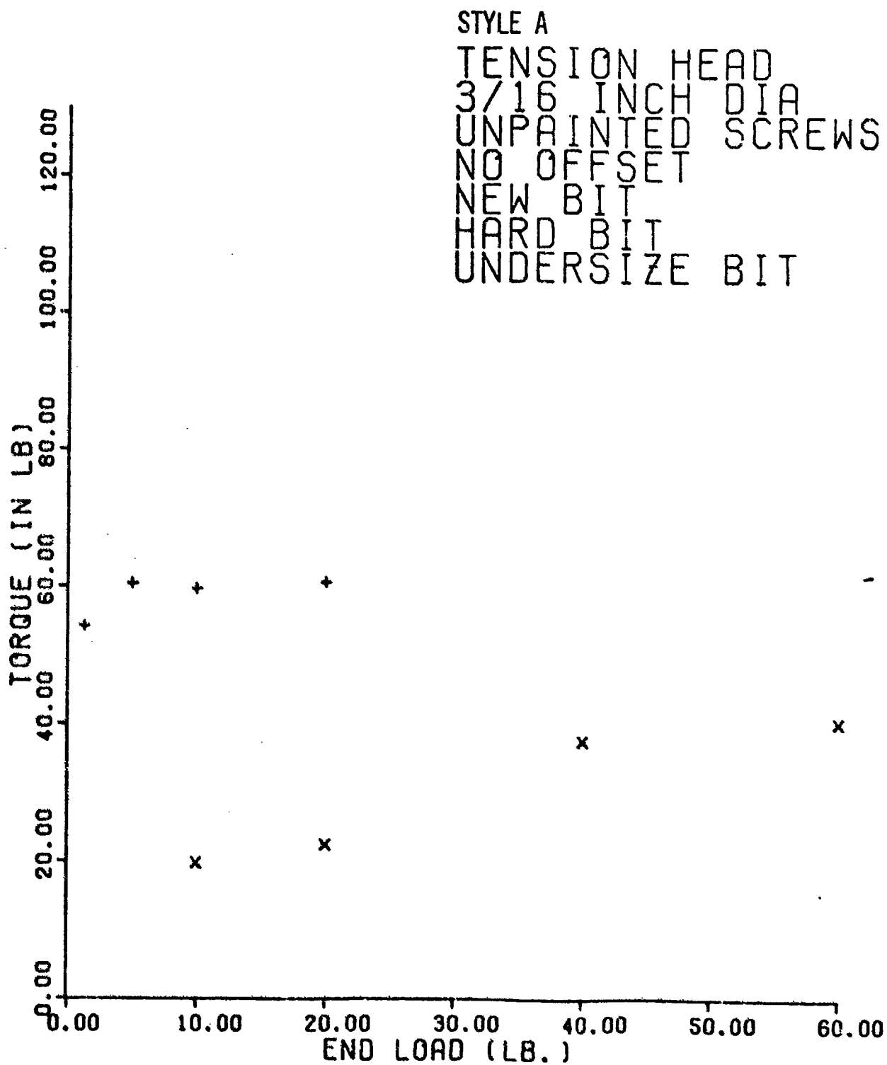
Figure 7. Style A Tests Results
