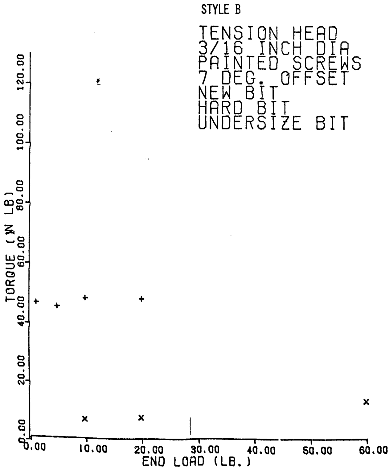
Figure 30. Style B Test Results
