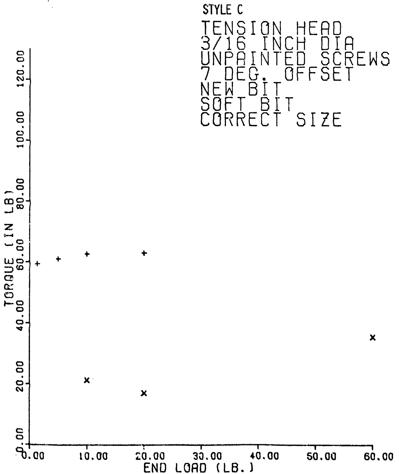
Figure 38. Style C Test Results
