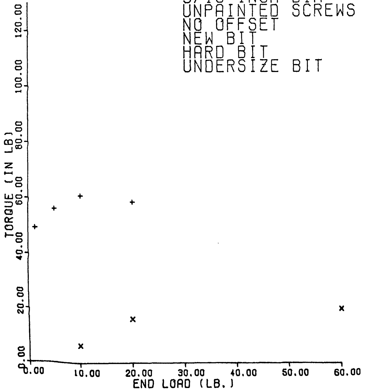
Figure 47. Style D Test Results
