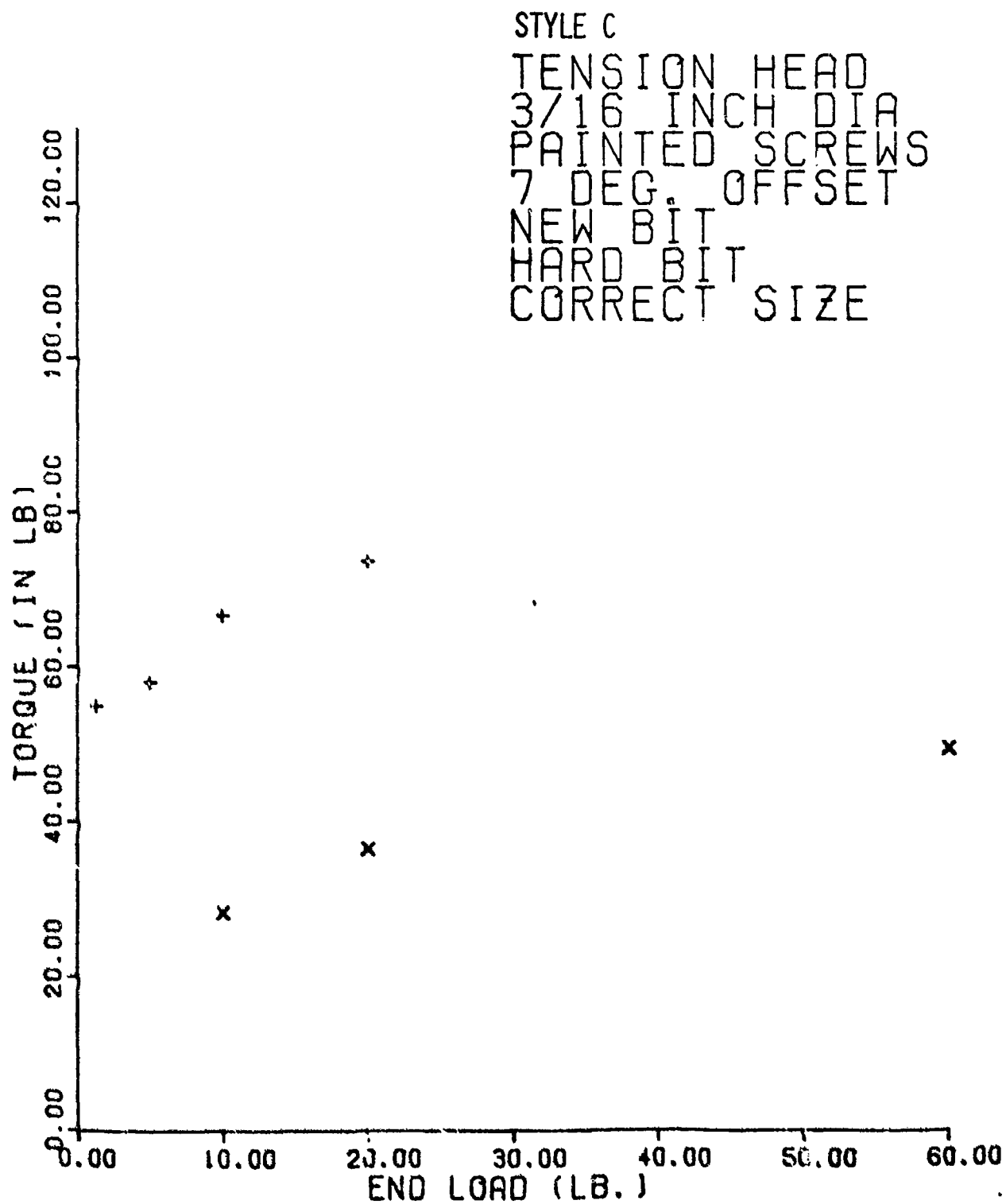
Figure 40. Style C Test Results
