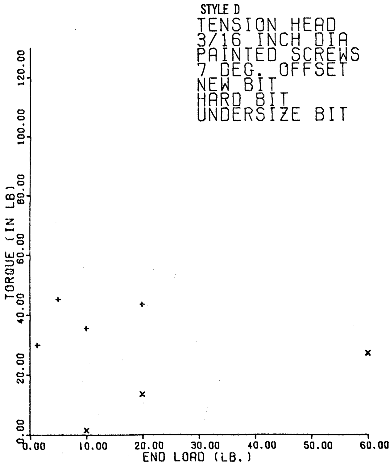
Figure 54. Style D Test Results
