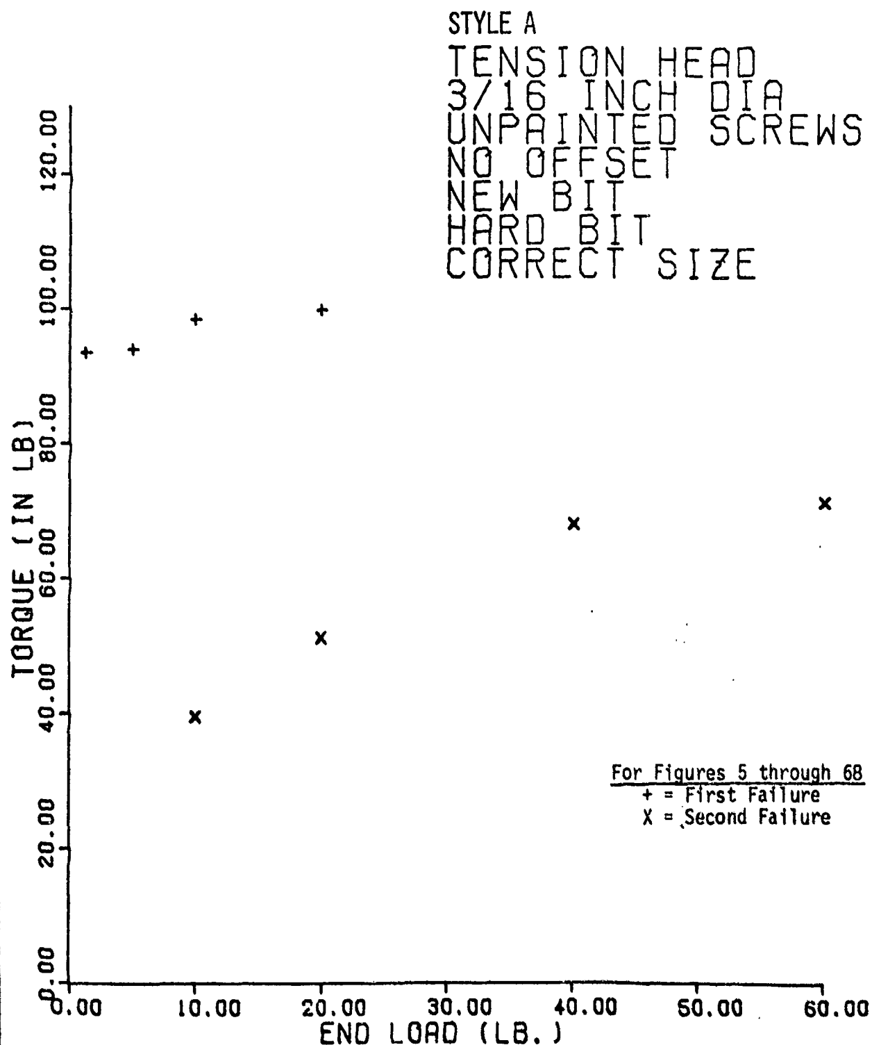
Figure 5. Style A Test Results
