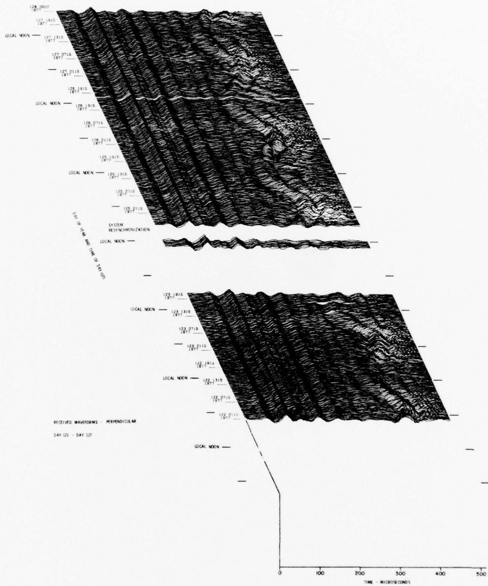
Figure 3. VLF/LF Reflectivity Data for the Polar Ionosphere, DAY 121 (1 May) - DAY 127 (7 May) 1977 (Cont) Part S. \perp Waveform Display
