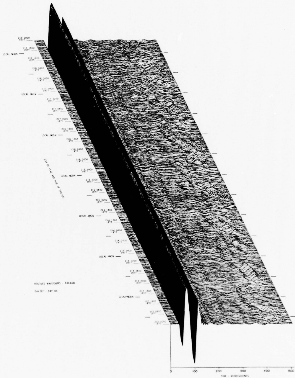
Figure 16. VLF/LF Reflectivity Data for the Polar Ionosphere, DAY 212 (31 Jul) - DAY 218 (6 Aug) 1977 (Cont) Part R. ¶ Waveform Display
