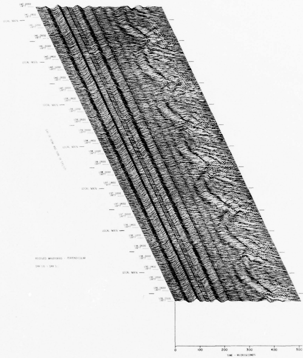
Figure 5. VLF/LF Reflectivity Data for the Polar Ionosphere, DAY 135 (15 May) - DAY 141 (21 May) 1977 (Cont) Part S. \perp Waveform Display
