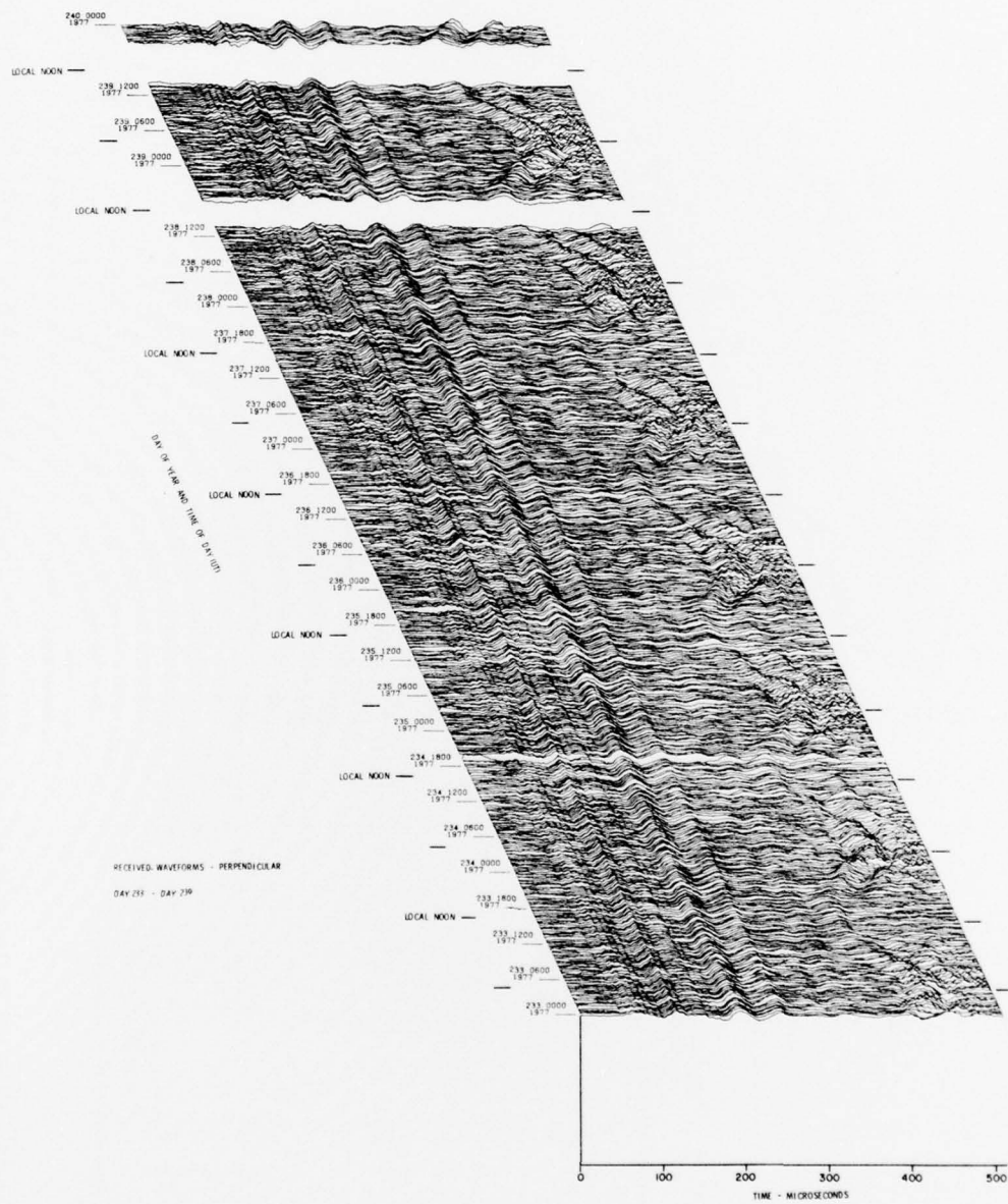
Figure 19. VLF/LF Reflectivity Data for the Polar Ionosphere, DAY 233 (21 Aug) - DAY 239 (27 Aug) 1977 (Cont) Part S. \perp Waveform Display
