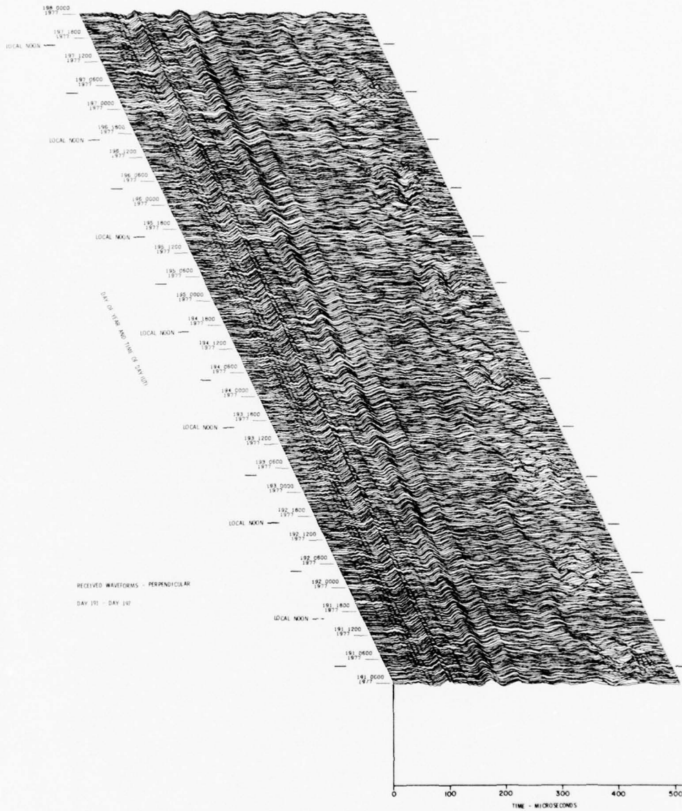
Figure 13. VLF/LF Reflectivity Data for the Polar Ionosphere, DAY 191 (10 Jul) - DAY 197 (16 Jul) 1977 (Cont) Part S. \perp Waveform Display
