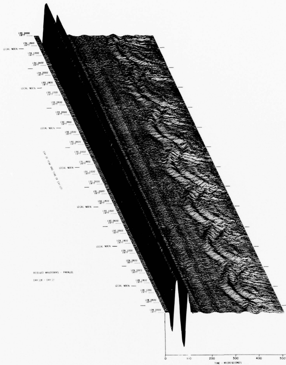
Figure 4. VLF/LF Reflectivity Data for the Polar Ionosphere, DAY 128 (8 May) - DAY 134 (14 May) 1977 (Cont) Part R. || Waveform Display
