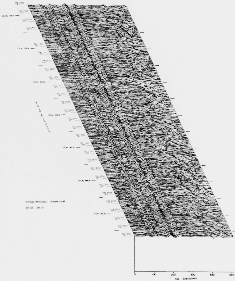
Figure 17. VLF/LF Reflectivity Data for the Polar Ionosphere, DAY 219 (7 Aug) - DAY 225 (13 Aug) 1977 (Cont) Part S. \perp Waveform Display
