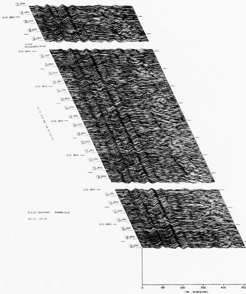
Figure 10. VLF/LF Reflectivity Data for the Polar Ionosphere, DAY 170 (19 Jun) - DAY 176 (25 Jun) 1977 (Cont) Part S. ↓ Waveform Display
