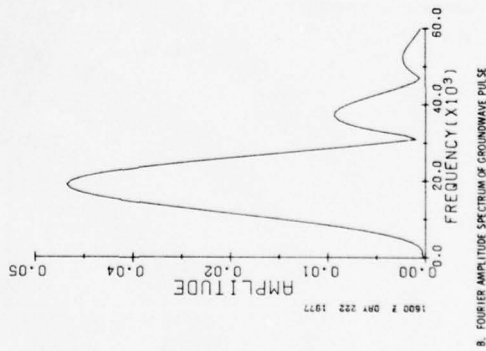
A. RECEIVED WAVEFORMS - 1800GMT, DAY 222
