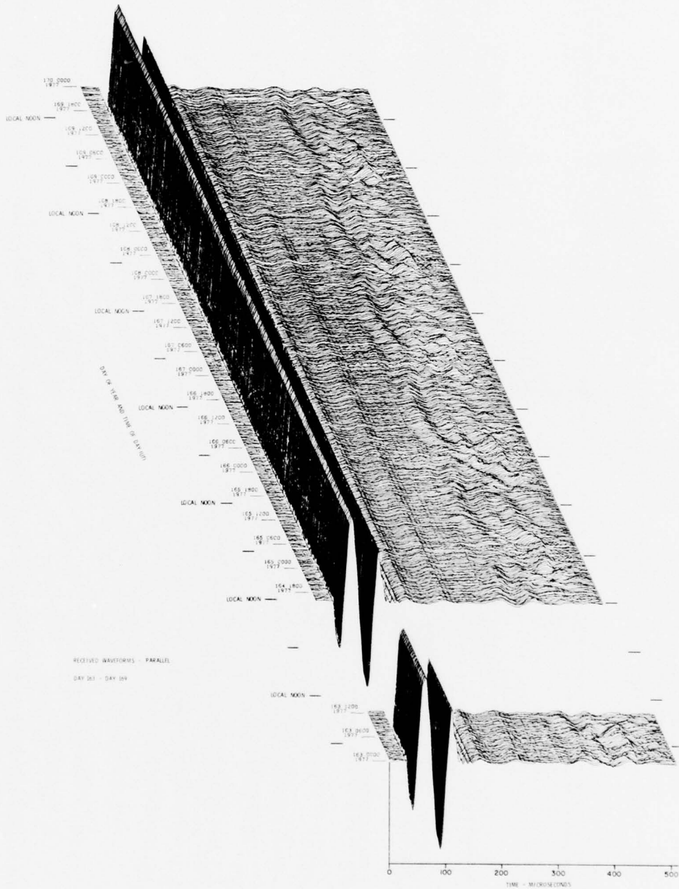
Figure 9. VLF/LF Reflectivity Data for the Polar Ionosphere, DAY 163 (12 Jun) - DAY 169 (18 Jun) 1977 (Cont) Part R. II Waveform Display
