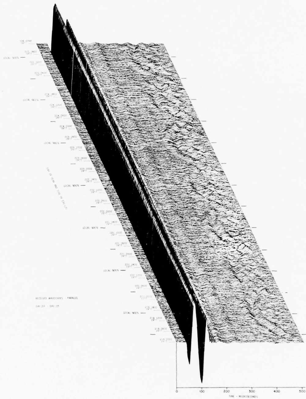
Figure 17. VLF/LF Reflectivity Data for the Polar Ionosphere, DAY 219 (7 Aug) - DAY 225 (13 Aug) 1977 (Cont) Part R. // Waveform Display
