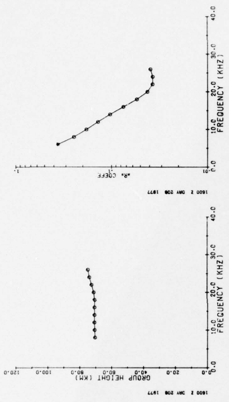
C. GROUP MIRROR REFLECTION HEIGHTS AND ASSOCIATED \mu_{R1} REFLECTION COEFFICIENTS FROM PARALLEL SKYWAVE DATA
