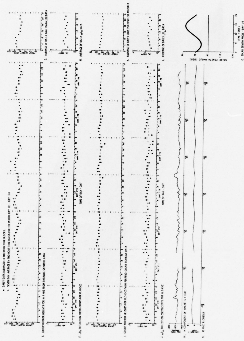
Figure 10. VLF/LF Reflectivity Data for the Polar Ionosphere, DAY 170 (19 Jun) - DAY 176 (25 Jun) 1977 (Cont)
