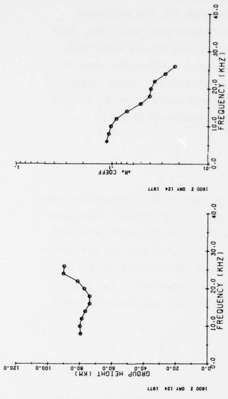
C. GROUP MIRROR REFLECTION HEIGHTS AND ASSOCIATED R_p REFLECTION COEFFICIENTS FROM PARALLEL SKYWAVE DATA
