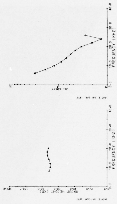
D. GROUP MIRROR REFLECTION HEIGHTS AND ASSOCIATED \mu_{R1} REFLECTION COEFFICIENTS FROM PERPENDICULAR SKYWAVE DATA
