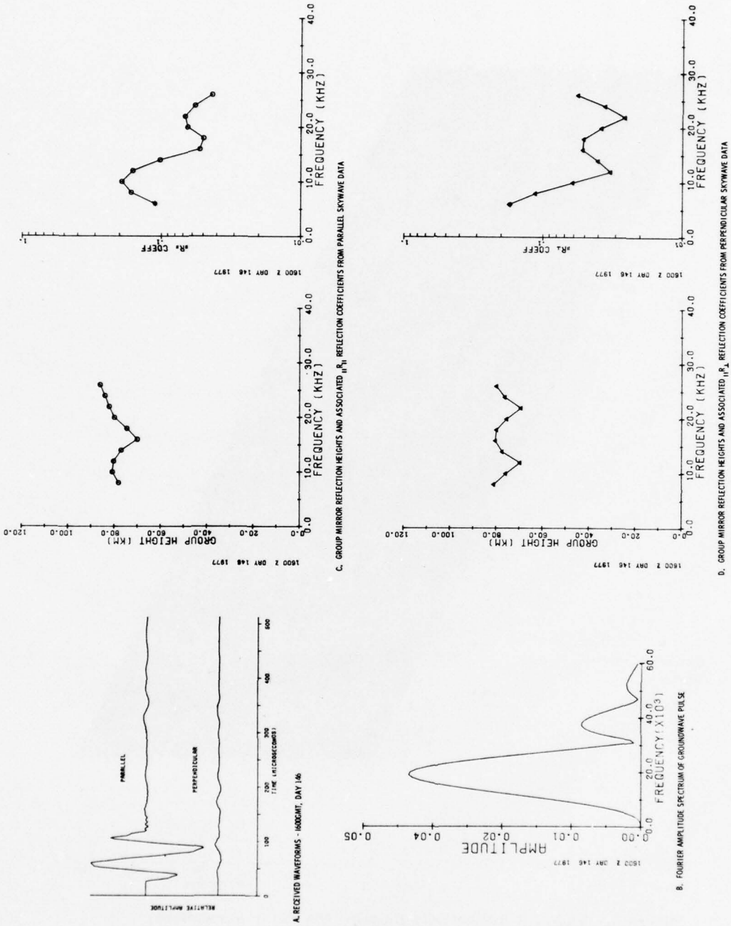
Figure 6. VLF/LF Reflectivity Data for the Polar Ionosphere, DAY 142 (22 May) - DAY 148 (28 May) 1977
