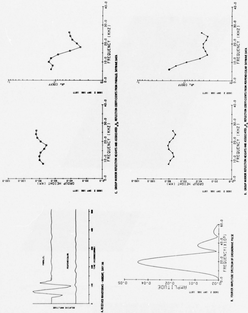
Figure 9. VLF/LF Reflectivity Data for the Polar Ionosphere, DAY 163 (12 Jun) - DAY 169 (18 Jun) 1977
