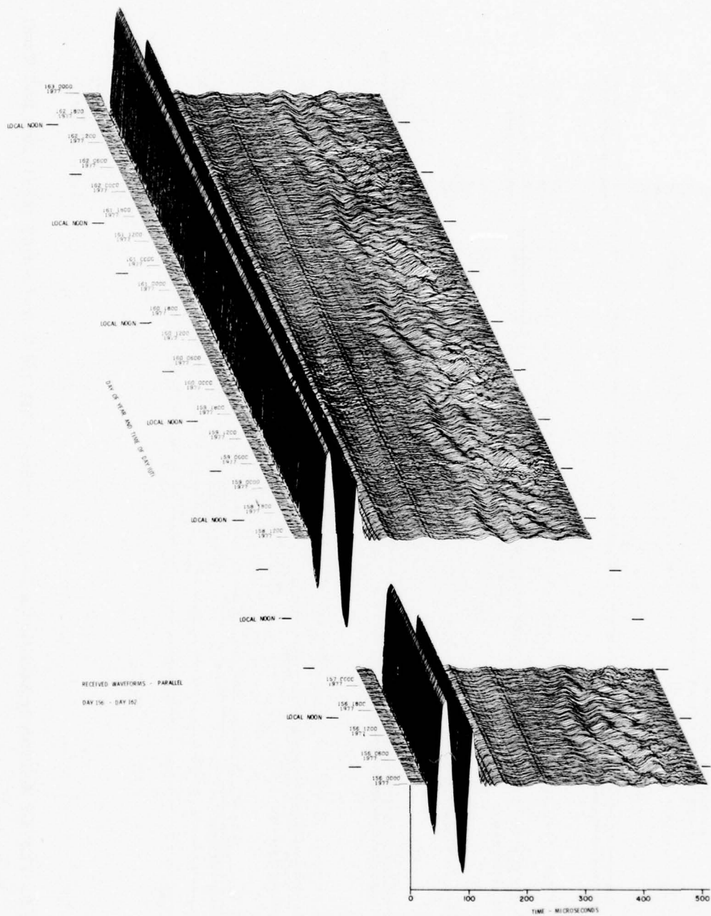
Figure 8. VLF/LF Reflectivity Data for the Polar Ionosphere, DAY 156 (5 Jun) - DAY 162 (11 Jun) 1977 (Cont) Part R. II Waveform Display
