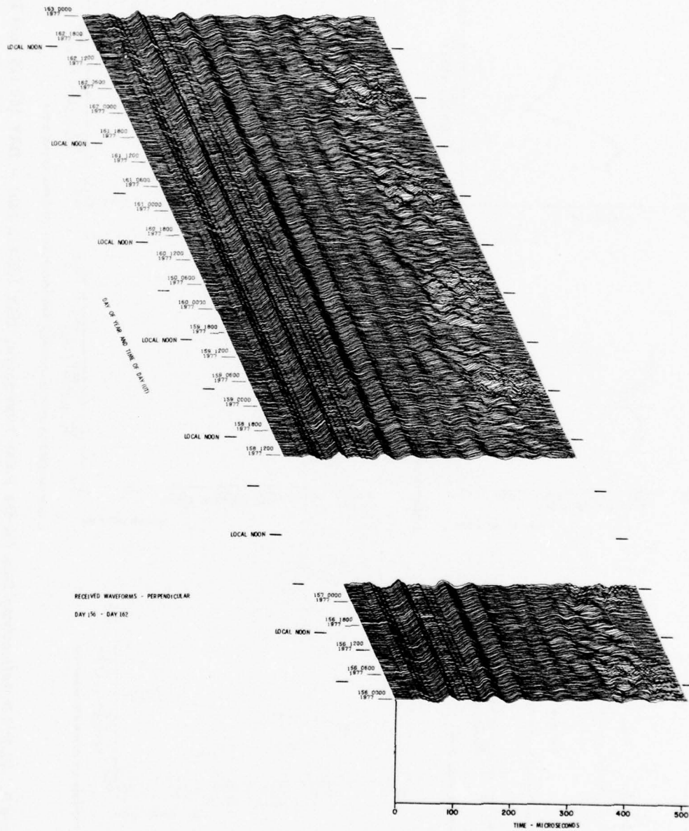
Figure 8. VLF/LF Reflectivity Data for the Polar Ionosphere, DAY 156 (5 Jun) - DAY 162 (11 Jun) 1977 (Cont) Part S. ↓ Waveform Display
