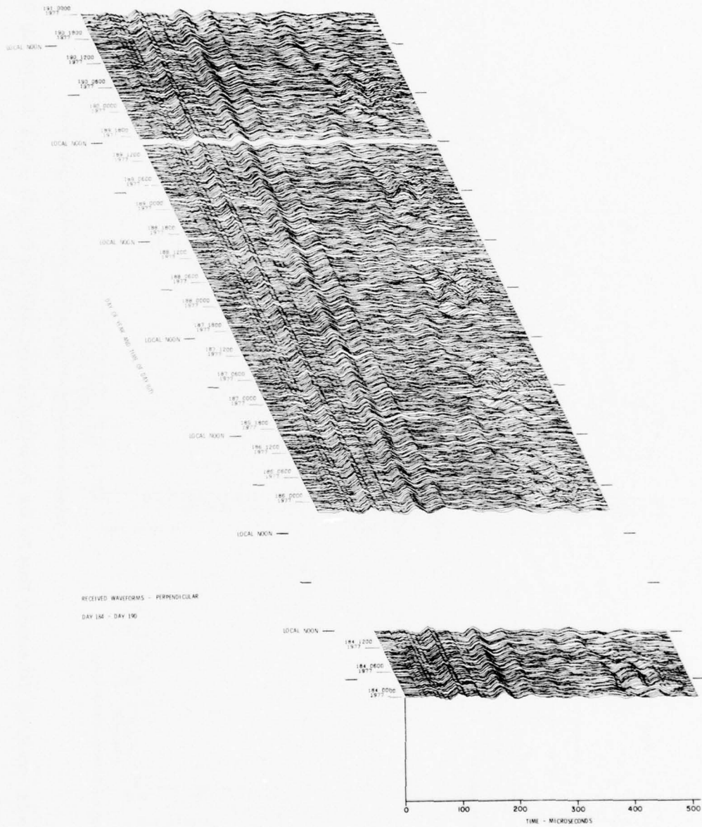
Figure 12. VLF/LF Reflectivity Data for the Polar Ionosphere, DAY 184 (3 Jul) - DAY 190 (9 Jul) 1977 (Cont) Part S. \perp Waveform Display
