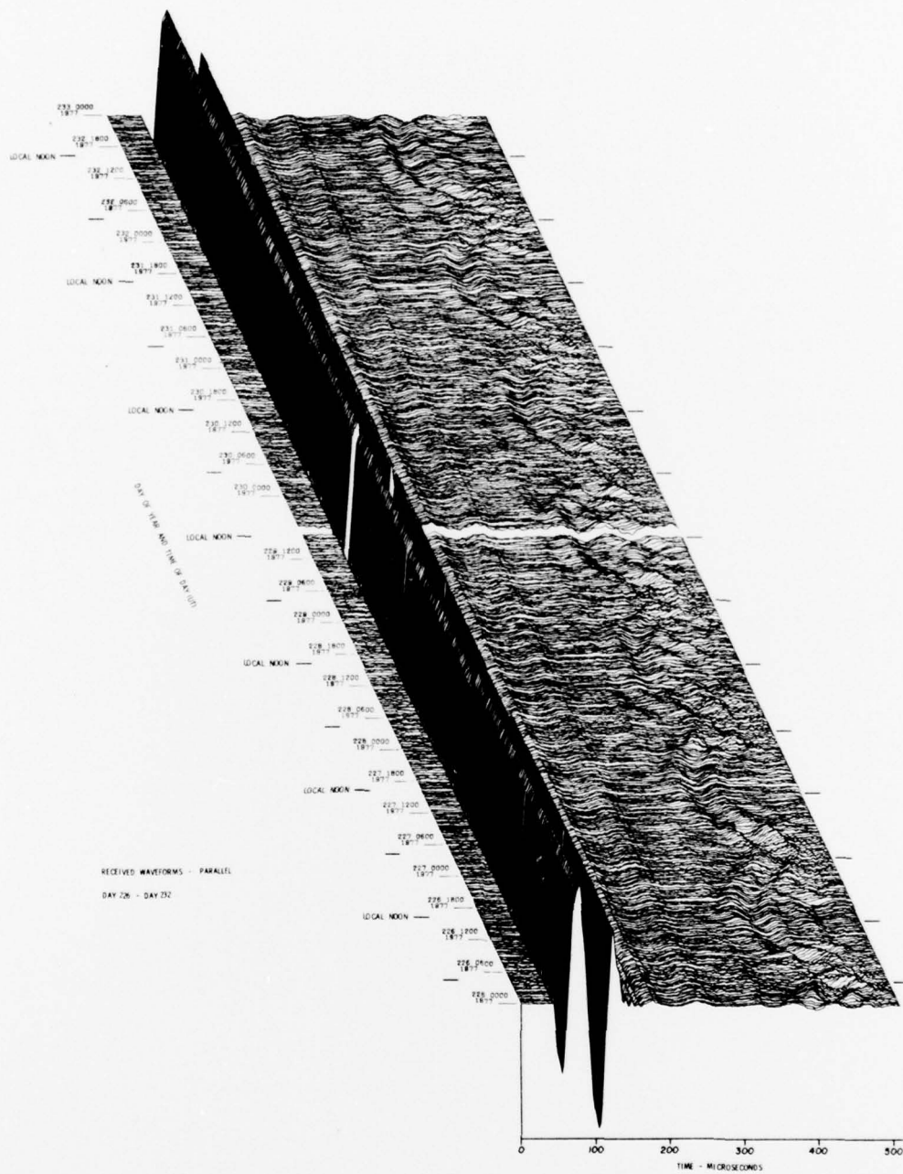
Figure 18. VLF/LF Reflectivity Data for the Polar Ionosphere, DAY 226 (14 Aug) - DAY 232 (20 Aug) 1977 (Cont) Part R. || Waveform Display
