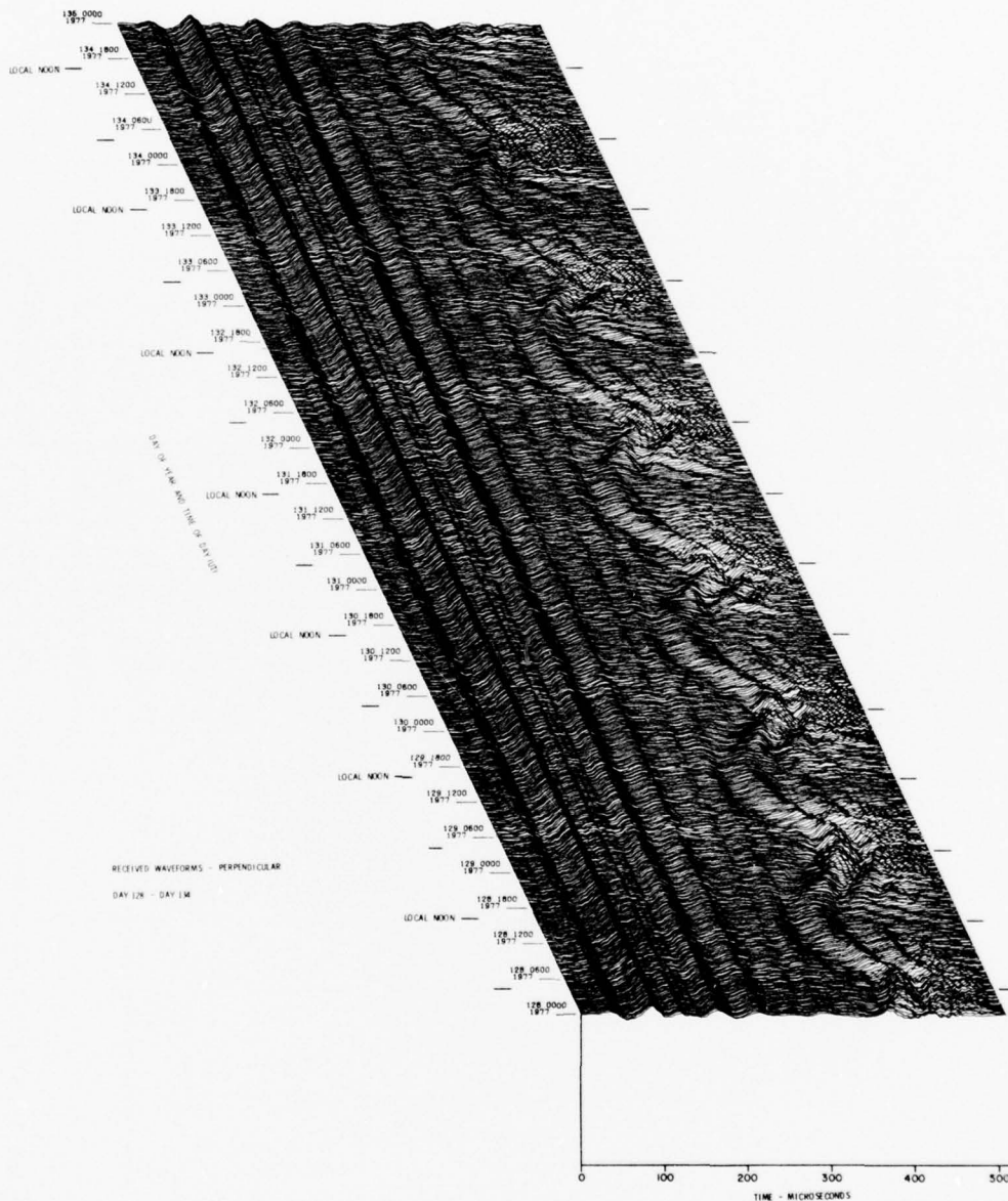
Figure 4. VLF/LF Reflectivity Data for the Polar Ionosphere, DAY 128 (8 May) - DAY 134 (14 May) 1977 (Cont) Part S. \perp Waveform Display
