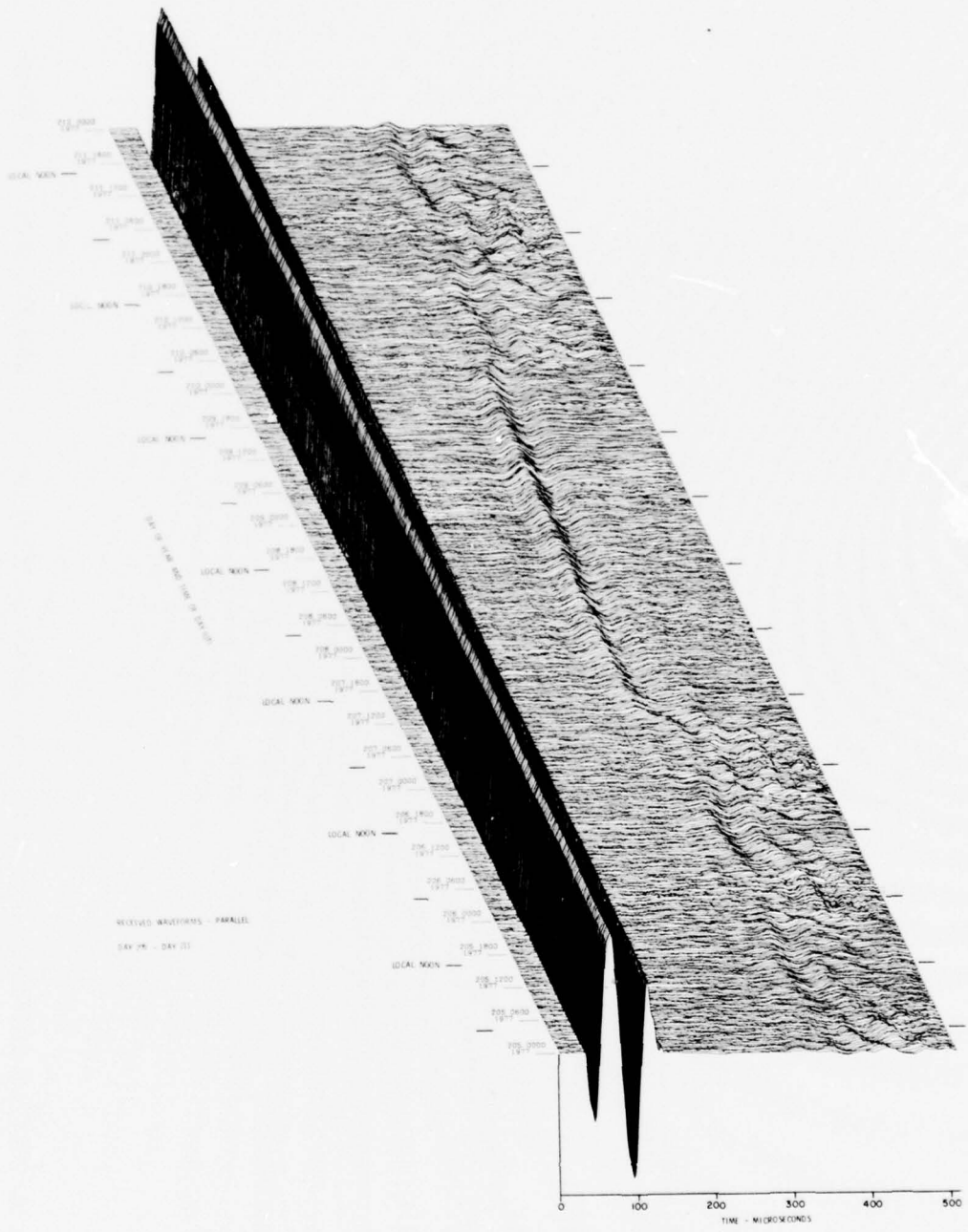
Figure 15. VLF/LF Reflectivity Data for the Polar Ionosphere, DAY 205 (24 Jul) - DAY 211 (30 Jul) 1977 (Cont) Part R. || Waveform Display
