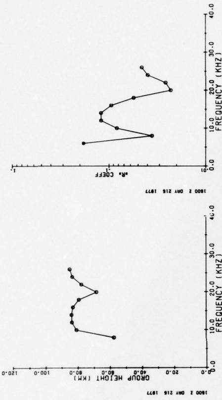
C. GROUP MIRROR REFLECTION HEIGHTS AND ASSOCIATED R_A REFLECTION COEFFICIENTS FROM PARALLEL SKYWAVE DATA
