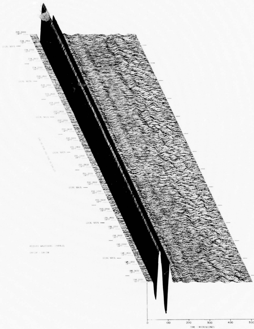
Figure 14. VLF/LF Reflectivity Data for the Polar Ionosphere, DAY 198 (17 Jul) - DAY 204 (23 Jul) 1977 (Cont) Part R. II Waveform Display
