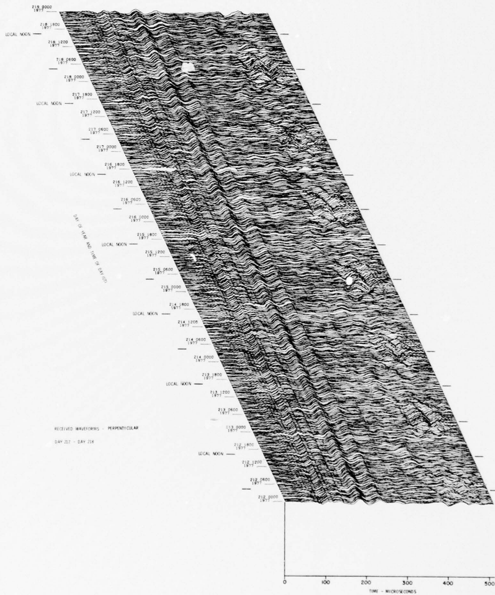
Figure 16. VLF/LF Reflectivity Data for the Polar Ionosphere, DAY 212 (31 Jul) - DAY 218 (6 Aug) 1977 (Cont) Part S. \perp Waveform Display
