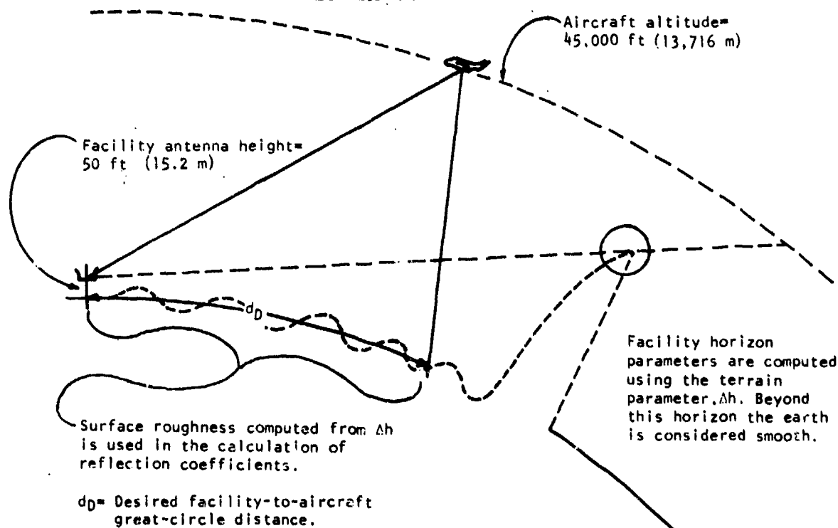
Figure A9. Problem A2, geometry sketch (not drawn to scale).
