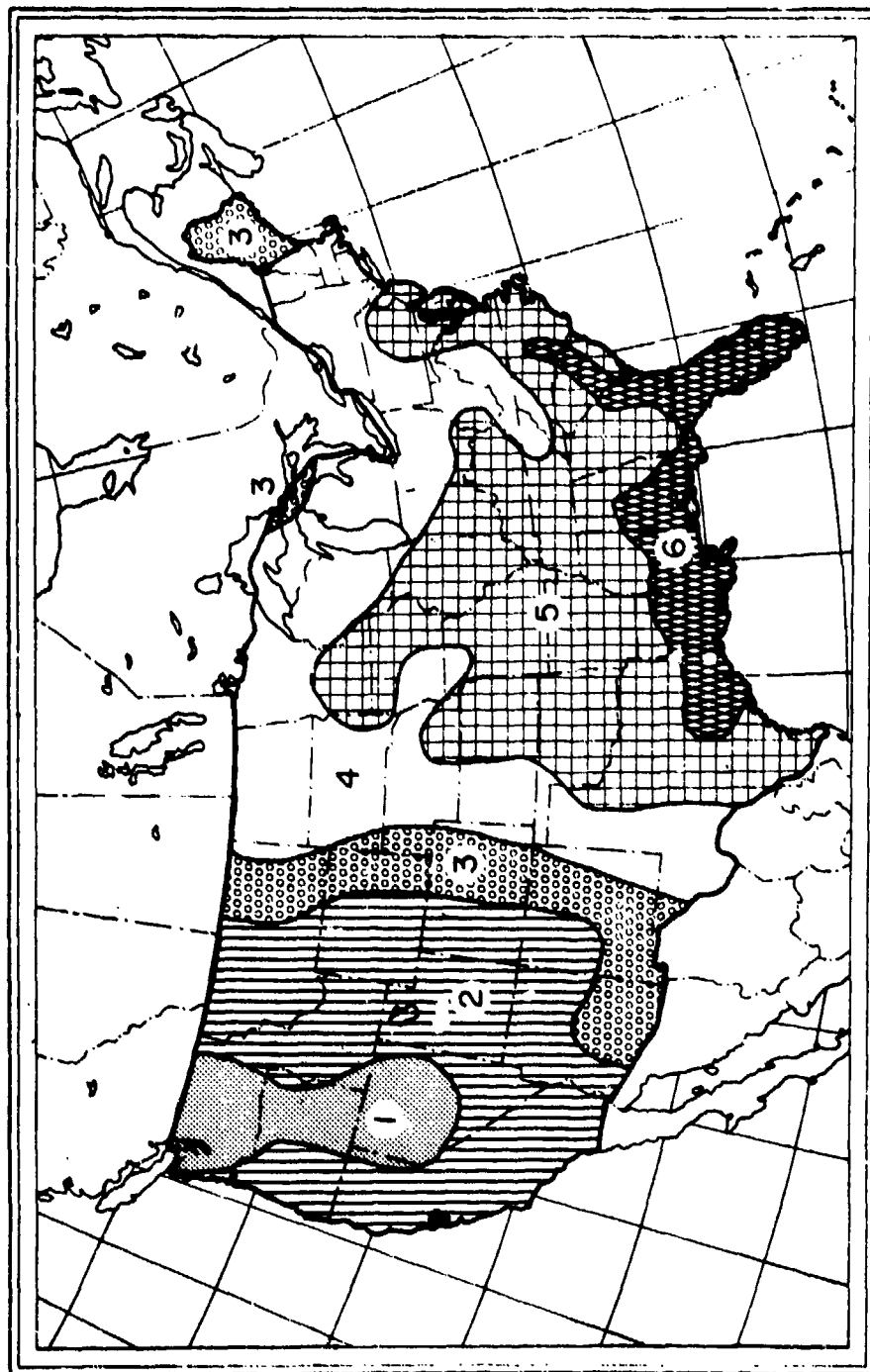
Figure 49. Rain zones of the continental United States [54, fig. 10]. Areas where the 5-min rainfall rate in inches/hour is expected to occur once in 2 years on the average are shown; e.g., area 5 ranges from 4 1/2 to 5 1/2 in/hr (110 to 140 mm/hr). Rain rates of 1, 2, 3, 4, 5, and 6 in/hr are equivalent to rates of 25, 51, 76, 100, 130 and 150 mm/hr, respectively.
