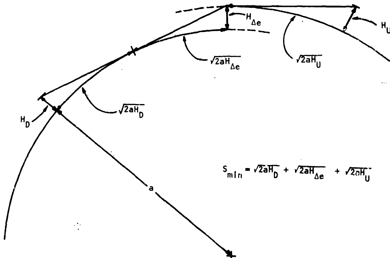
Figure A28. Geometry for S_{min} (not drawn to scale.)
