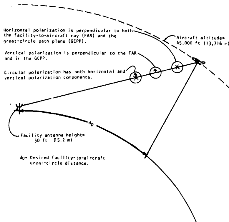
Figure A1. Problem A1, geometry sketch (not drawn to scale).
