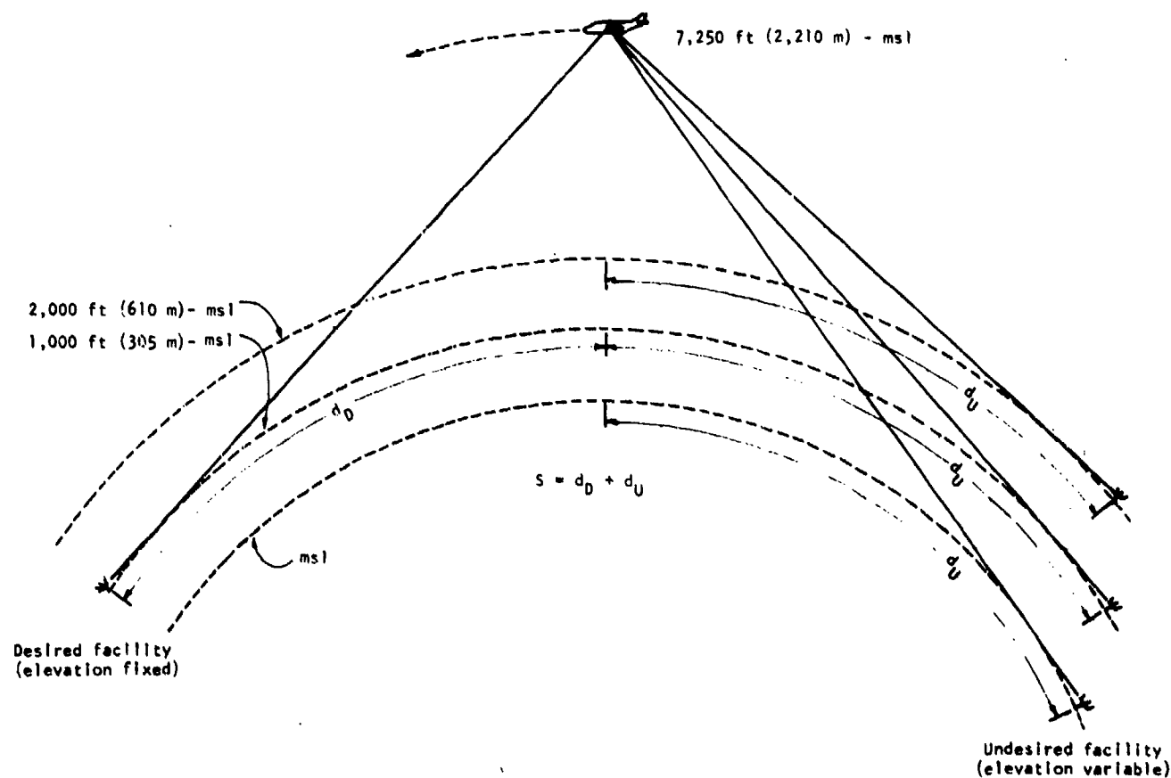
Figure A26. Problem A6, geometry sketch (not drawn to scale).
