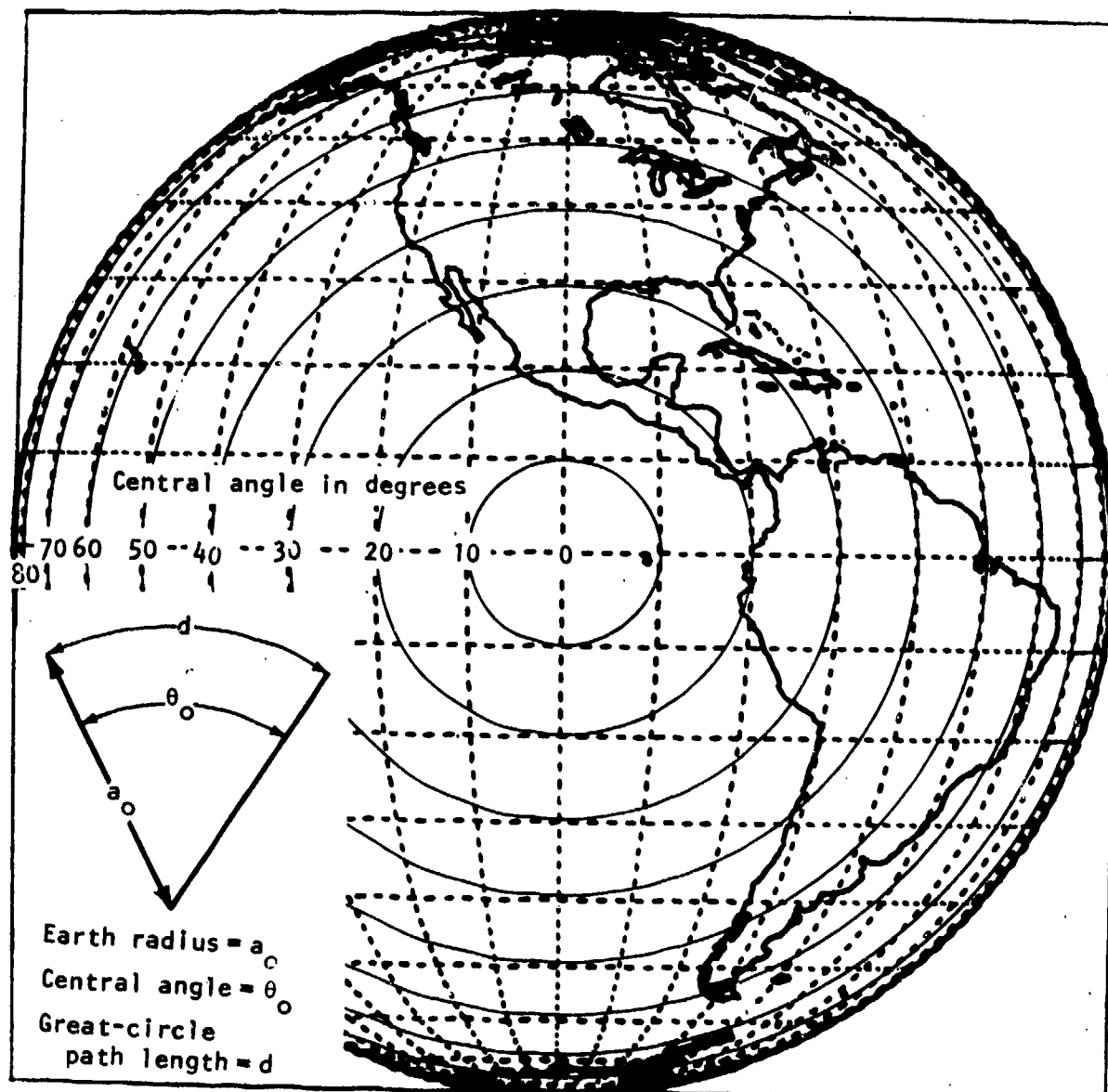
Figure 41. Geographic location of constant central angle contours The subsatellite point is at 100^{\circ}\text{W} [23, figs. 8, 9].
