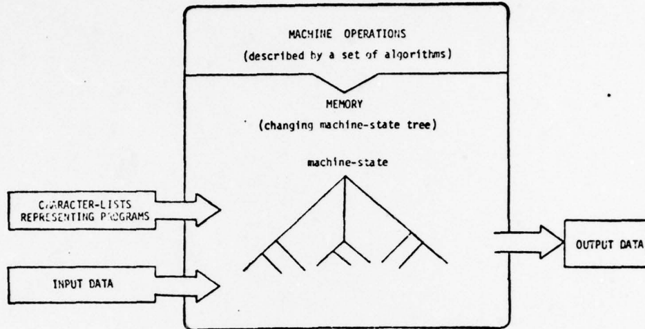
Figure 1. The Abstract Machine
