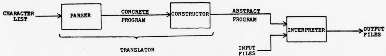
Figure 2. The Definition Process
