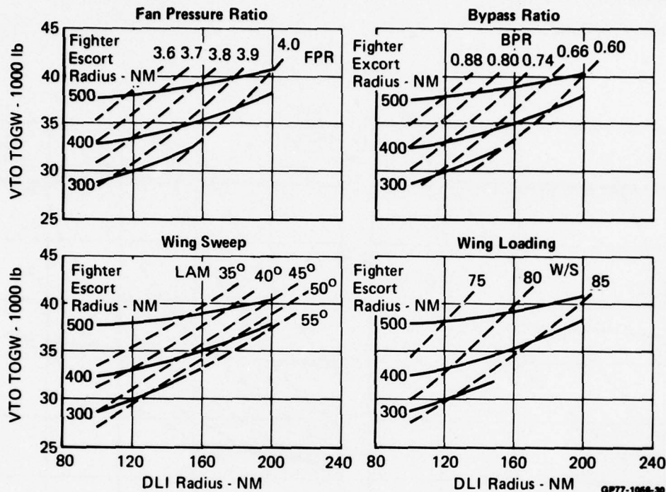
FIGURE 18 MULTI-MISSION INTERACTIONS Fixed Cycle Engine Turbofan
