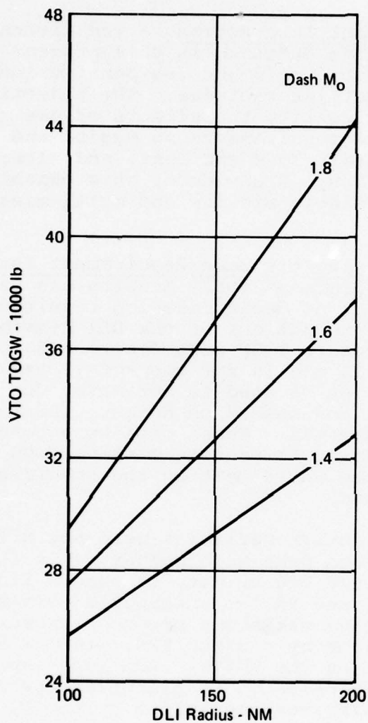
FIGURE 14 ENGINE/AIRFRAME/REQUIREMENT INTERACTIONS - DLI MISSION Fixed Cycle Engine Turbofan (FCE-TF)
