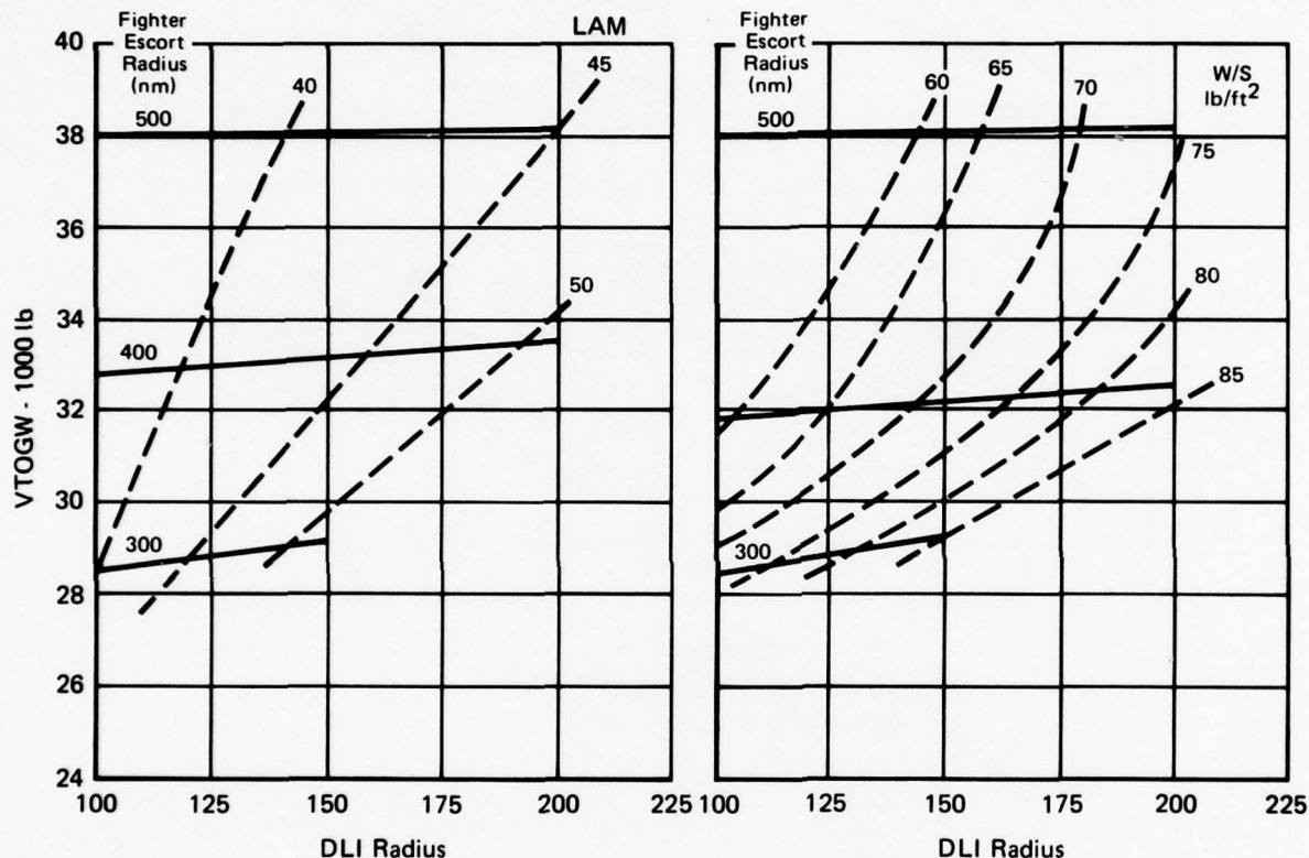
FIGURE 19 MULTI-MISSION INTERACTIONS Variable Geometry Turbine Turbojet
